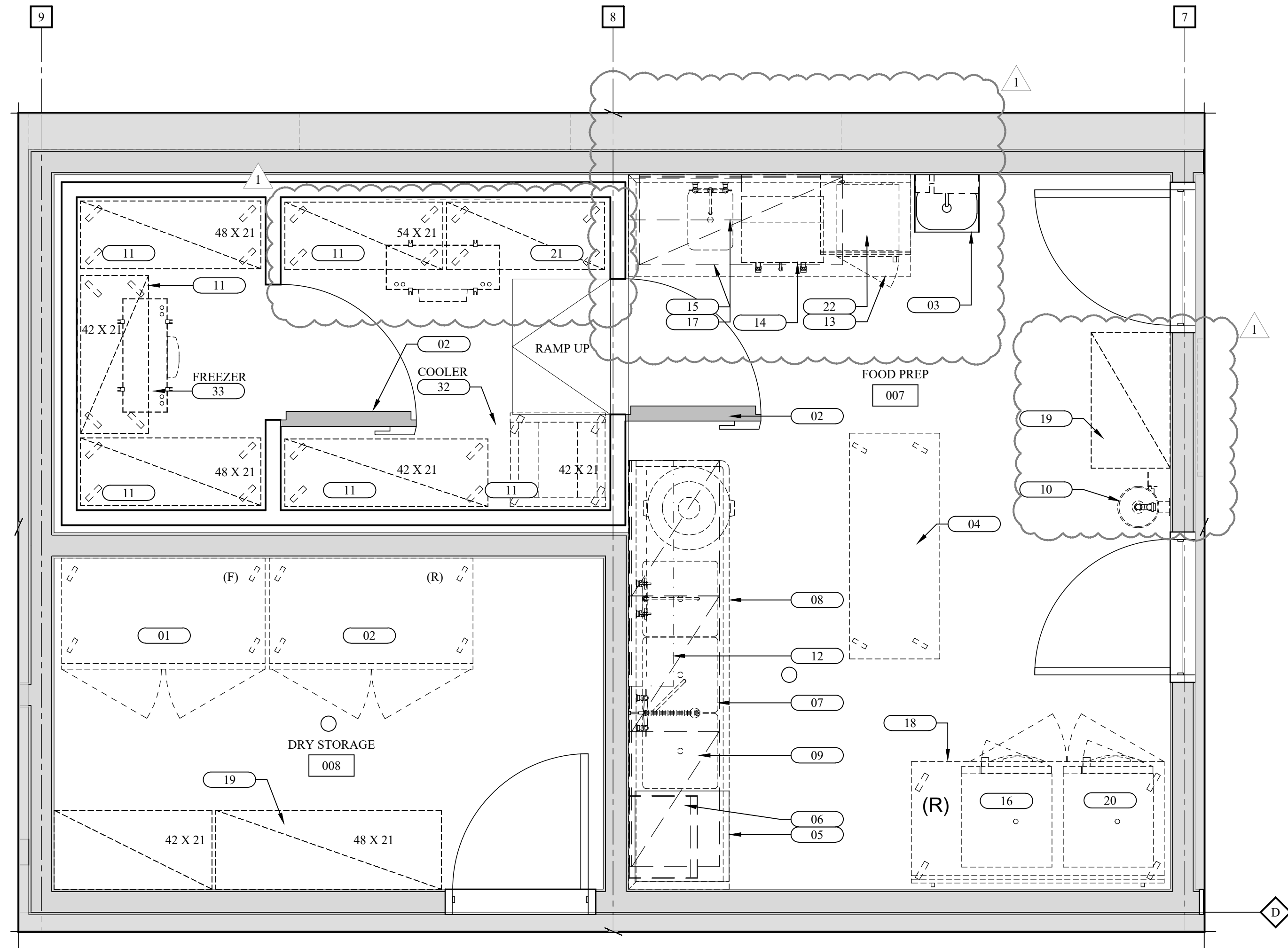
1 FOOD PREP & DRY STORAGE PLAN 1/2" = 1'-0"
