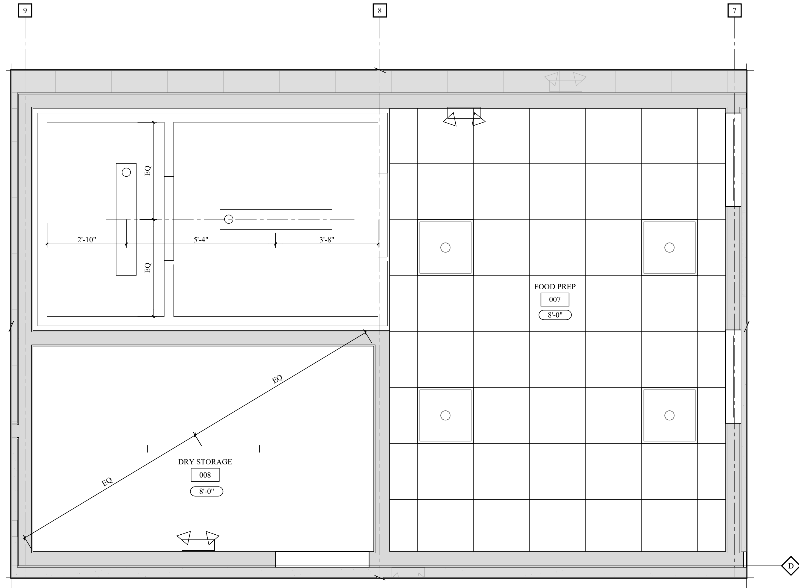
2 FOOD PREP & DRY STORAGE RCP PLAN 1/2" = 1'-0"
