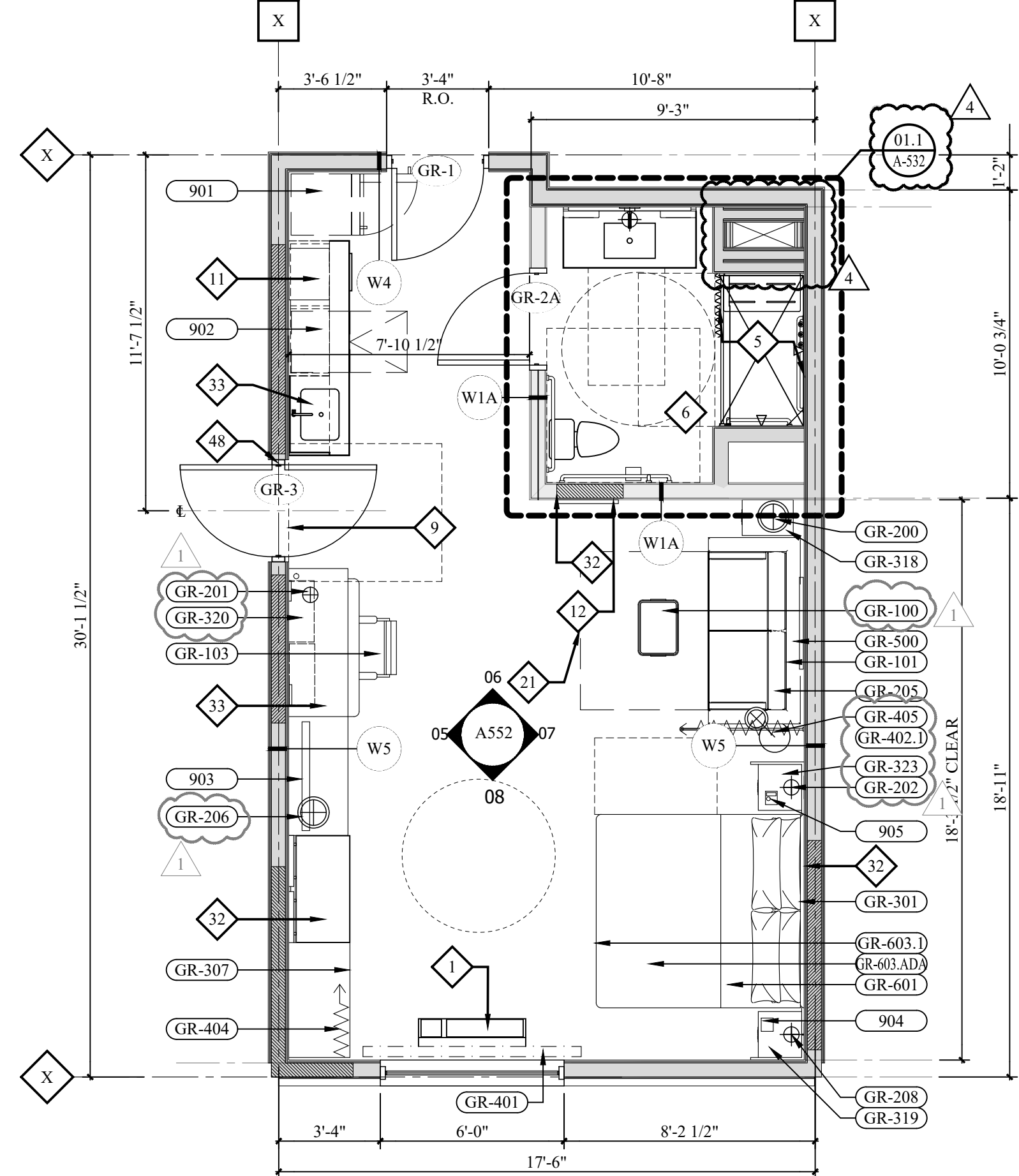
01 KING STUDIO ACC MOD-ARCHITECTURAL PLAN 1/4" = 1'-0"
