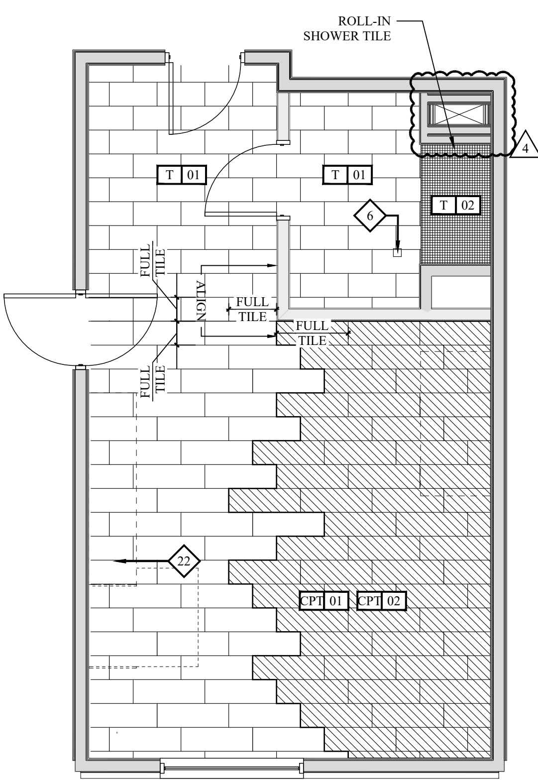
03 KING STUDIO ACC MOD-FINISH PLAN 1/4" = 1'-0"
