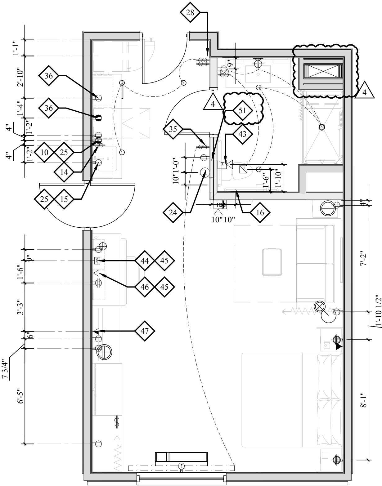
04 KING STUDIO ACC MOD-ELECTRICAL PLAN 1/4" = 1'-0"
