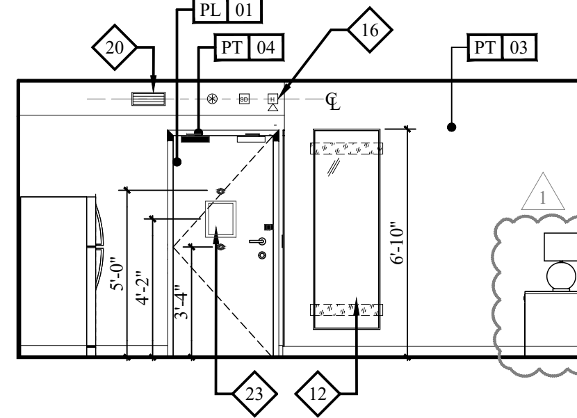
06 INTERIOR ELEVATION 1/4" = 1'-0"
