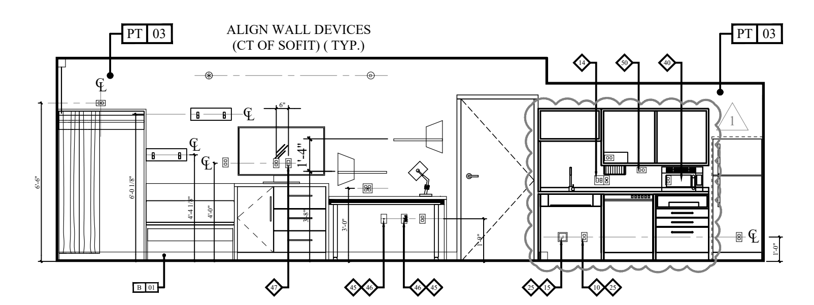
05 INTERIOR ELEVATION 1/4" = 1'-0"
