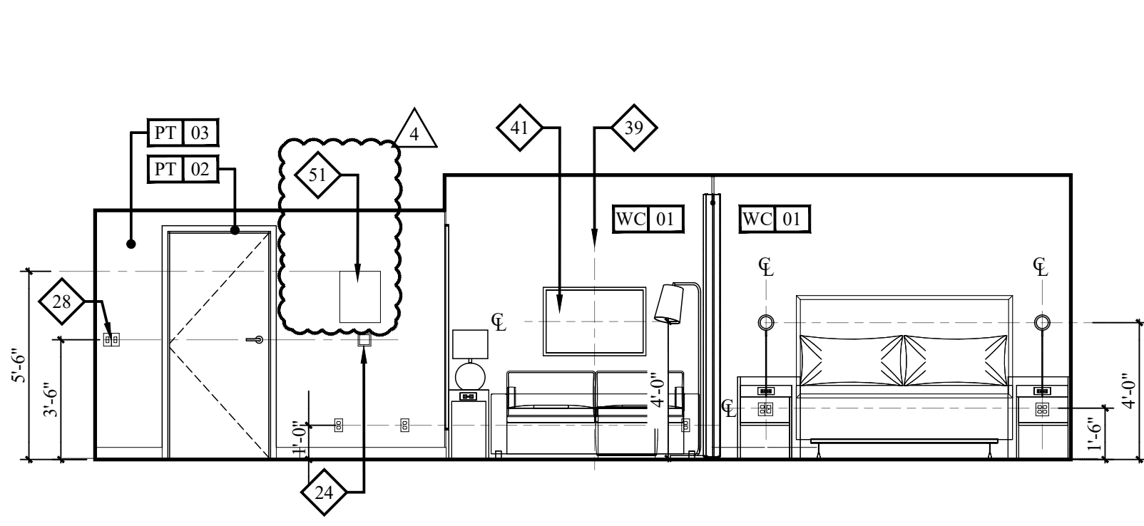
07 INTERIOR ELEVATION 1/4" = 1'-0"
