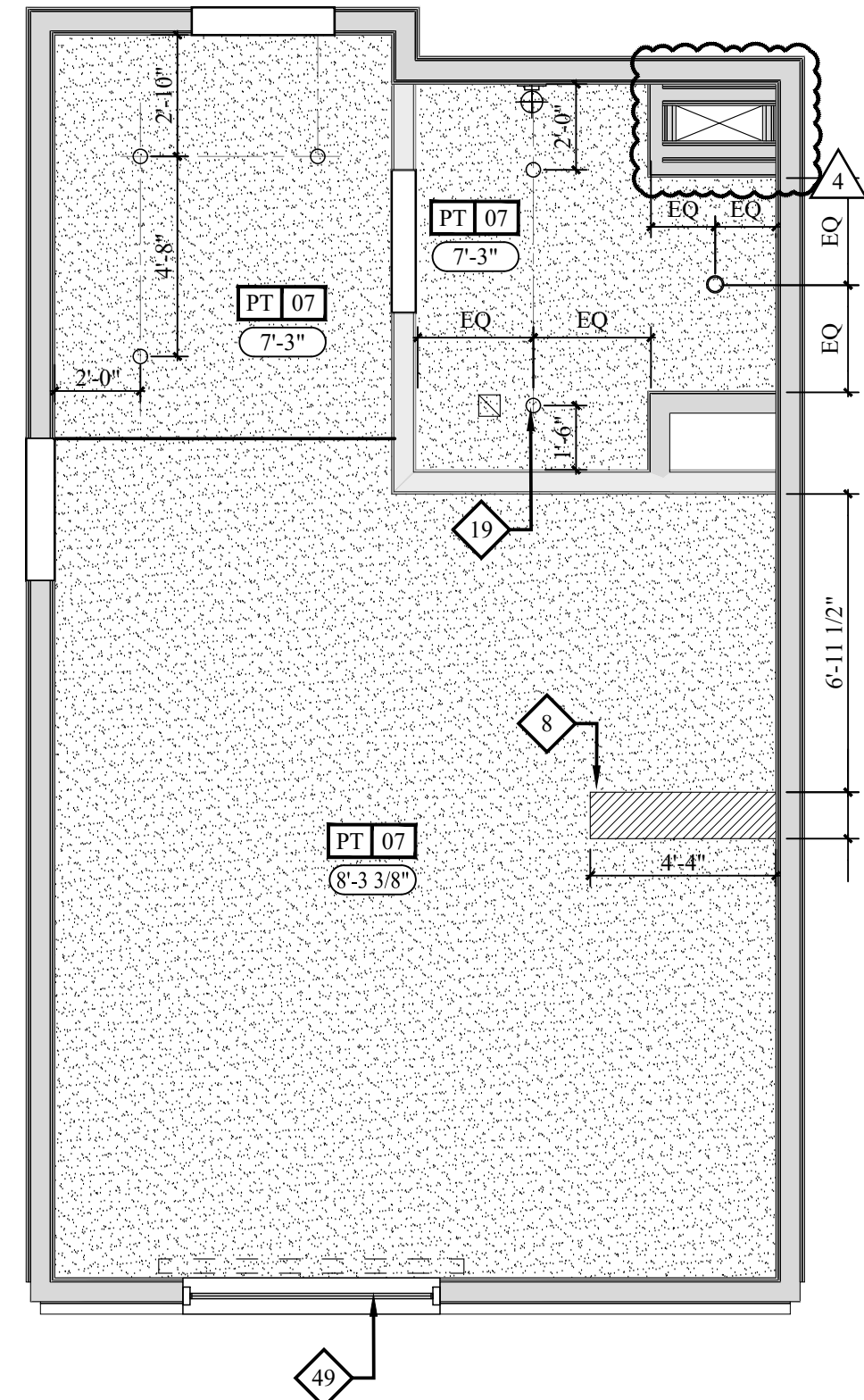
02 KING STUDIO ACC MOD-REFLECTED CEILING PLAN 1/4" = 1'-0"
