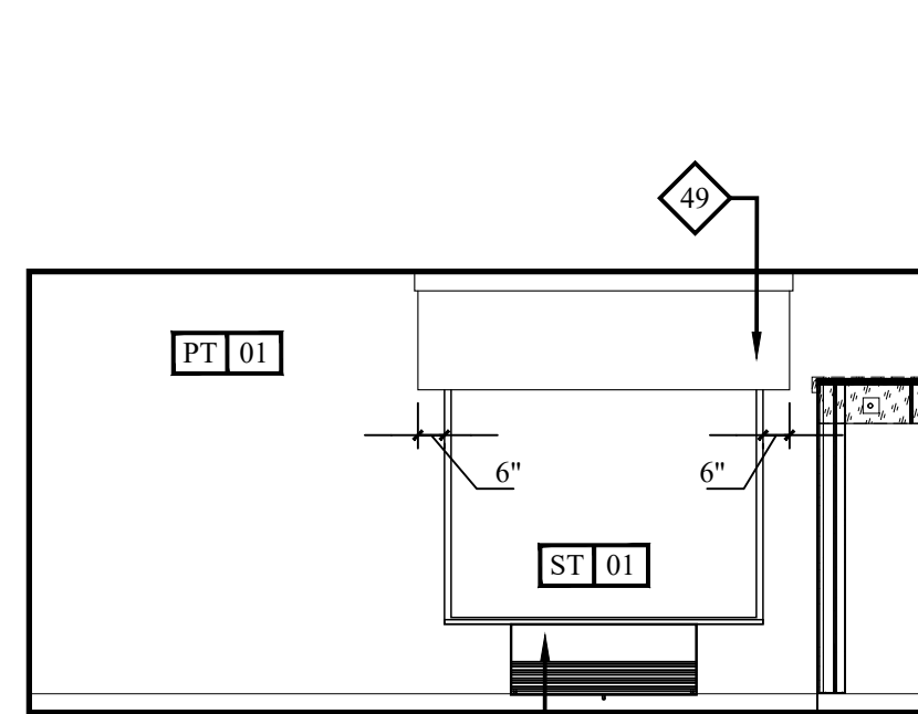
08 INTERIOR ELEVATION 1/4" = 1'-0"
