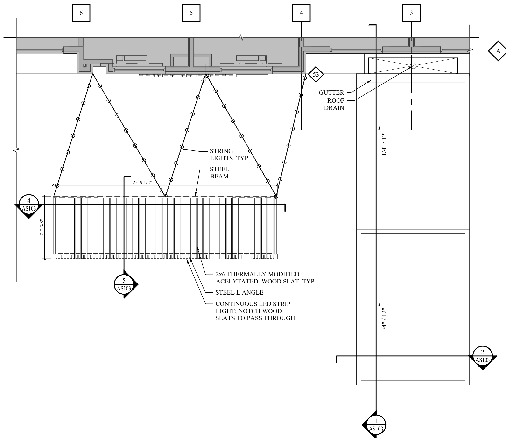
4 ENLARGED PLAN - CANOPY AND TRELLIS 3/16" = 1'-0"
