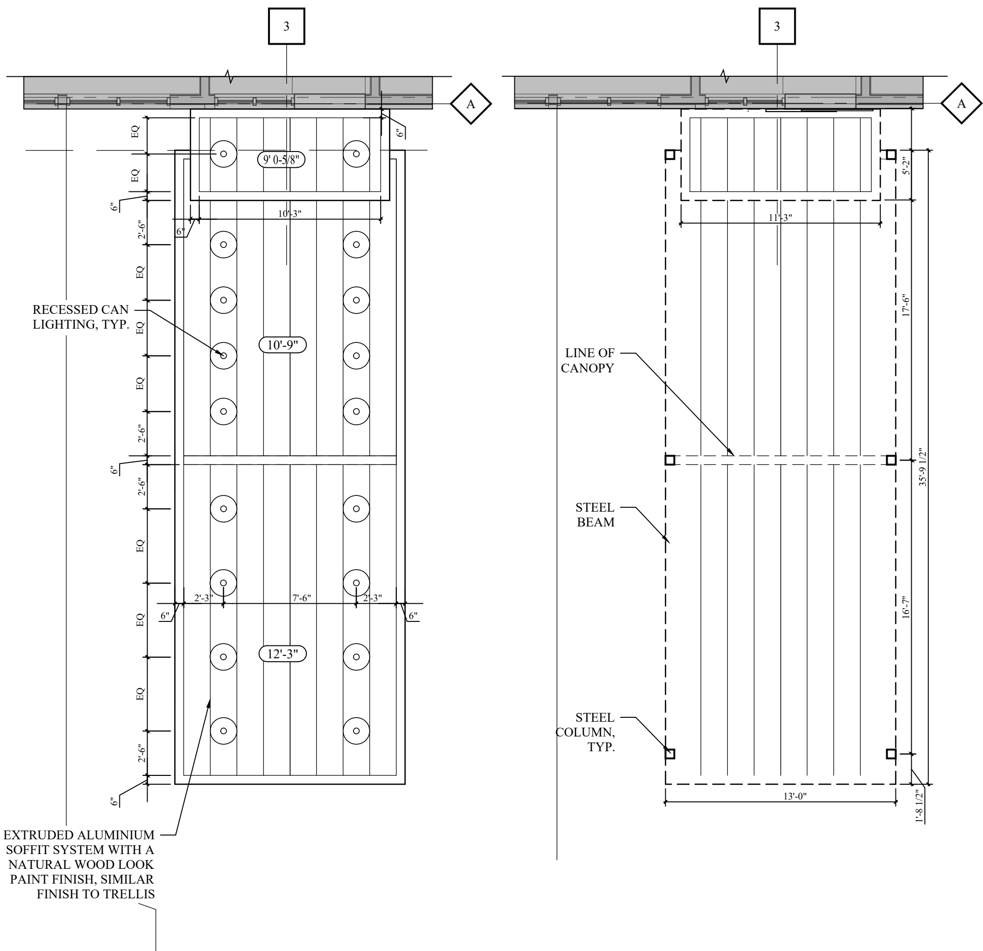
3 CANOPY - RCP PLAN 3/16" = 1'-0"
