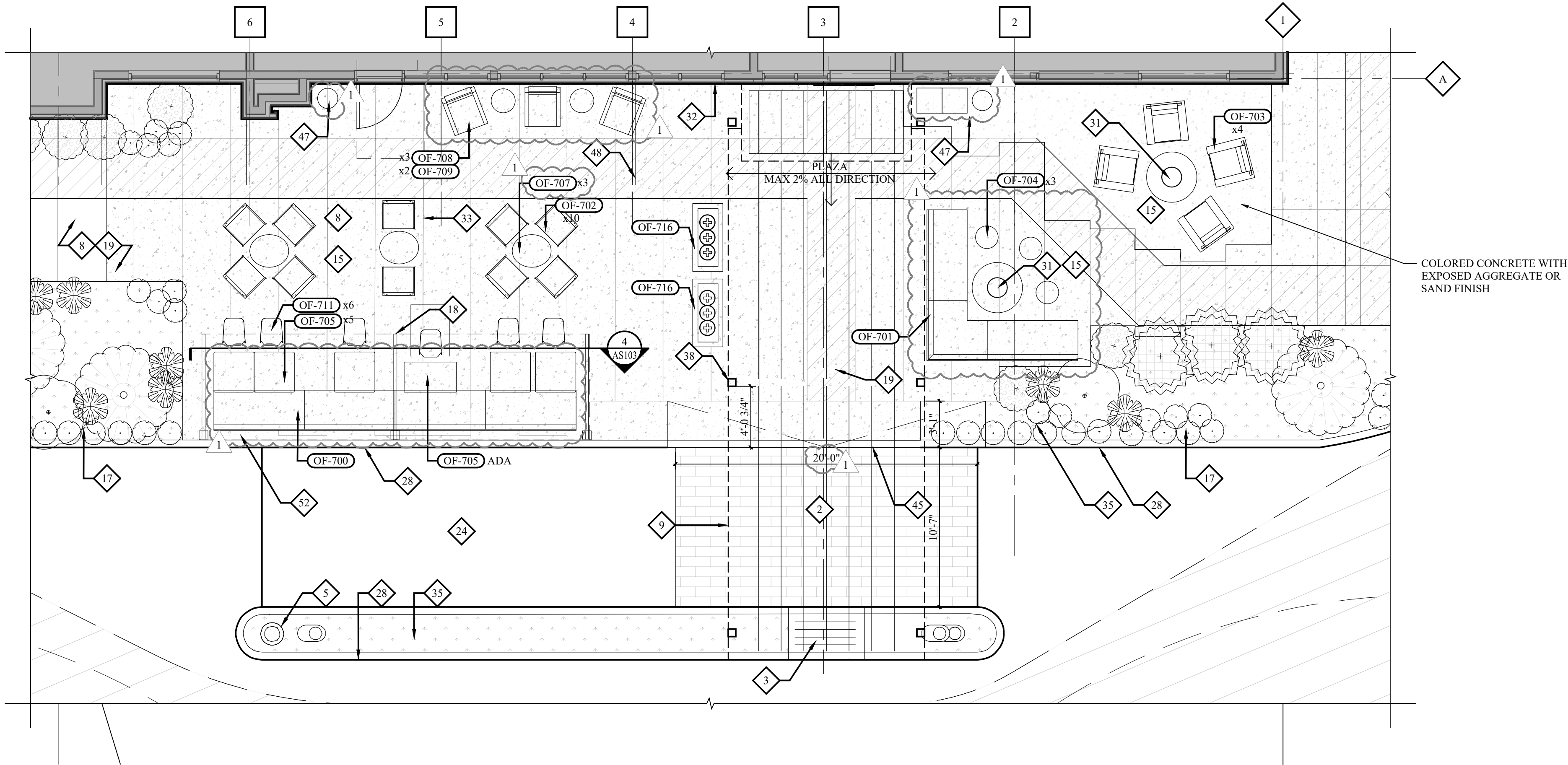
1 ENTRANCE/DROP OFF CANOPY & OUTDOOR LOUNGE PLAN 3/16" = 1'-0"
