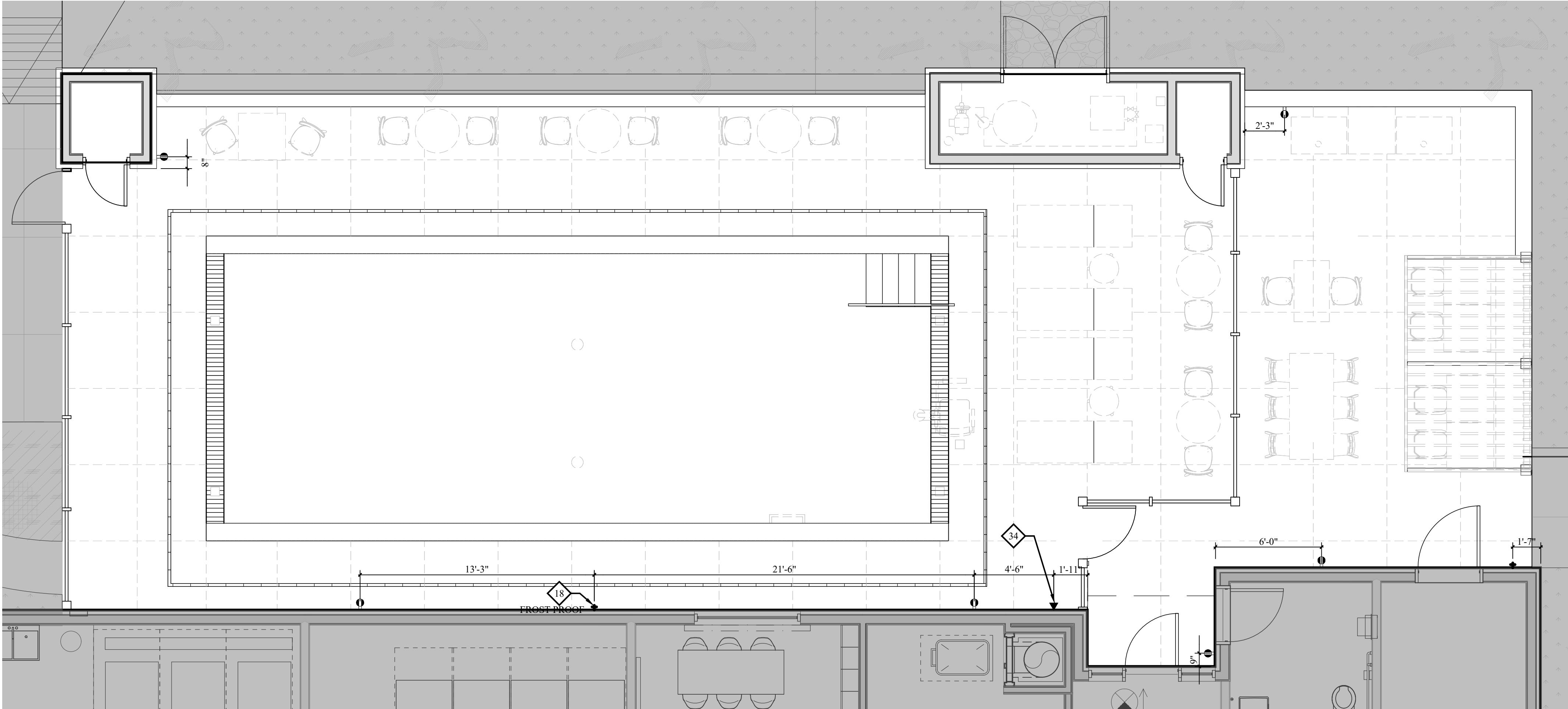
1 ENL. OUTDOOR POOL - POWER PLAN 1/4" = 1'-0"
