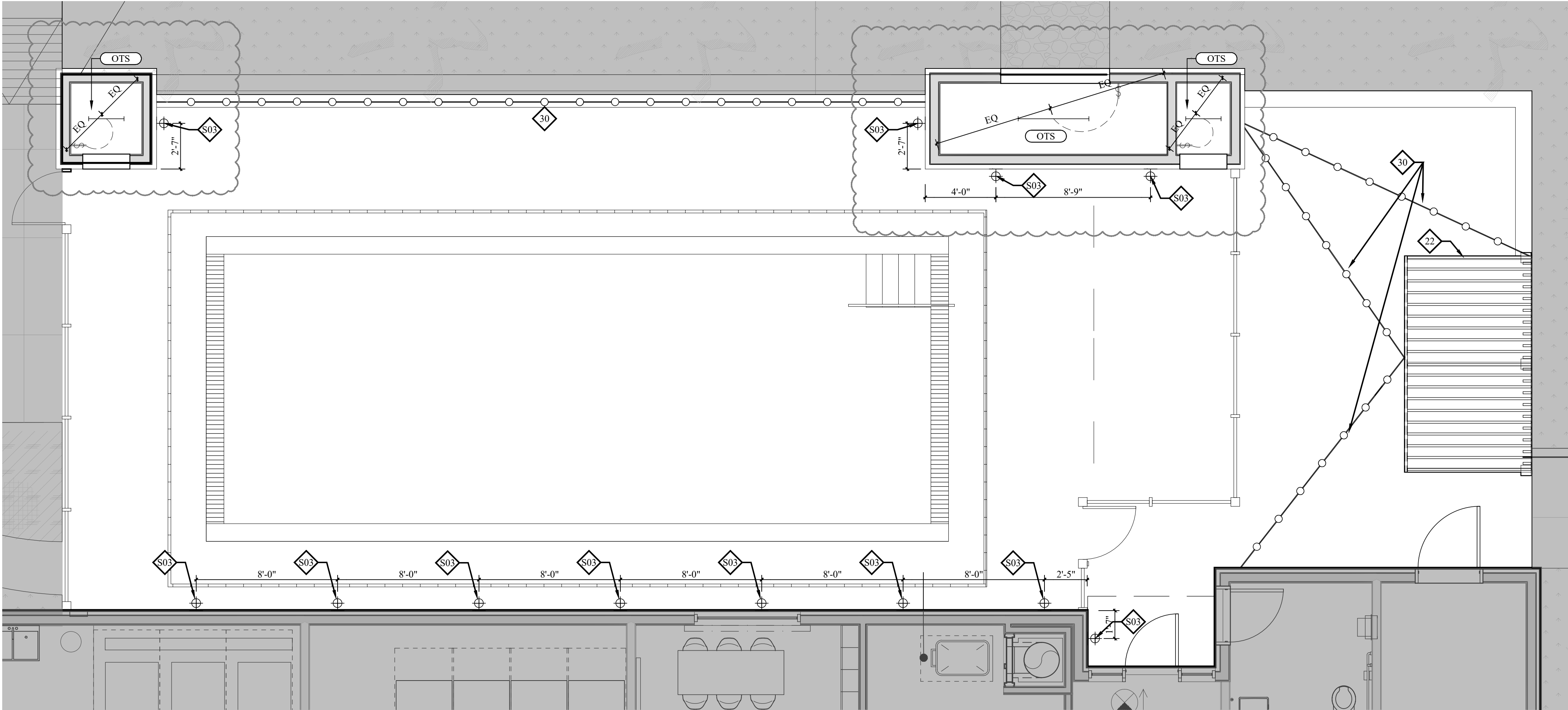
2 ENL. OUTDOOR POOL - REFLECTIVE CEILING PLAN 1/4" = 1'-0"
