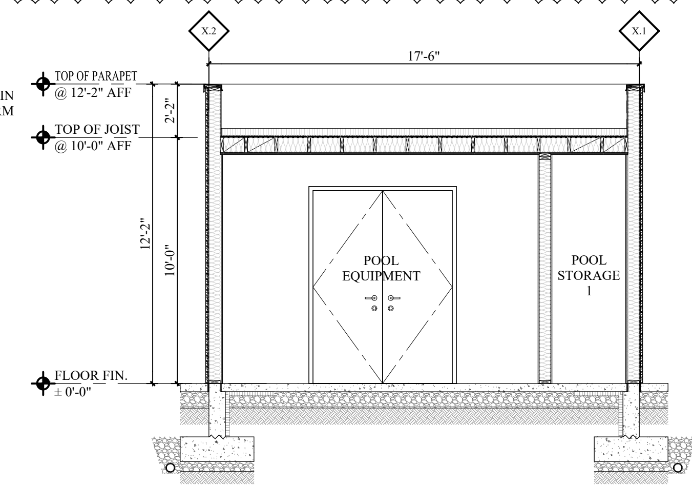
5 POOL EQUIP. - SECTION
