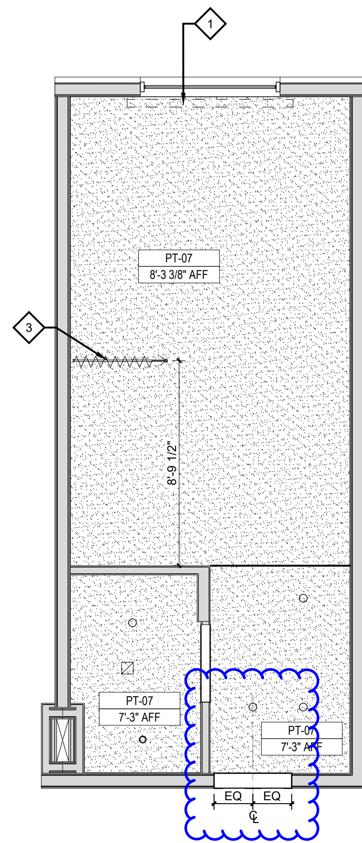
2 KING STUDIO- REFLECTED CEILING PLAN 1/4" = 1'-0"
