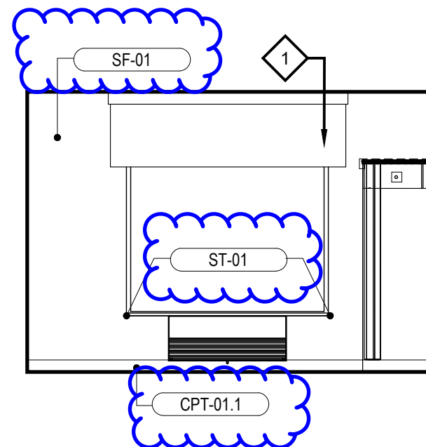
8 INTERIOR ELEVATION 1/4" = 1'-0"
