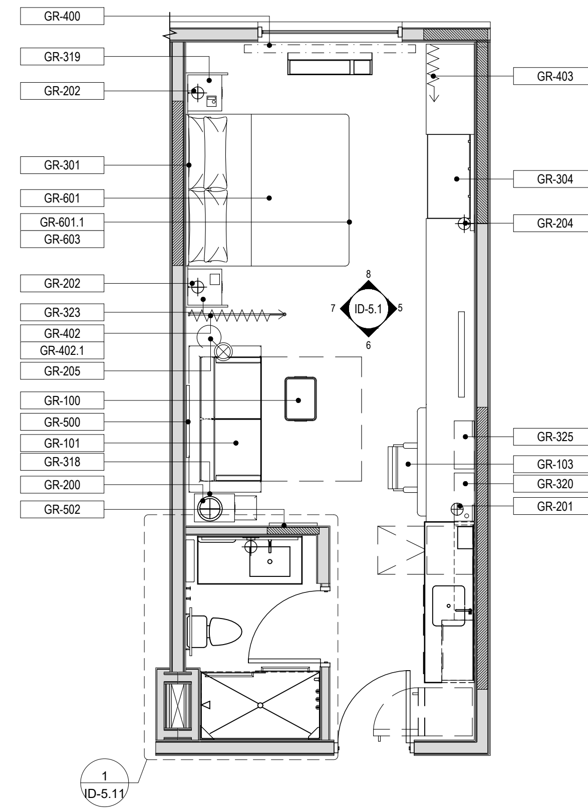
1 KING STUDIO - FFE PLAN 1/4" = 1'-0"
