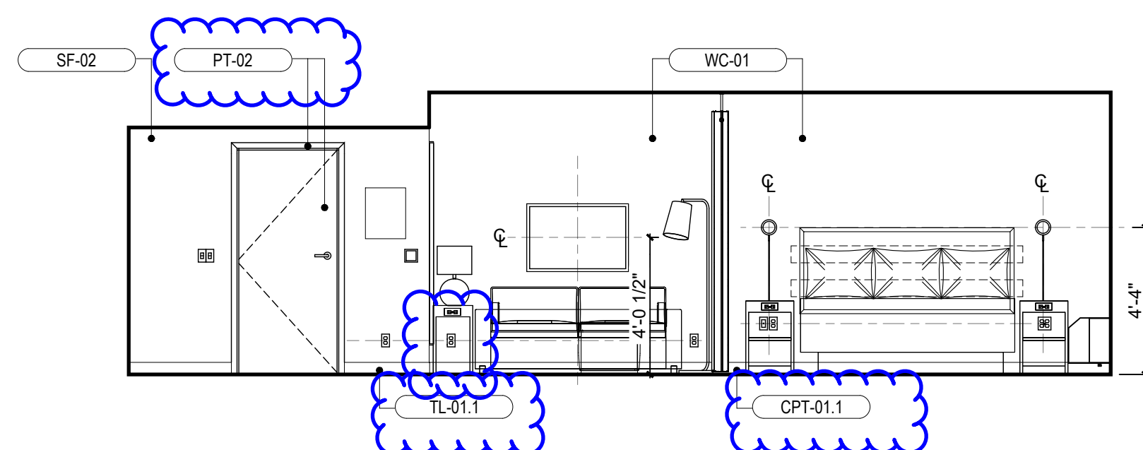
7 INTERIOR ELEVATION 1/4" = 1'-0"
