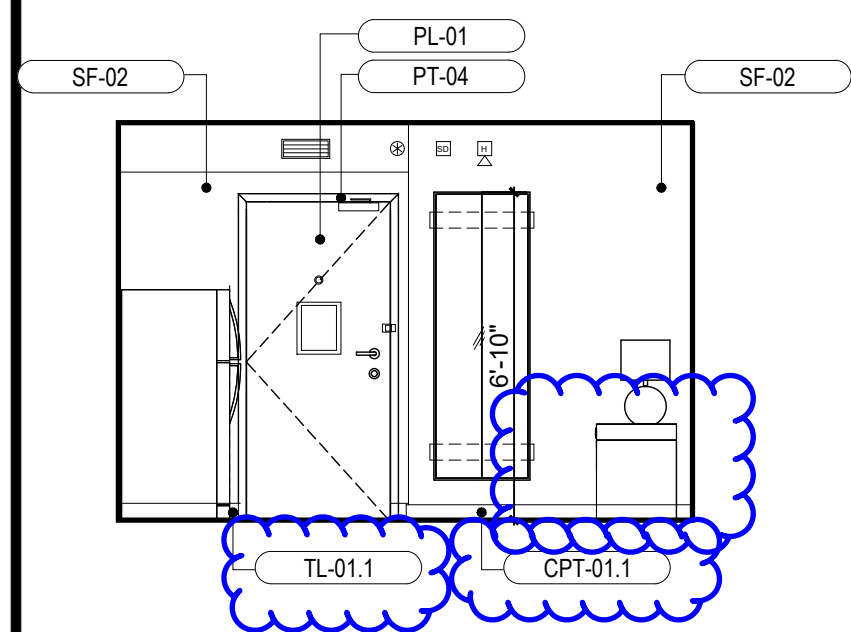
6 INTERIOR ELEVATION 1/4" = 1'-0"
