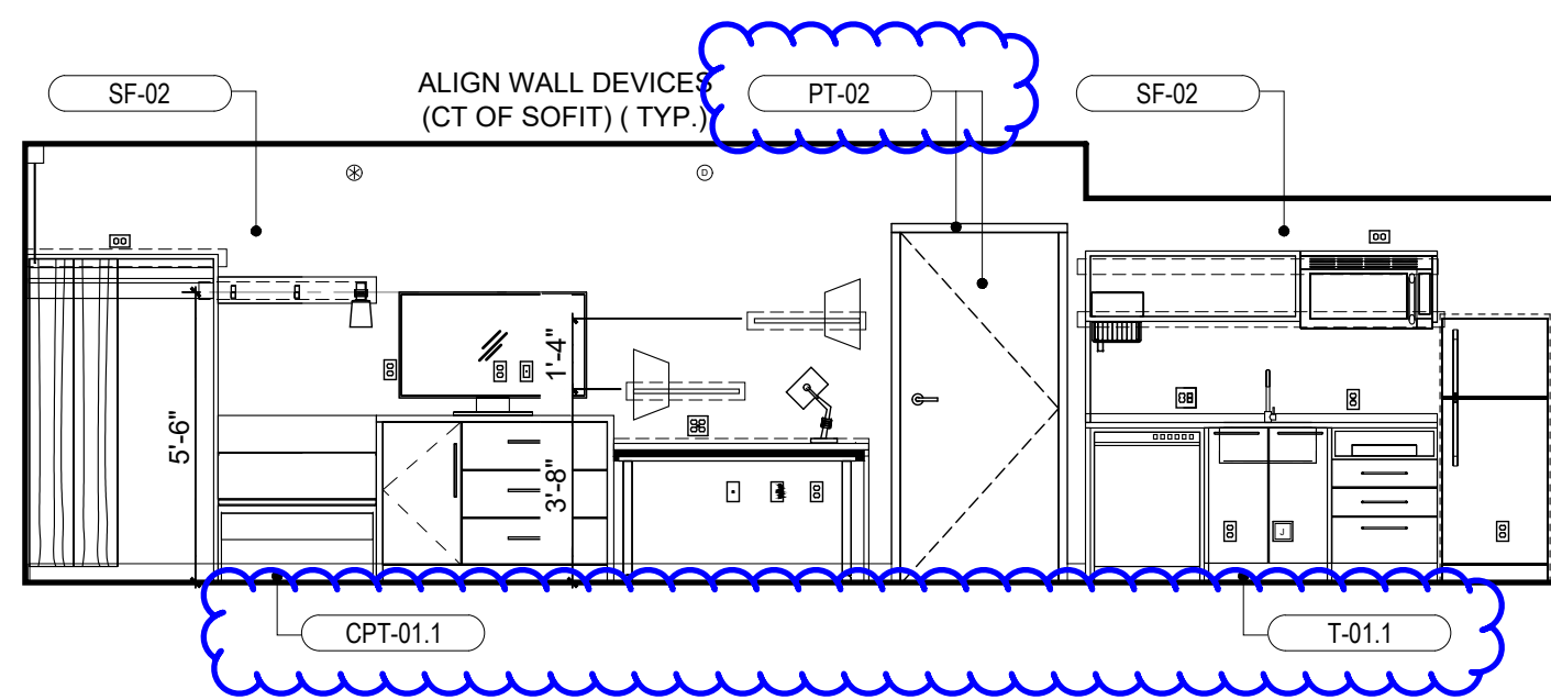
9 INTERIOR ELEVATION 1/4" = 1'-0"
