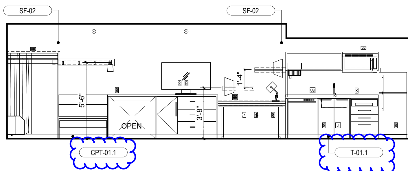
5 INTERIOR ELEVATION 1/4" = 1'-0"
