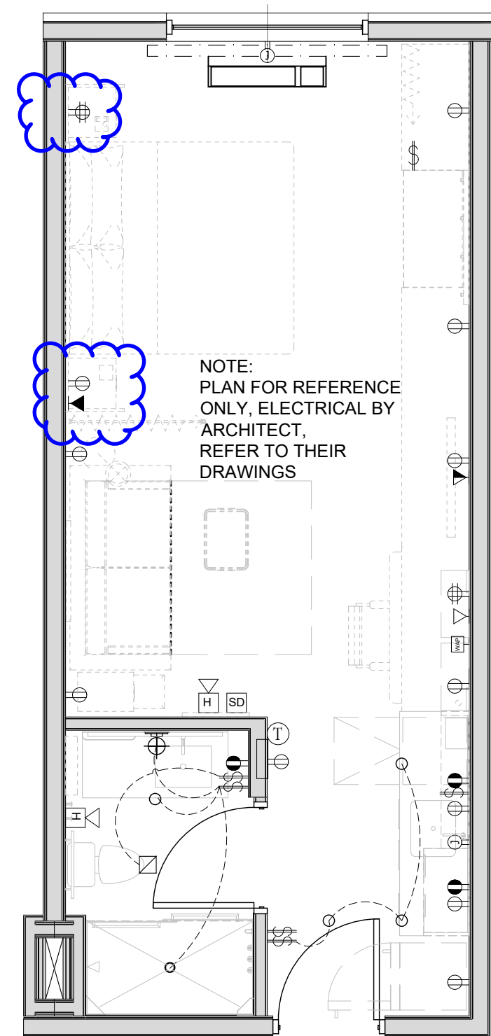
4 KING STUDIO-ELECTRICAL PLAN 1/4" = 1'-0"
