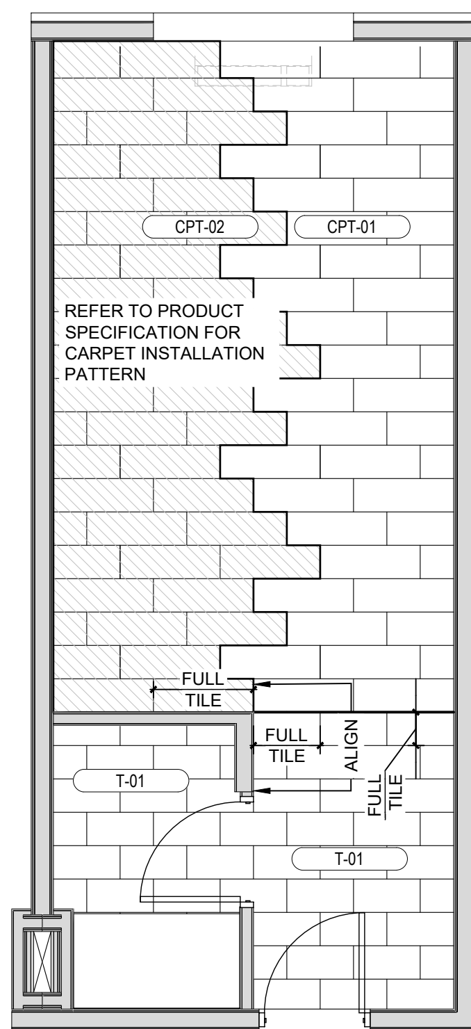
3 KING STUDIO-FINISH PLAN 1/4" = 1'-0"
