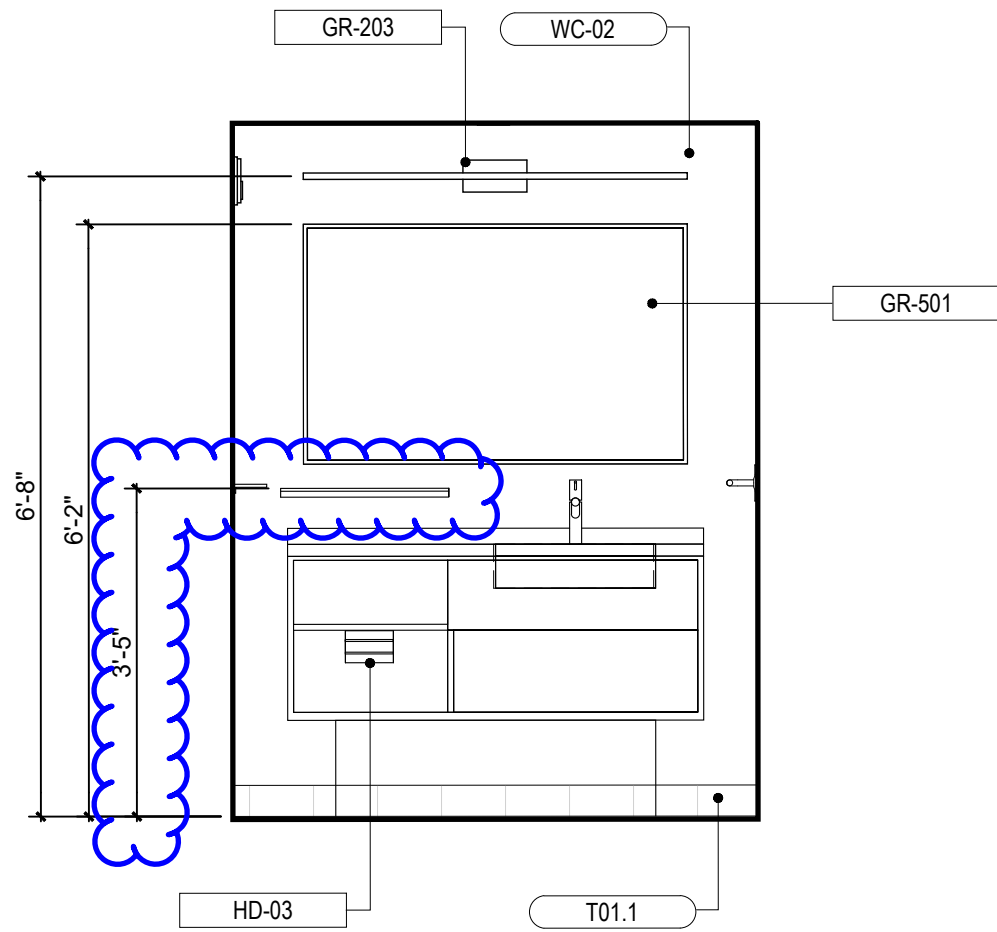
2 INTERIOR ELEVATION 1/2" = 1'-0"
