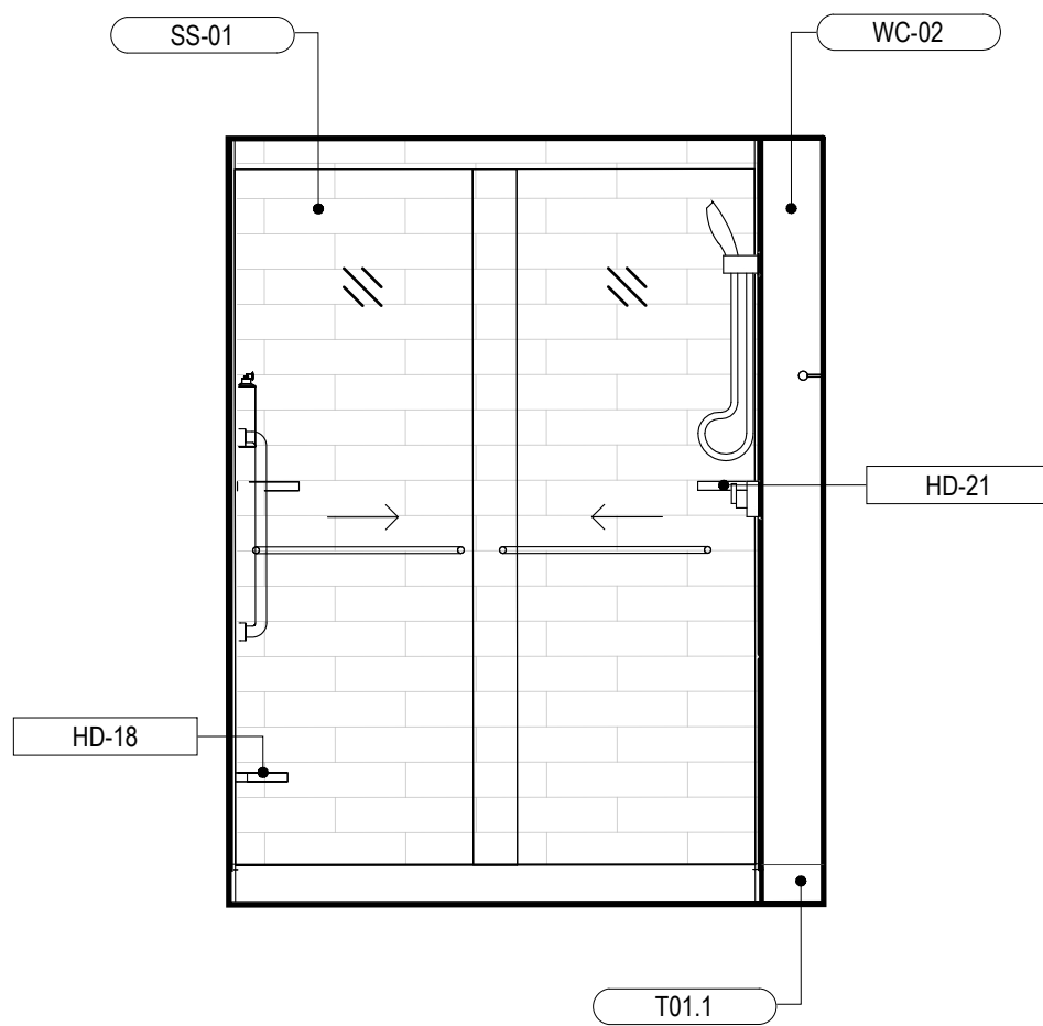
4 INTERIOR ELEVATION 1/2" = 1'-0"
