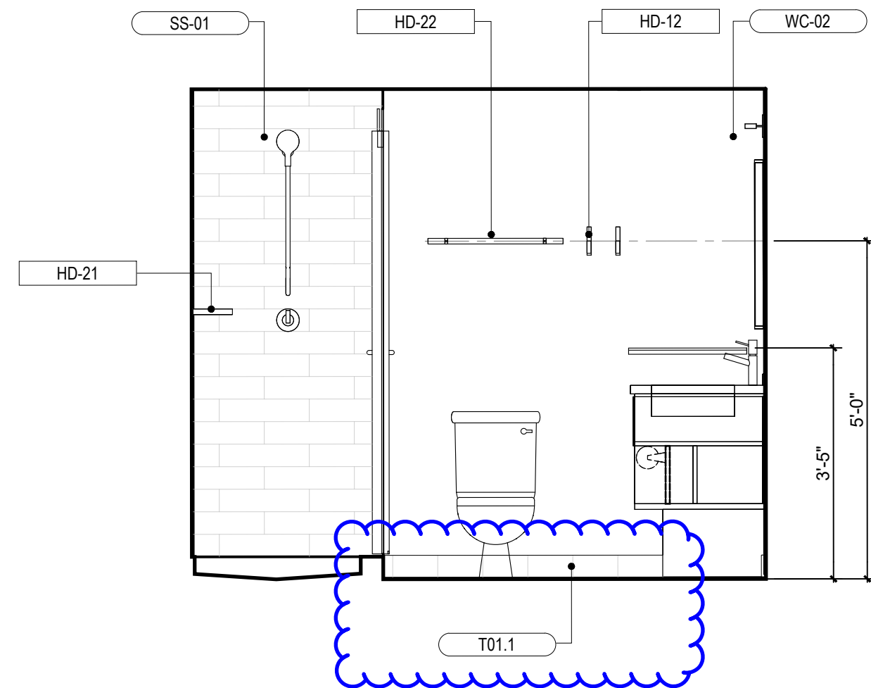
5 INTERIOR ELEVATION 1/2" = 1'-0"
