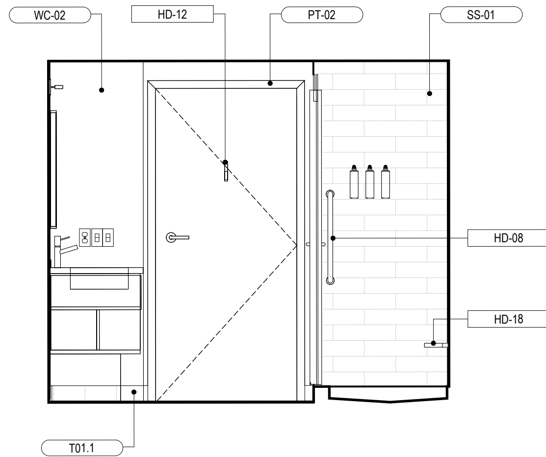
3 INTERIOR ELEVATION 1/2" = 1'-0"
