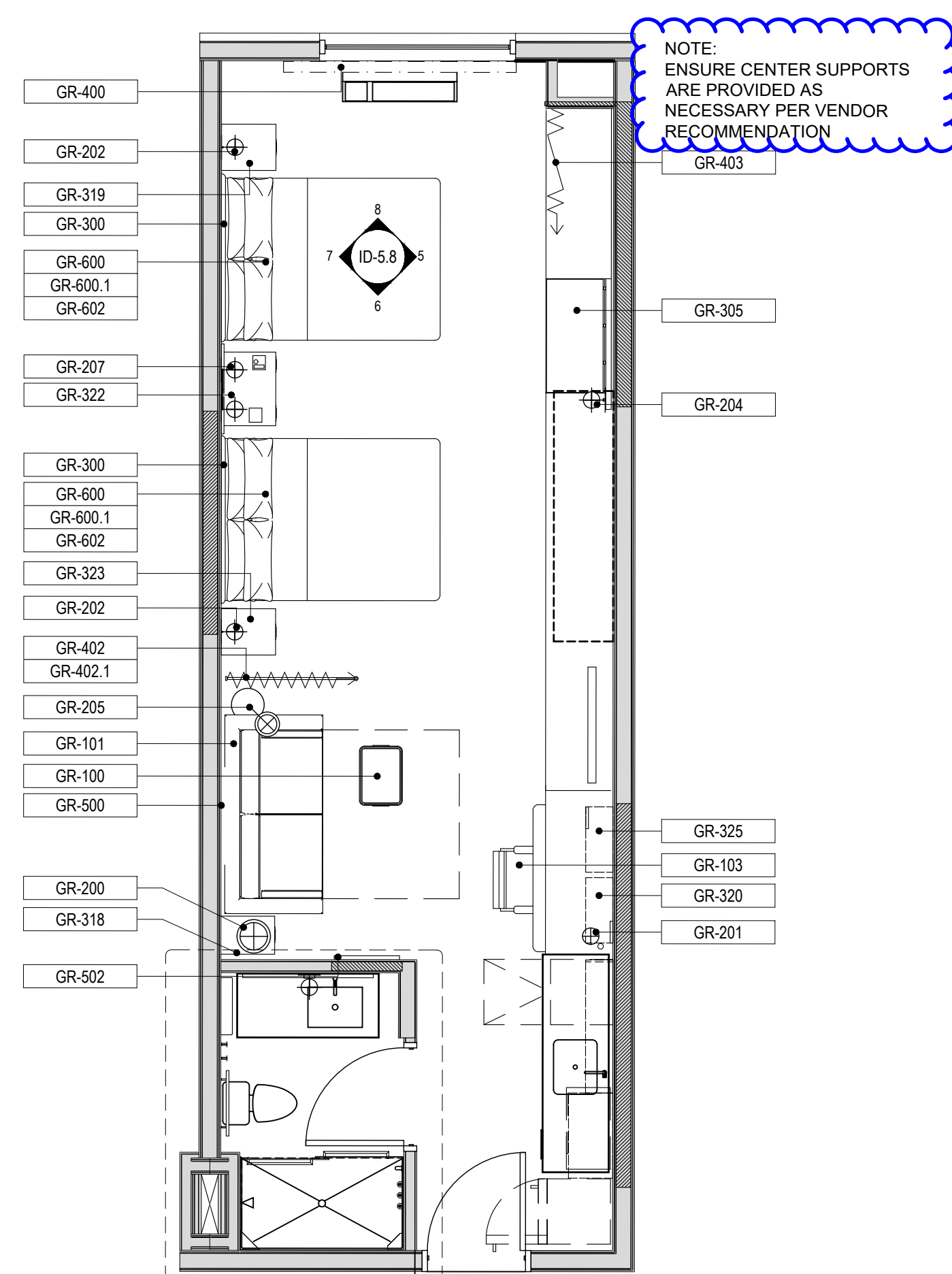
1 FFE PLAN
