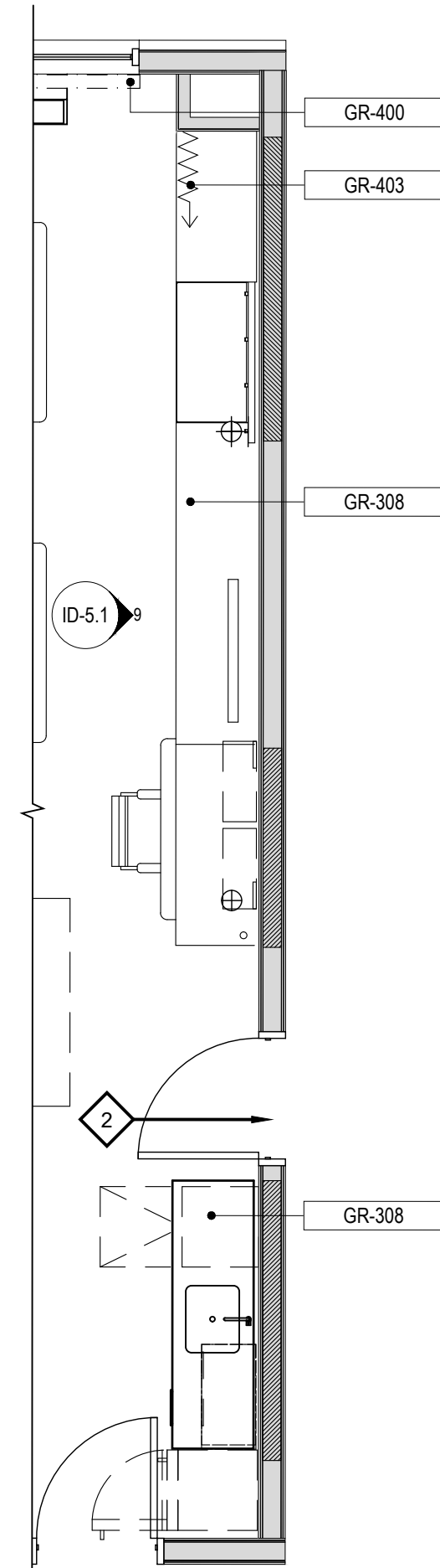
1.1 QQ STUDIO CONN. ARCHITECTURAL PLAN
