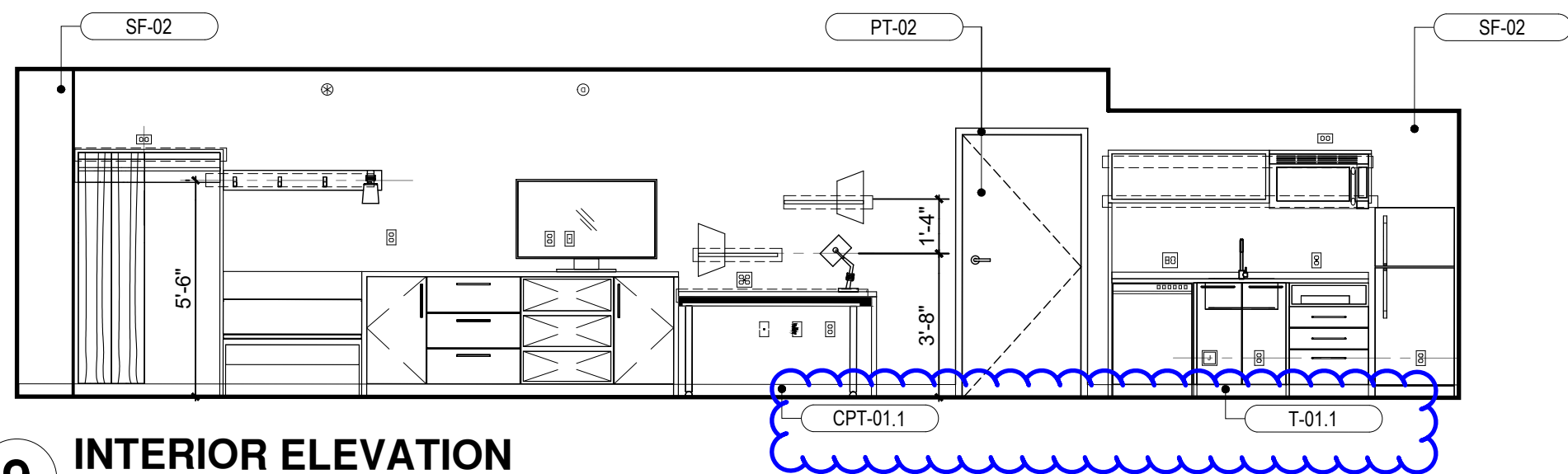
9 INTERIOR ELEVATION
