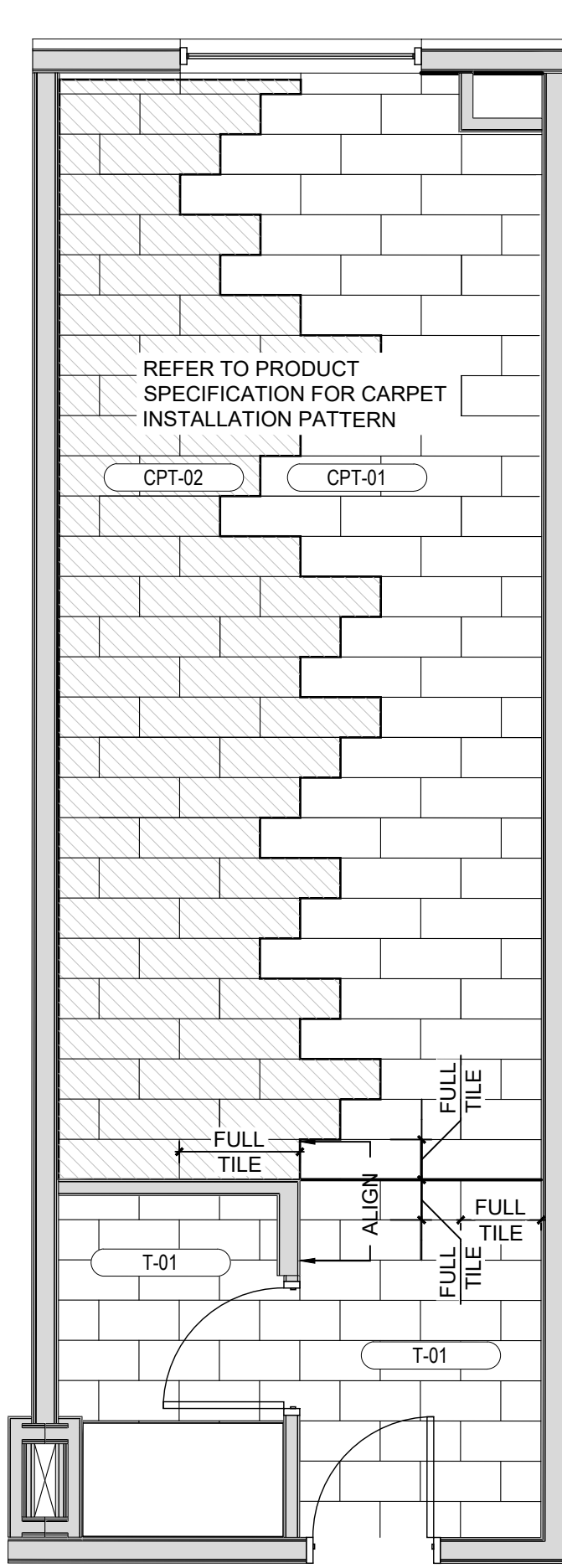
3 FINISH PLAN
