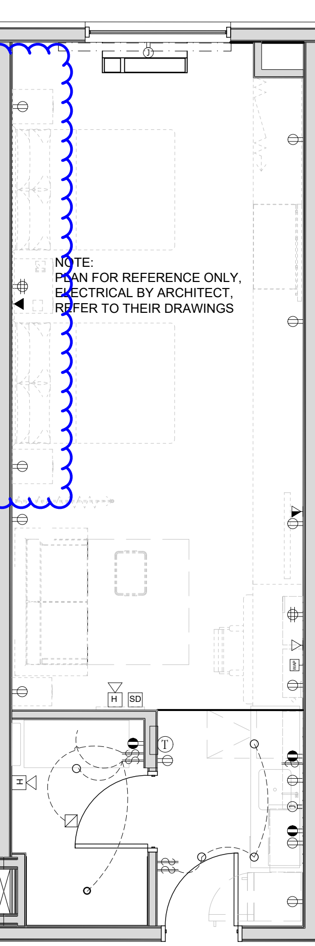
4 ELECTRICAL PLAN
