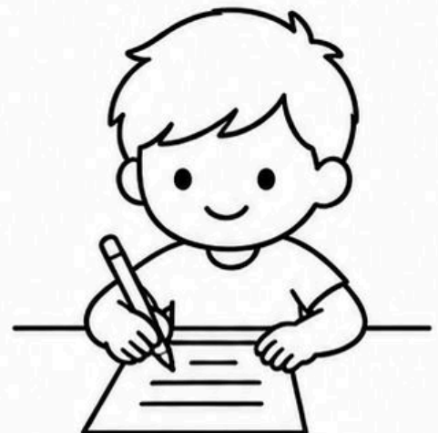
WRITE
