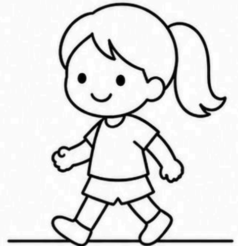
WALK
