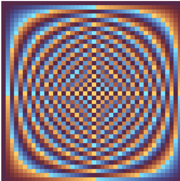
42 × 42 Fourier Matrix
