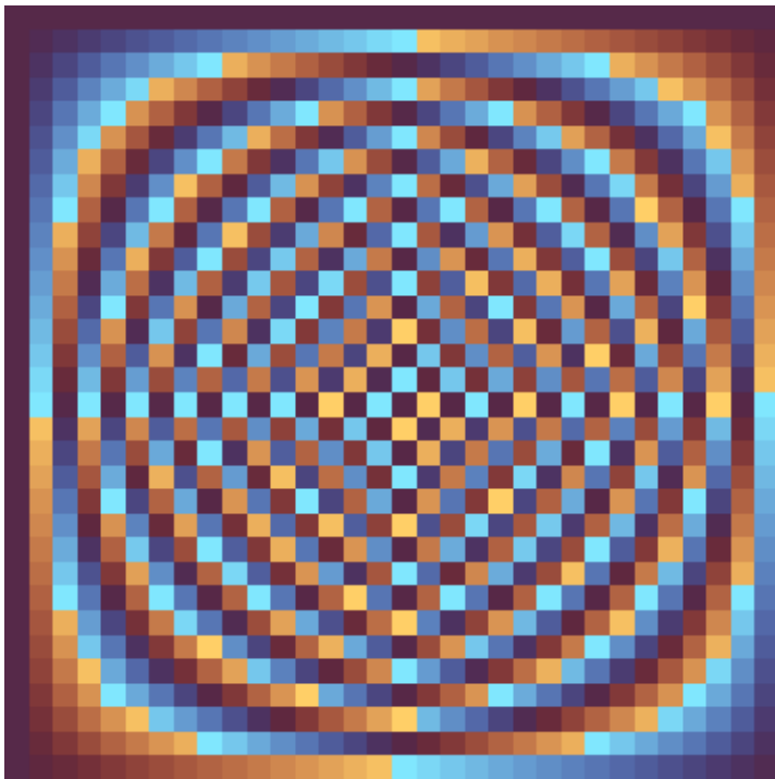
32 × 32 Fourier Matrix
