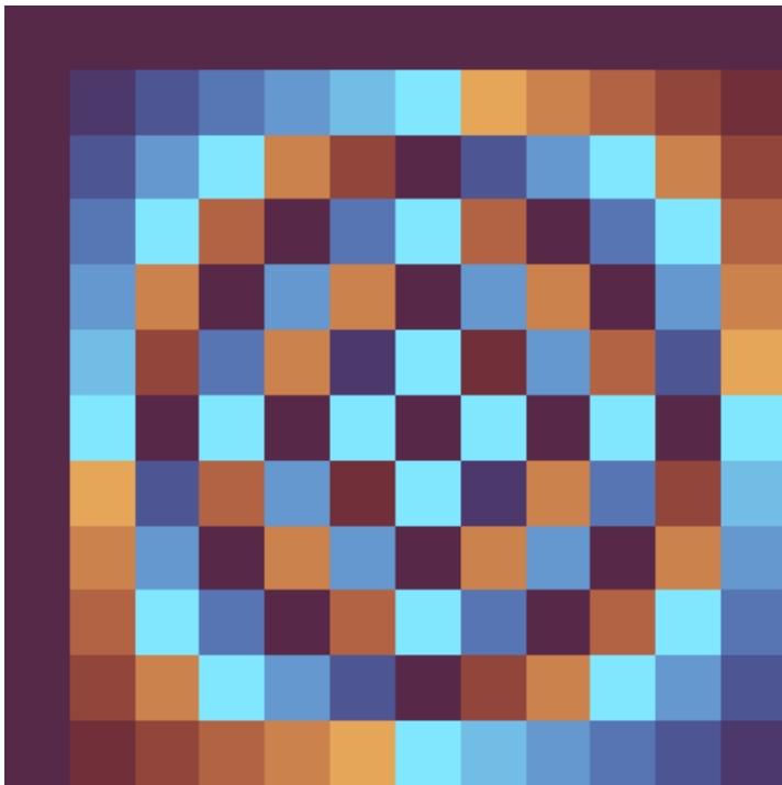
12 × 12 Fourier Matrix
