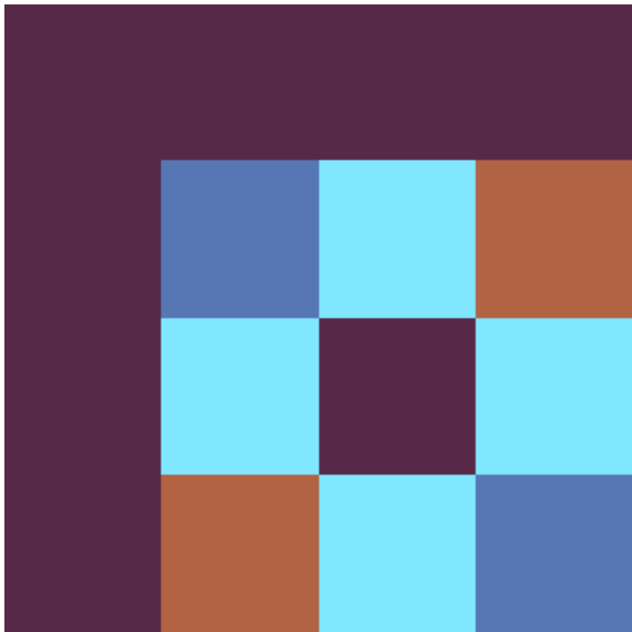
4 × 4 Fourier Matrix
