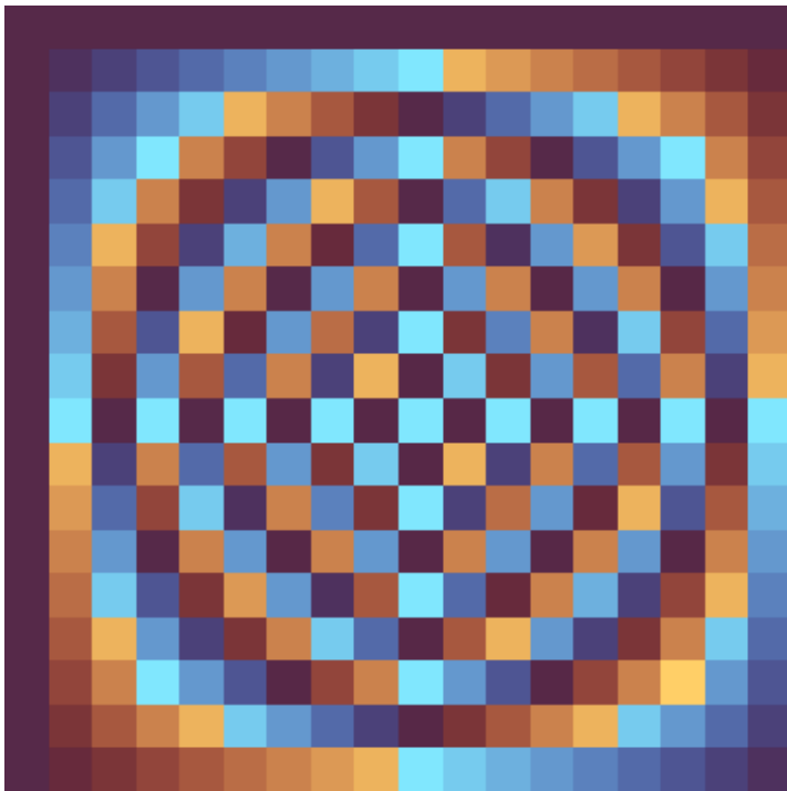
18 × 18 Fourier Matrix
