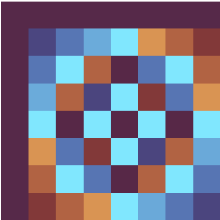
8 × 8 Fourier Matrix
