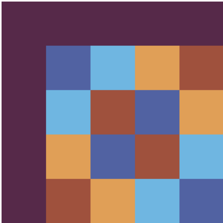
5 × 5 Fourier Matrix
