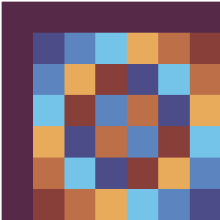
7 × 7 Fourier Matrix
