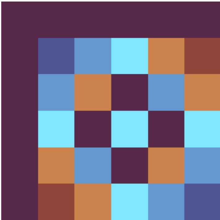
6 × 6 Fourier Matrix
