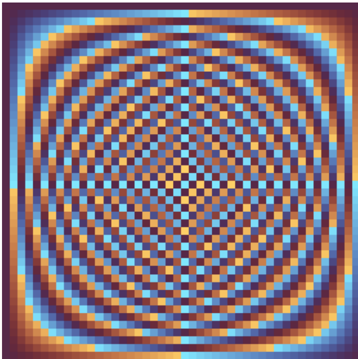
46 × 46 Fourier Matrix
