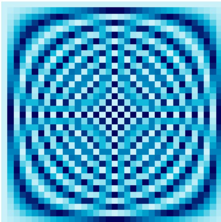
36 \times 36 Fourier Matrix
