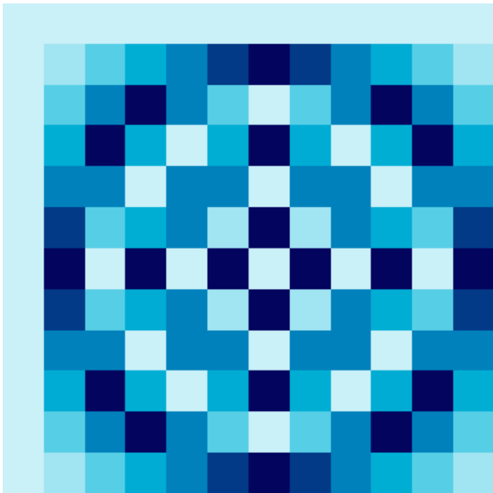
12 × 12 Fourier Matrix
