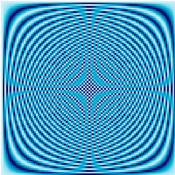
100 × 100 Fourier Matrix
