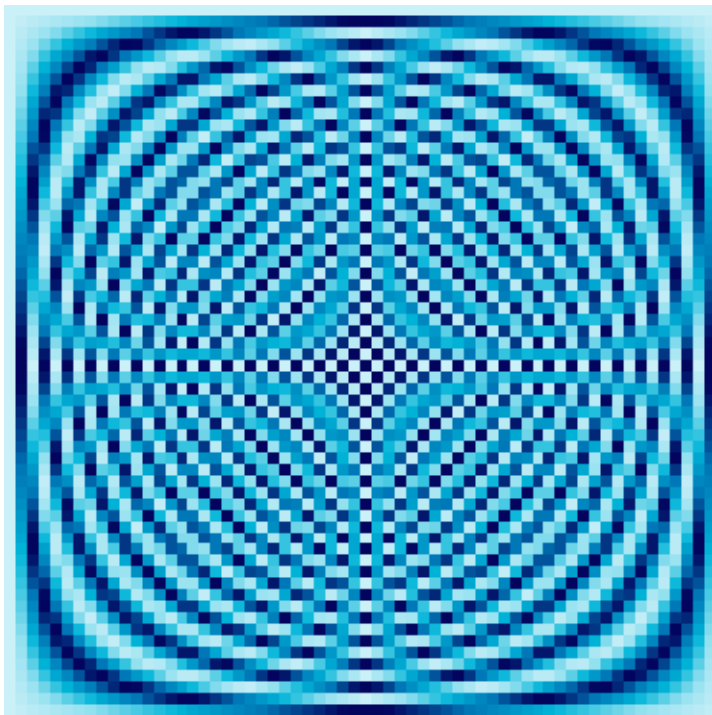
62 \times 62 Fourier Matrix
