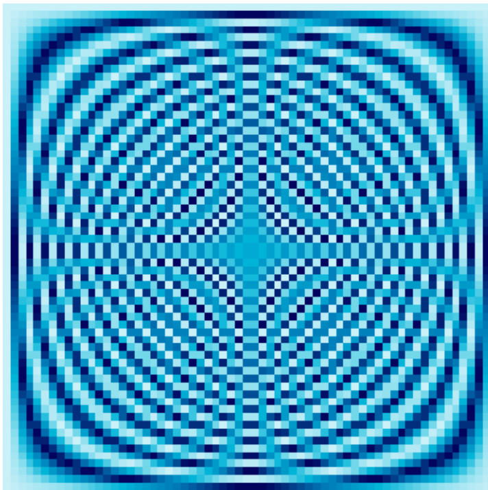
63 \times 63 Fourier Matrix
