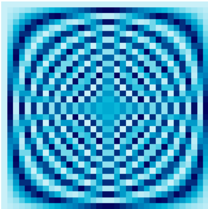
35 × 35 Fourier Matrix
