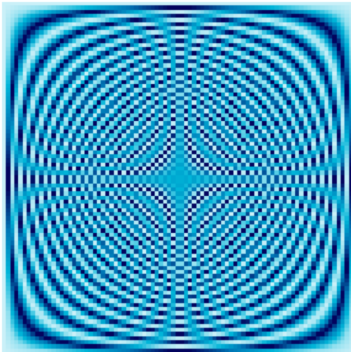
85 × 85 Fourier Matrix
