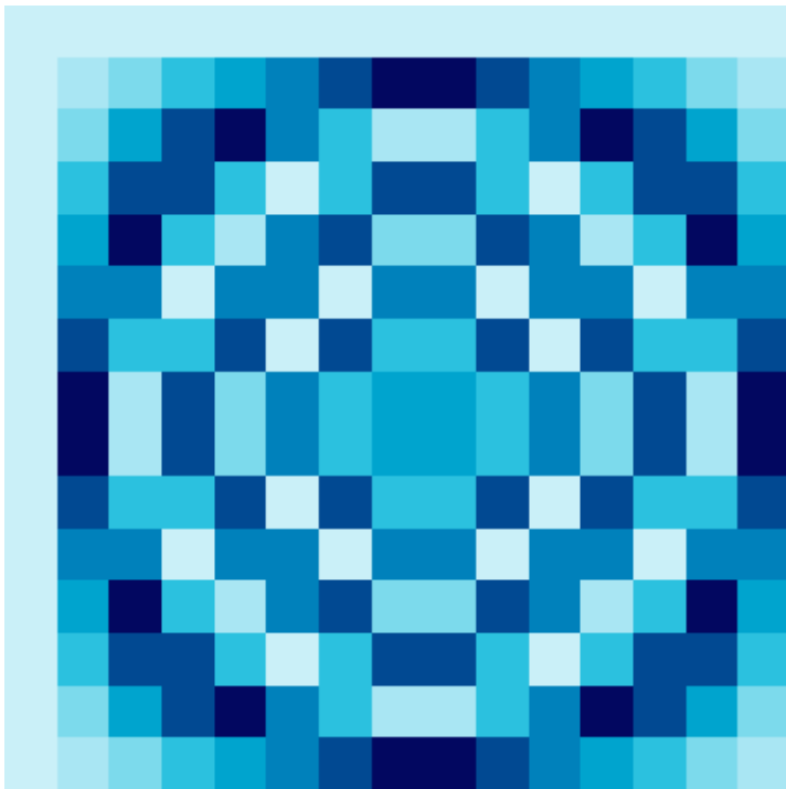
15 × 15 Fourier Matrix
