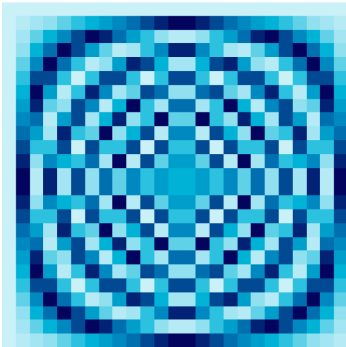
25 × 25 Fourier Matrix
