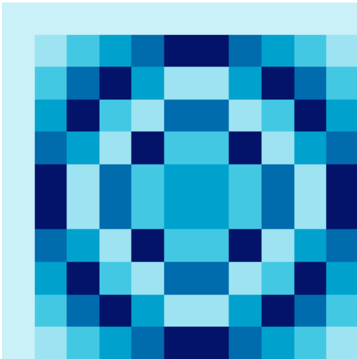
11 × 11 Fourier Matrix
