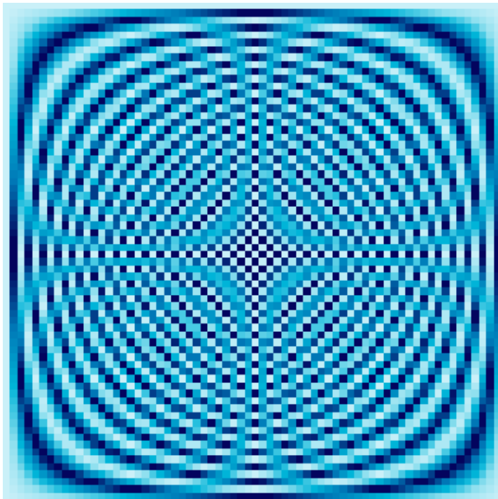
68 × 68 Fourier Matrix
