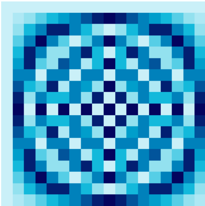
18 \times 18 Fourier Matrix
