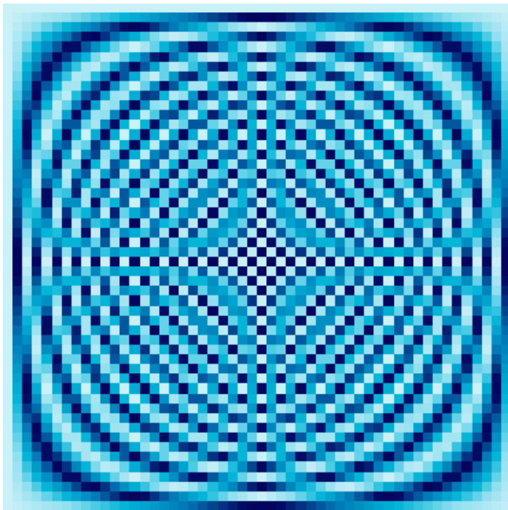
52 \times 52 Fourier Matrix
