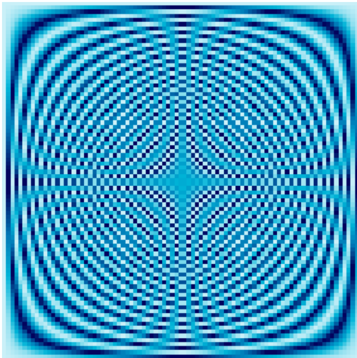
87 × 87 Fourier Matrix
