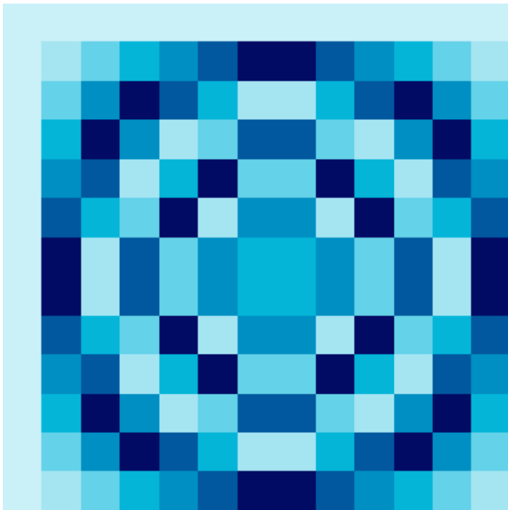
13 × 13 Fourier Matrix
