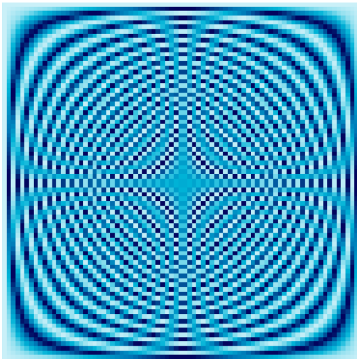
79 \times 79 Fourier Matrix
