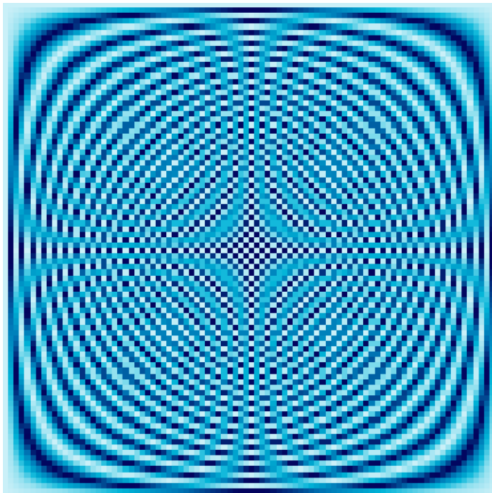
90 \times 90 Fourier Matrix
