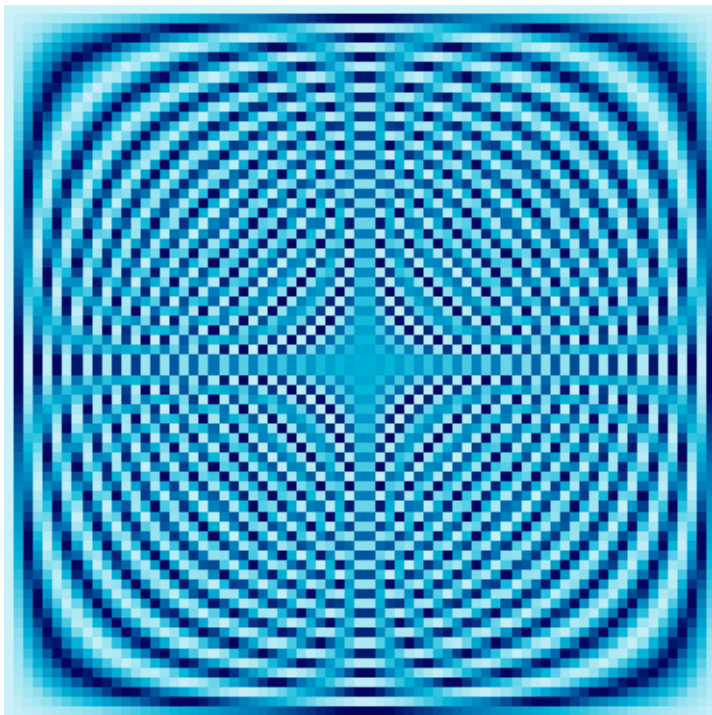
73 \times 73 Fourier Matrix
