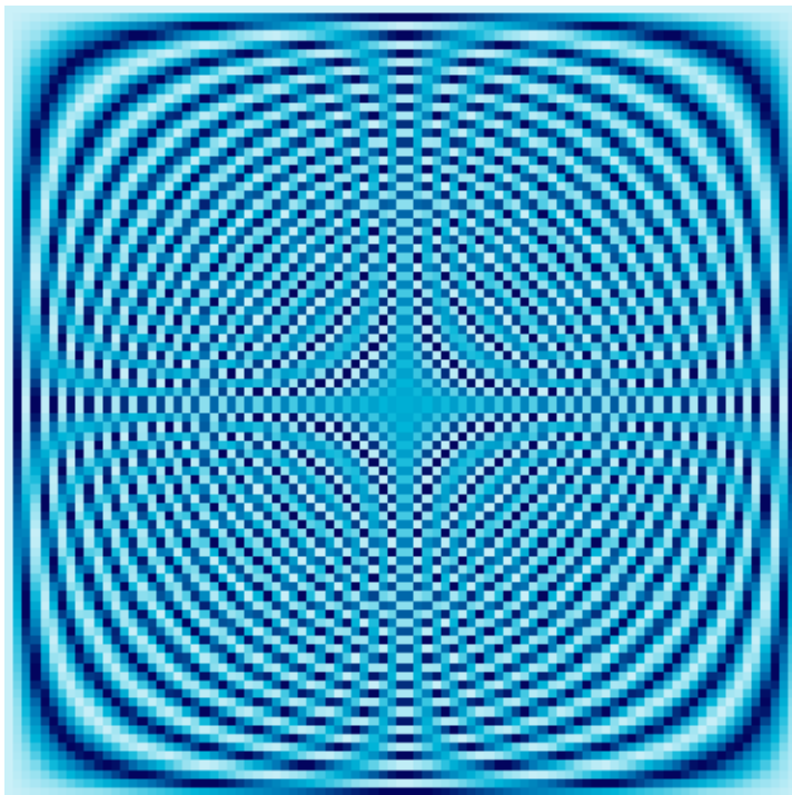
89 \times 89 Fourier Matrix
