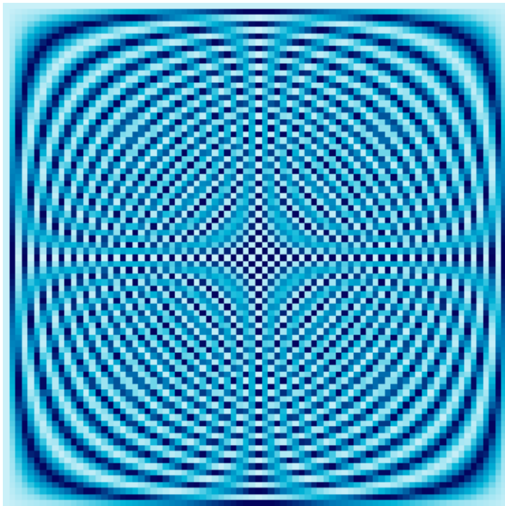
82 \times 82 Fourier Matrix
