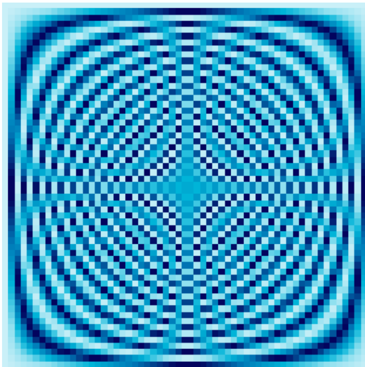
59 \times 59 Fourier Matrix
