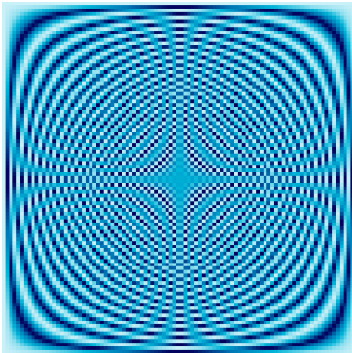
97 \times 97 Fourier Matrix
