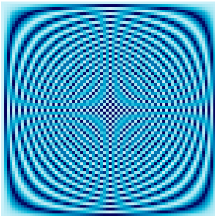
76 \times 76 Fourier Matrix
