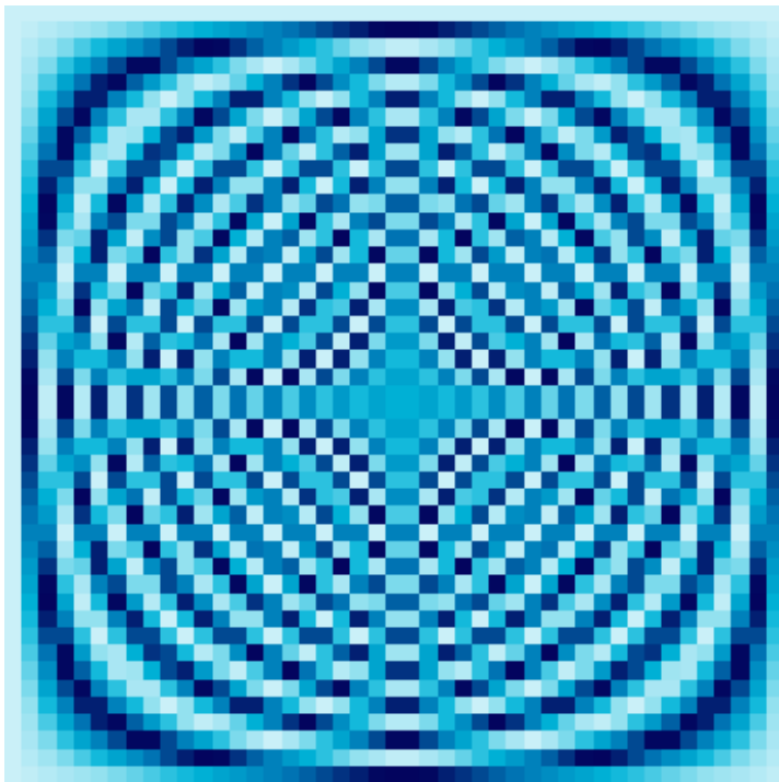
45 \times 45 Fourier Matrix
