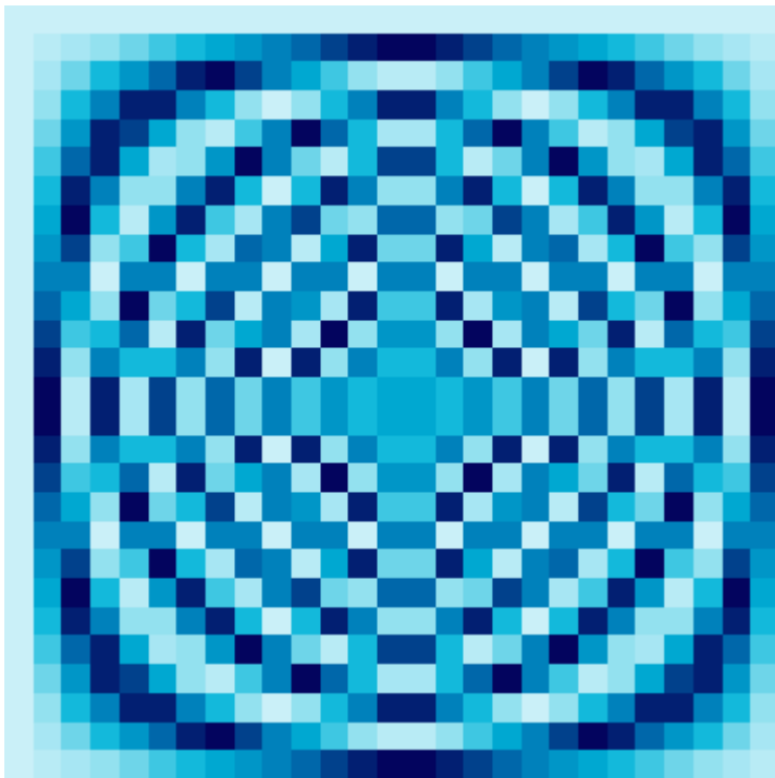
27 × 27 Fourier Matrix
