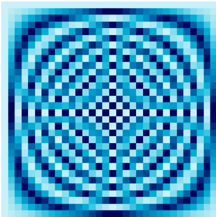
32 \times 32 Fourier Matrix
