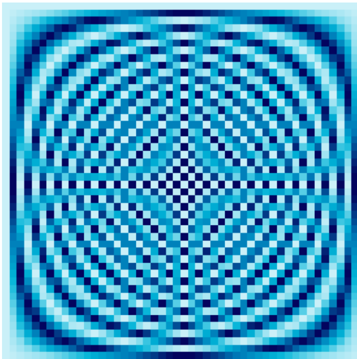
48 × 48 Fourier Matrix
