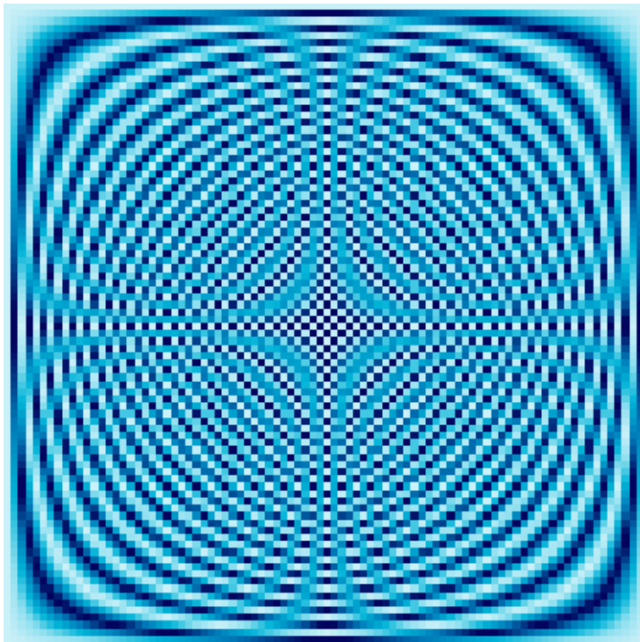
88 × 88 Fourier Matrix
