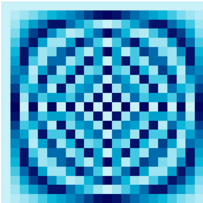
22 \times 22 Fourier Matrix
