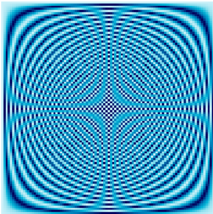
98 × 98 Fourier Matrix
