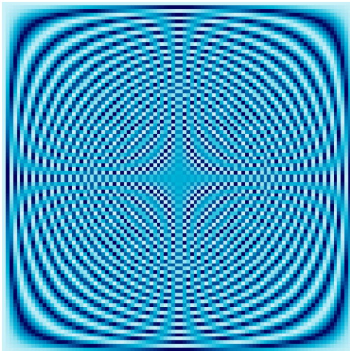
95 \times 95 Fourier Matrix
