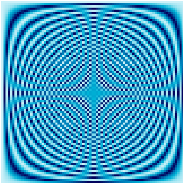
81 \times 81 Fourier Matrix
