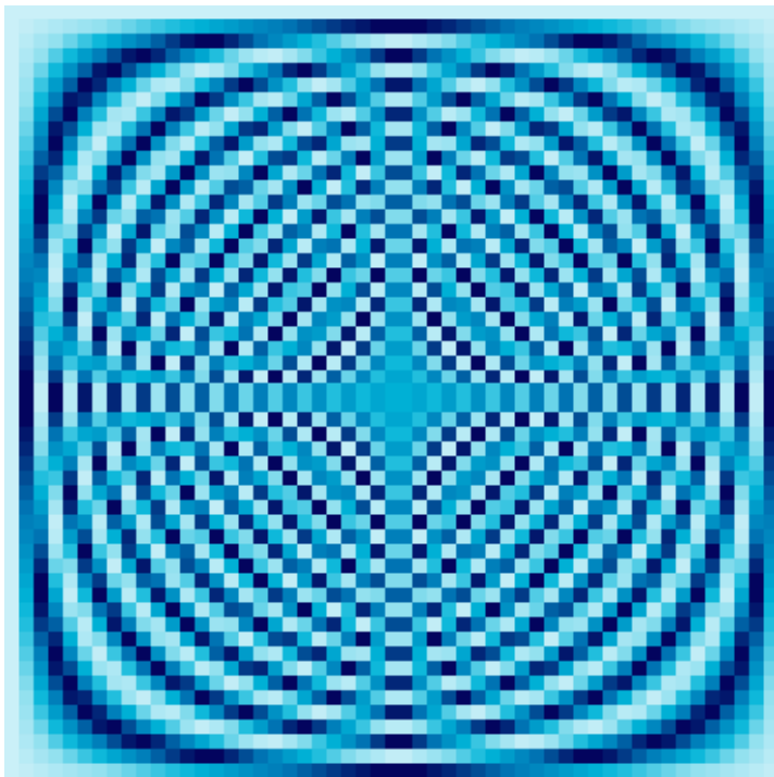
53 \times 53 Fourier Matrix
