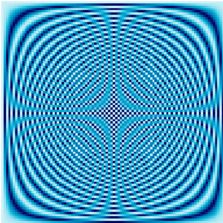
96 \times 96 Fourier Matrix
