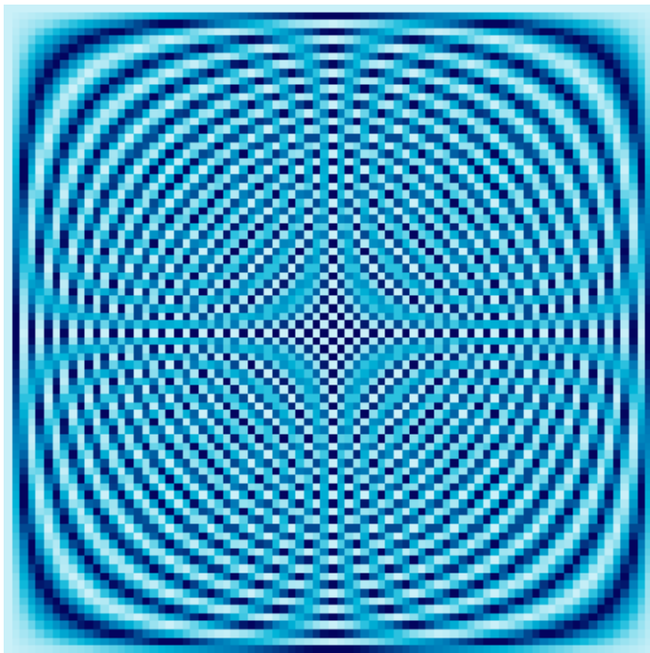
80 × 80 Fourier Matrix
