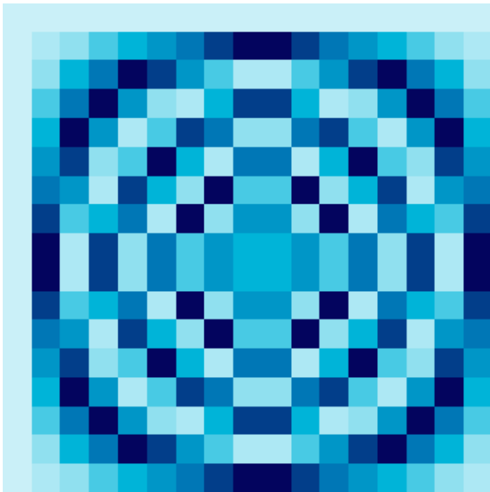
17 × 17 Fourier Matrix
