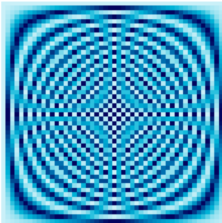
50 × 50 Fourier Matrix
