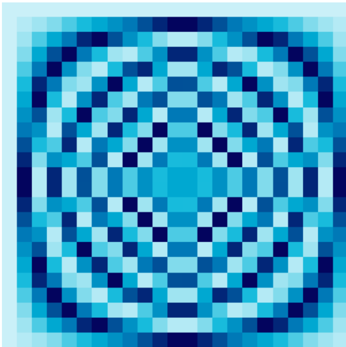
23 × 23 Fourier Matrix
