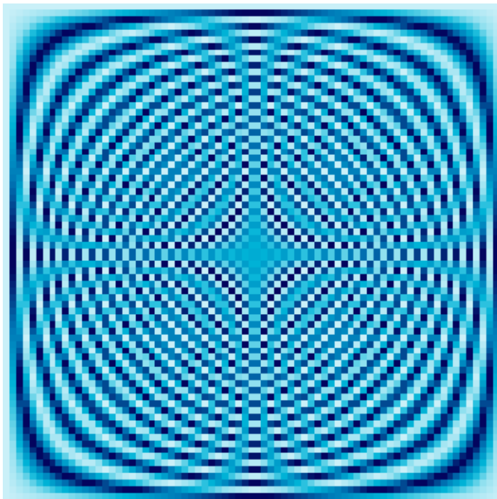
75 \times 75 Fourier Matrix
