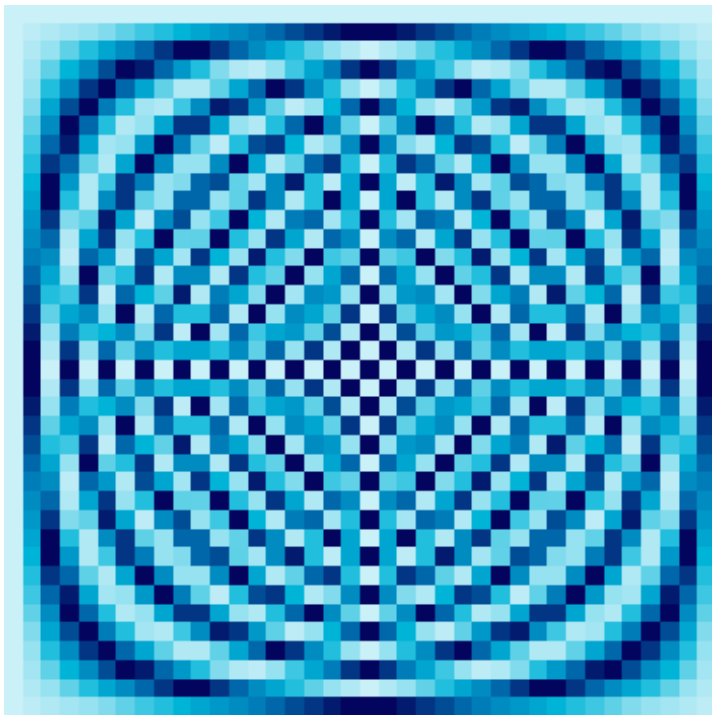
38 × 38 Fourier Matrix
