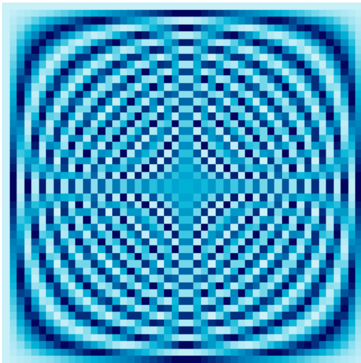
49 × 49 Fourier Matrix
