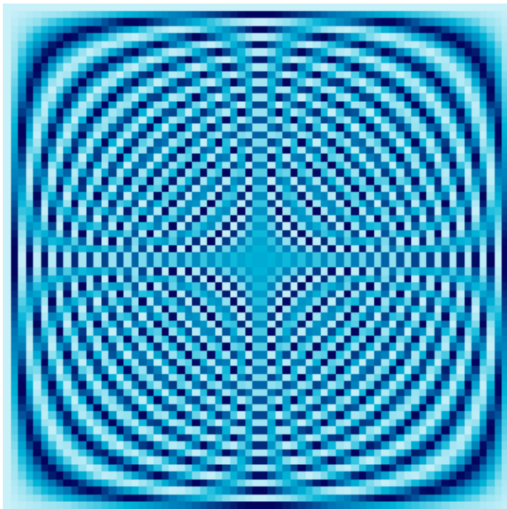
67 × 67 Fourier Matrix
