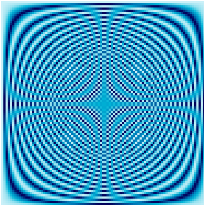
93 \times 93 Fourier Matrix
