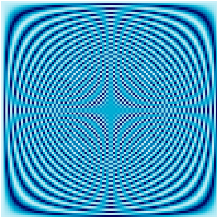
99 \times 99 Fourier Matrix
