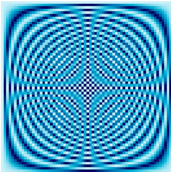
66 × 66 Fourier Matrix
