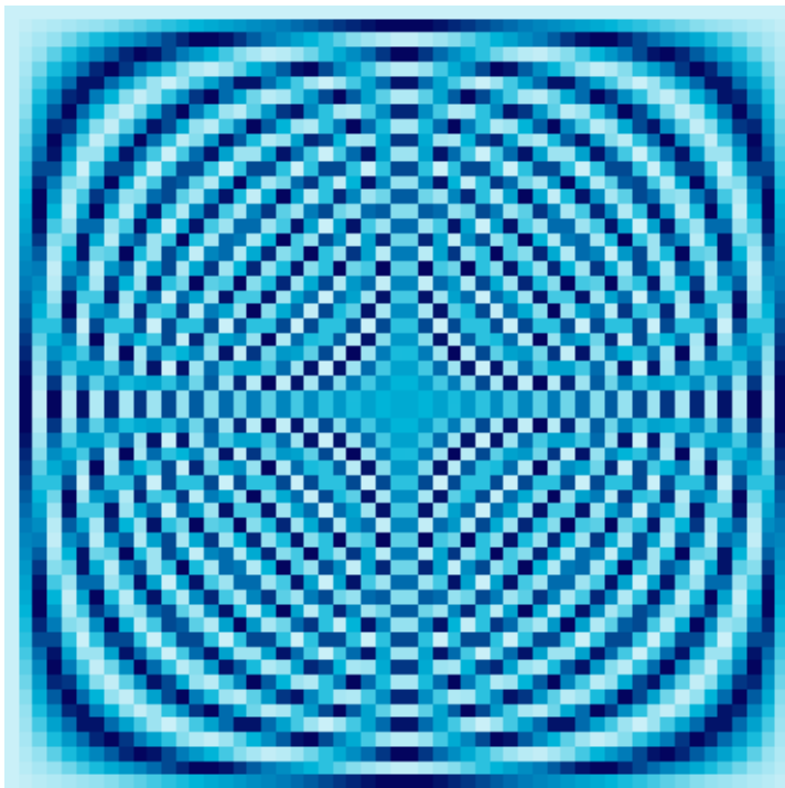
55 \times 55 Fourier Matrix
