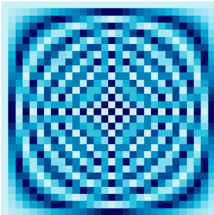
30 × 30 Fourier Matrix
