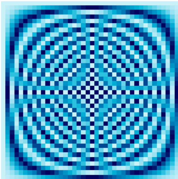
40 × 40 Fourier Matrix
