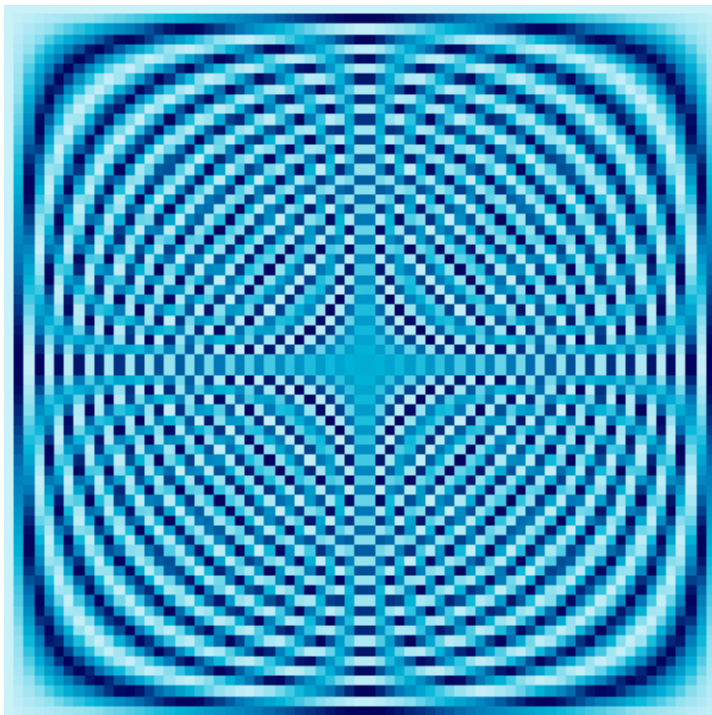
71 \times 71 Fourier Matrix
