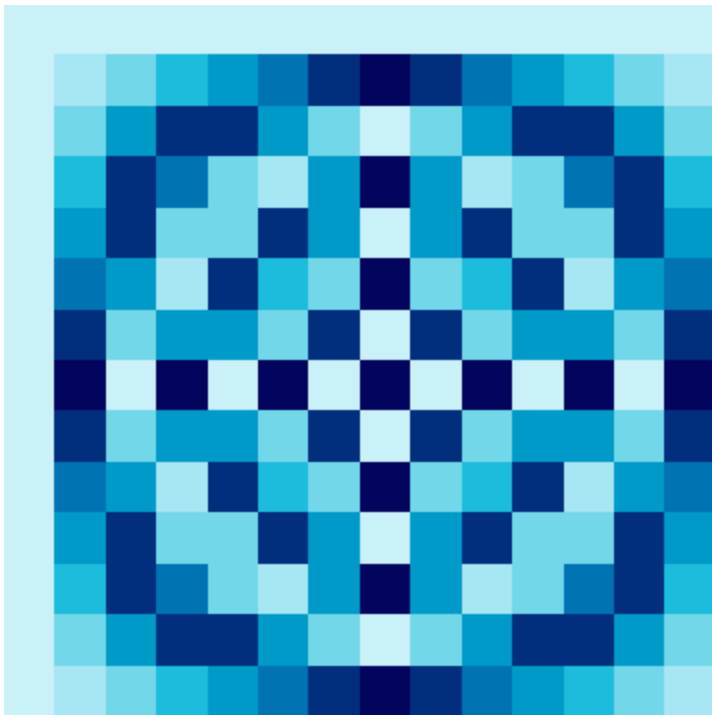
14 × 14 Fourier Matrix
