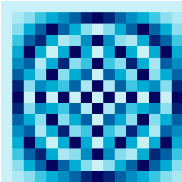
16 × 16 Fourier Matrix
