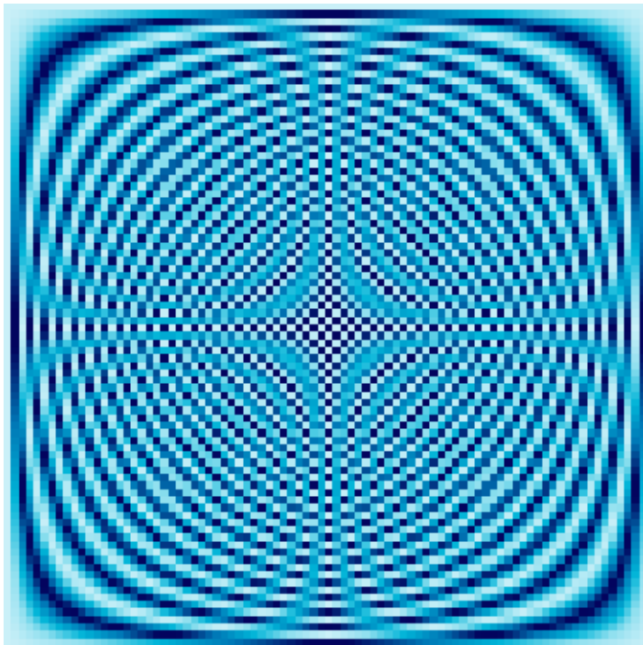
86 × 86 Fourier Matrix
