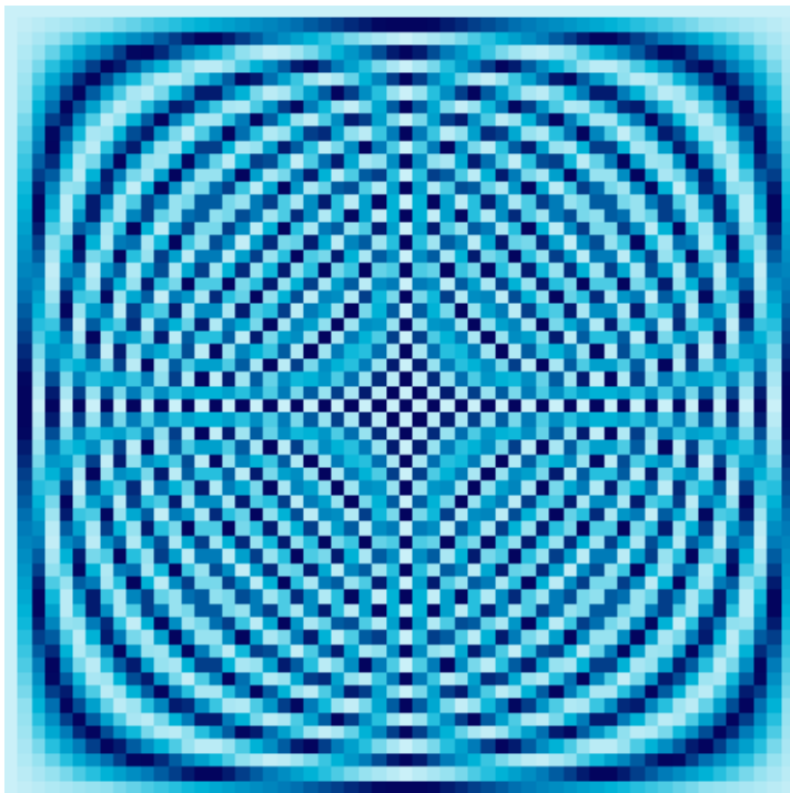
58 \times 58 Fourier Matrix
