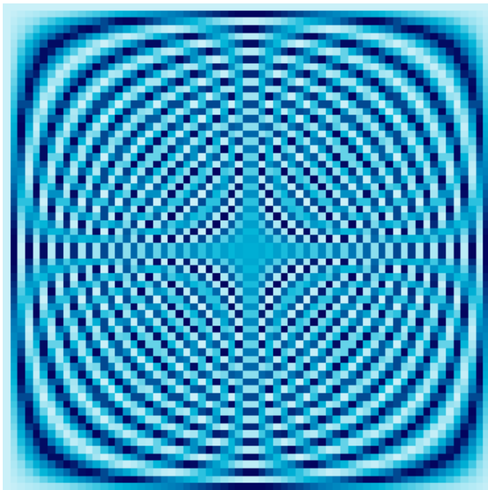
65 \times 65 Fourier Matrix
