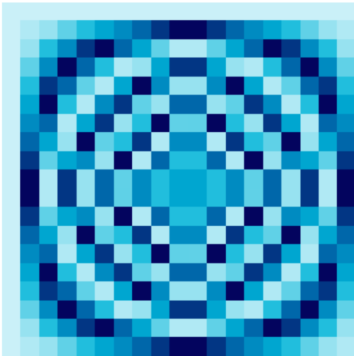
19 × 19 Fourier Matrix
