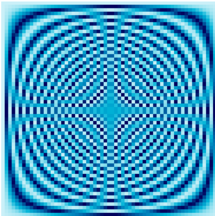
61 \times 61 Fourier Matrix
