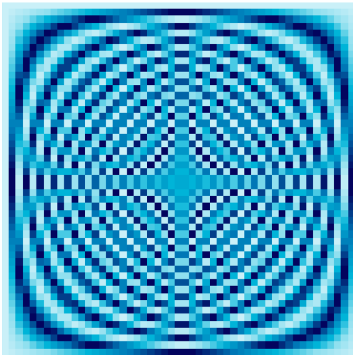
51 \times 51 Fourier Matrix
