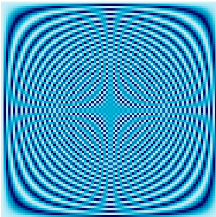
91 \times 91 Fourier Matrix
