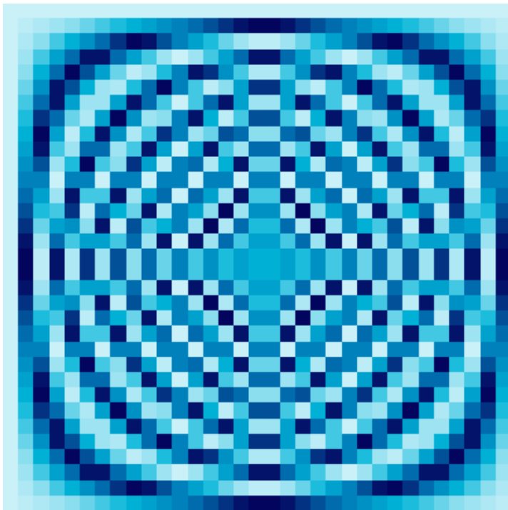
33 \times 33 Fourier Matrix
