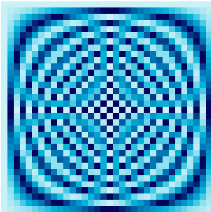
34 × 34 Fourier Matrix
