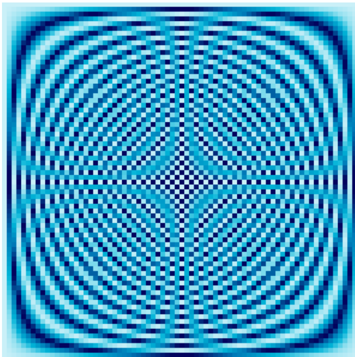
74 \times 74 Fourier Matrix
