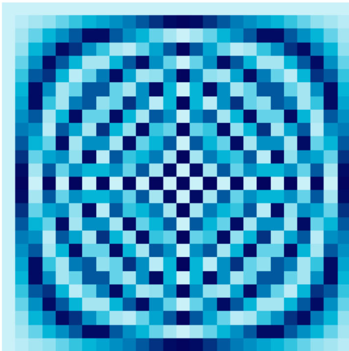
26 \times 26 Fourier Matrix
