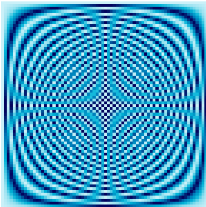
72 \times 72 Fourier Matrix
