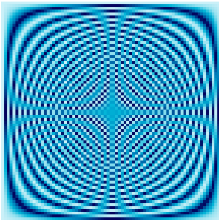
77 × 77 Fourier Matrix
