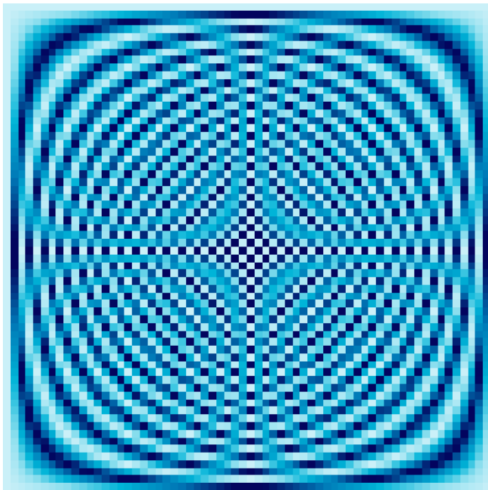
64 \times 64 Fourier Matrix
