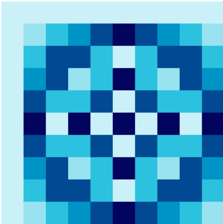
10 × 10 Fourier Matrix
