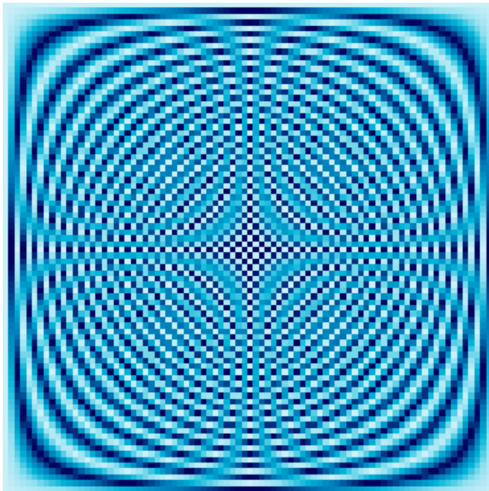
84 × 84 Fourier Matrix
