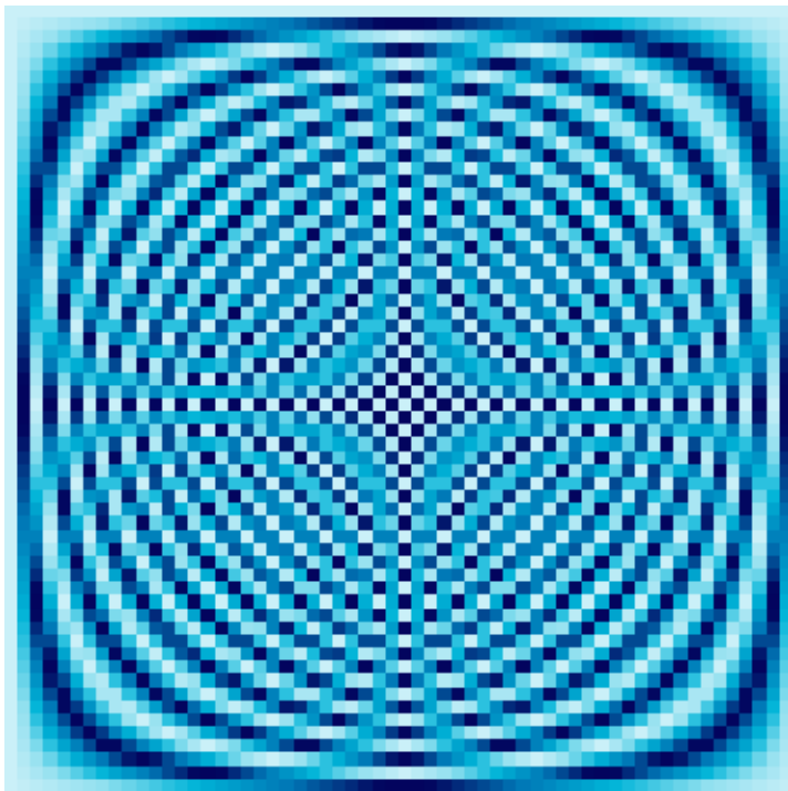
60 \times 60 Fourier Matrix
