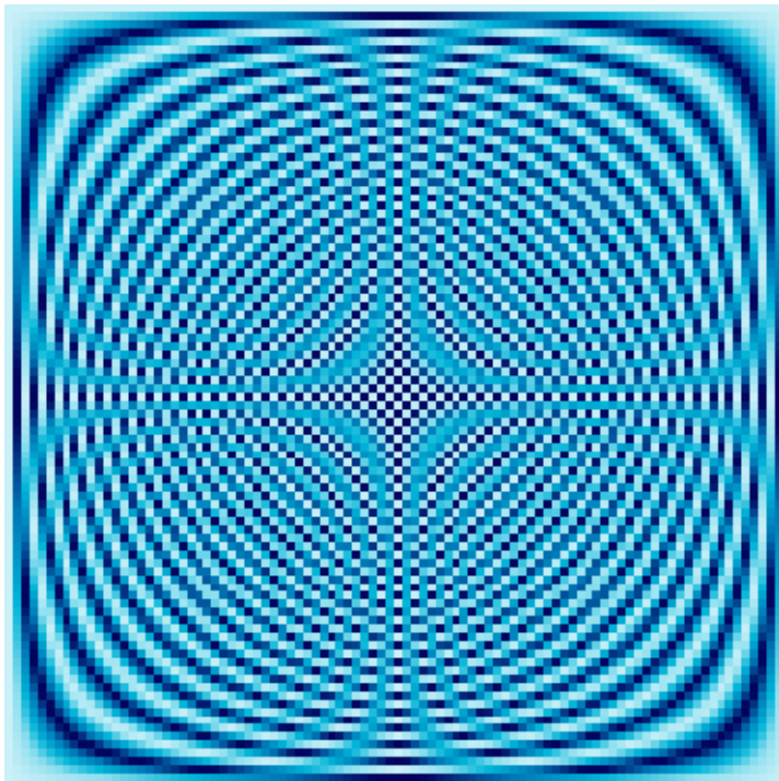
94 \times 94 Fourier Matrix
