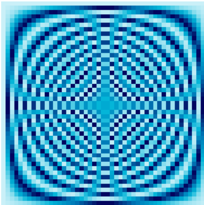
47 × 47 Fourier Matrix
