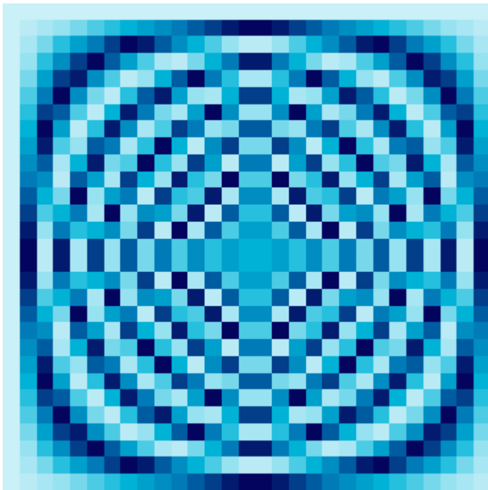
29 × 29 Fourier Matrix
