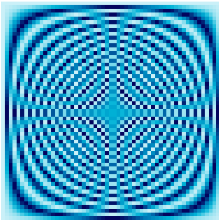
57 \times 57 Fourier Matrix
