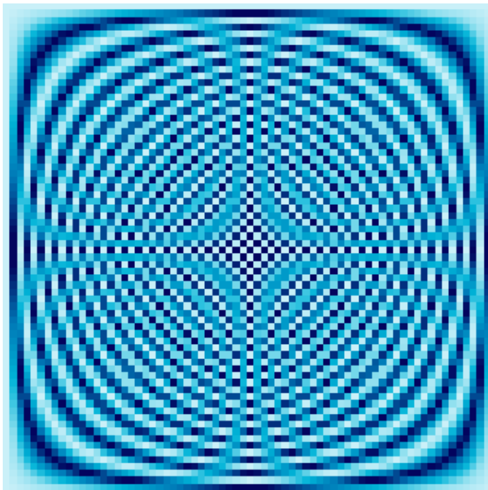
70 \times 70 Fourier Matrix
