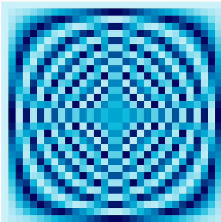
31 \times 31 Fourier Matrix
