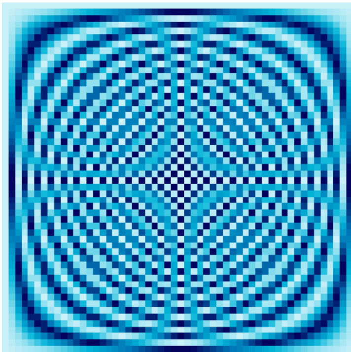
54 \times 54 Fourier Matrix
