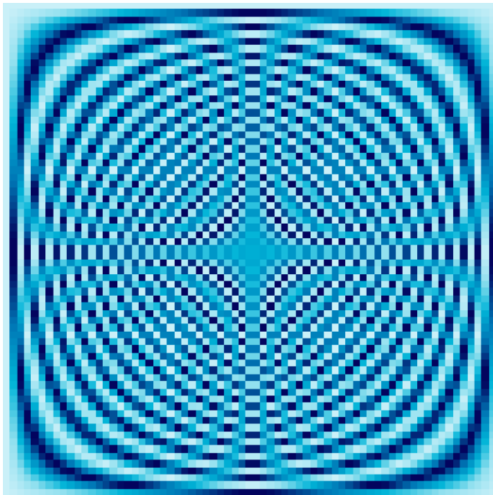
69 \times 69 Fourier Matrix
