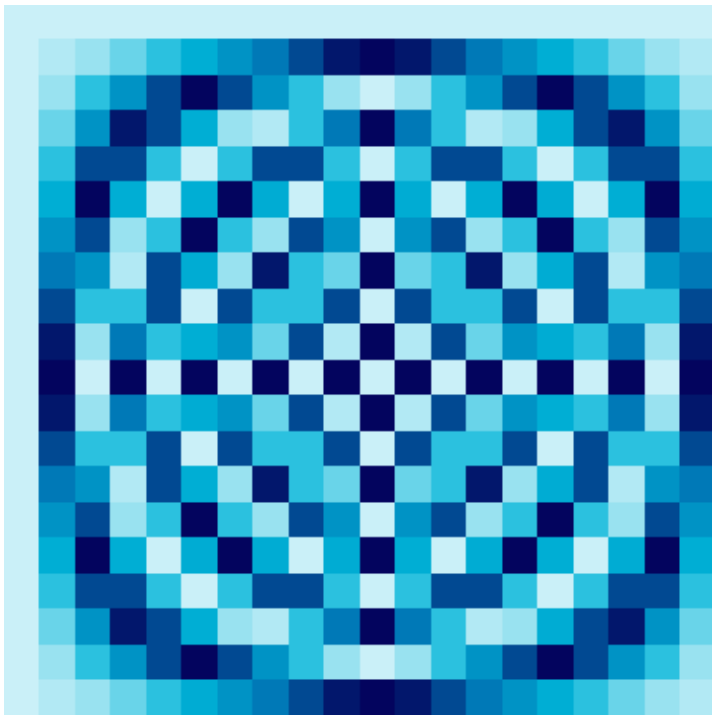
20 × 20 Fourier Matrix
