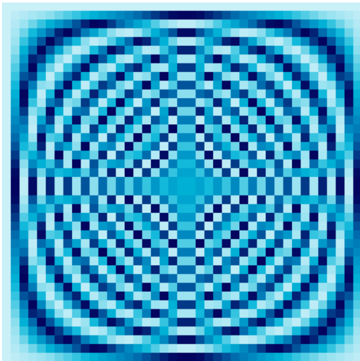
41 \times 41 Fourier Matrix
