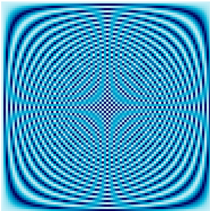
92 \times 92 Fourier Matrix
