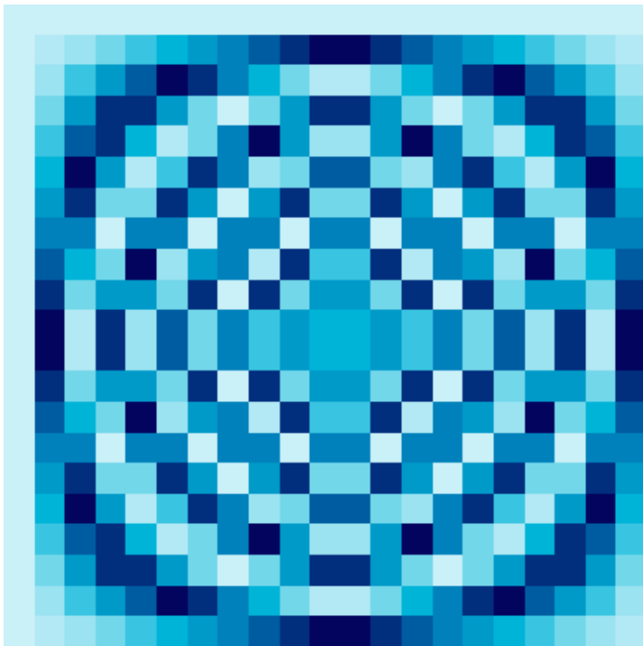
21 \times 21 Fourier Matrix
