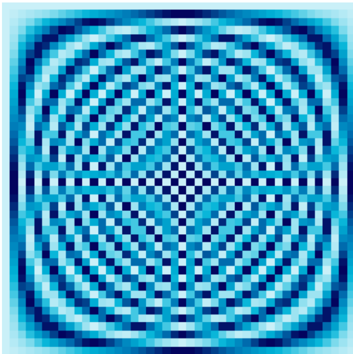
44 × 44 Fourier Matrix
