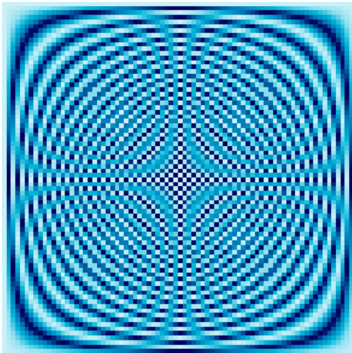
78 × 78 Fourier Matrix
