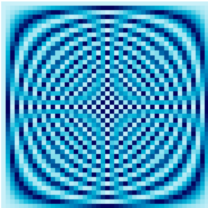
46 \times 46 Fourier Matrix
