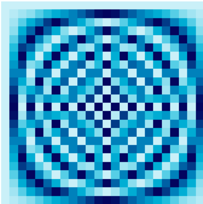
24 × 24 Fourier Matrix
