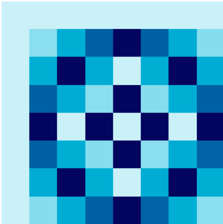
8 × 8 Fourier Matrix
