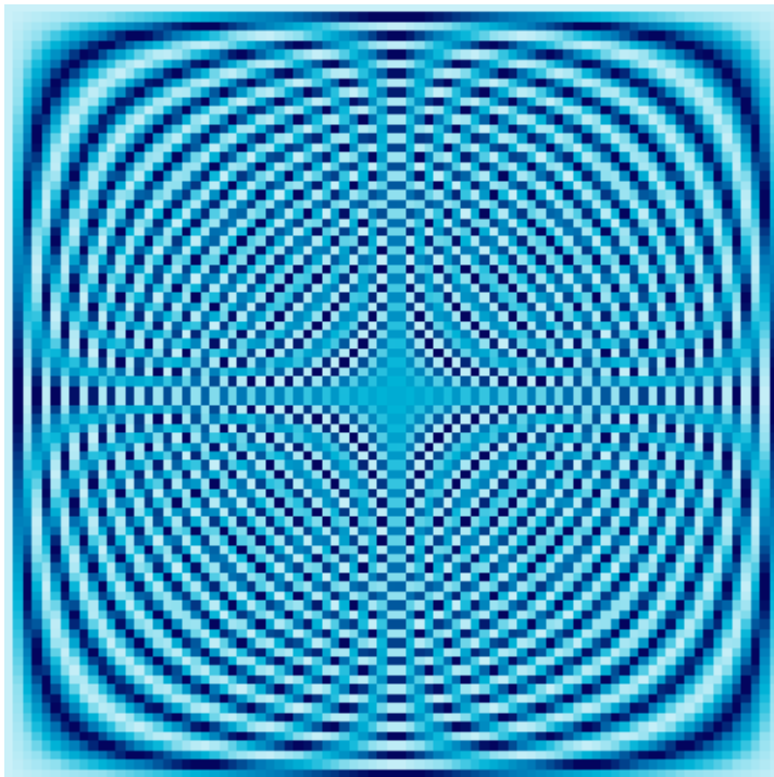
83 \times 83 Fourier Matrix
