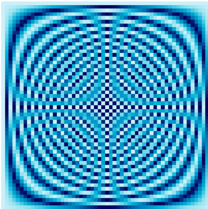
56 \times 56 Fourier Matrix
