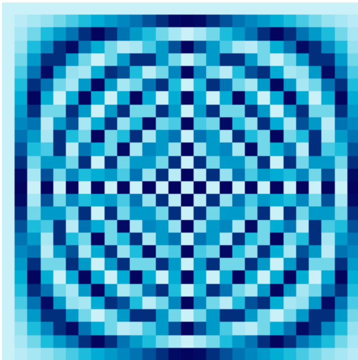
28 × 28 Fourier Matrix
