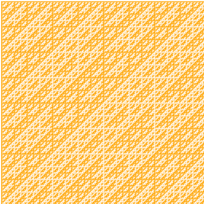
256 \times 256 Hadamard Matrix
