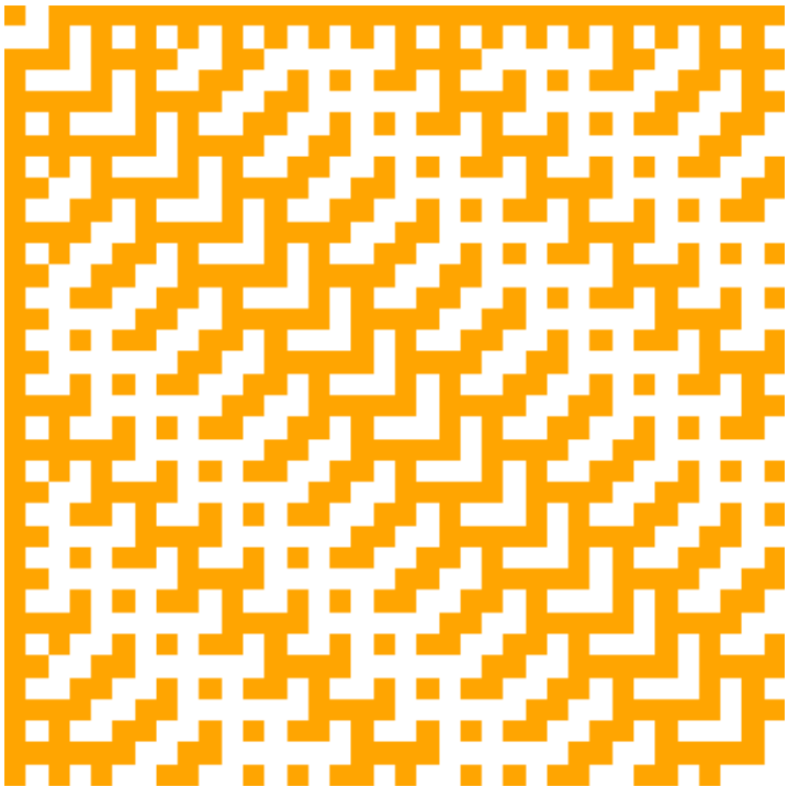
36 \times 36 Hadamard Matrix
