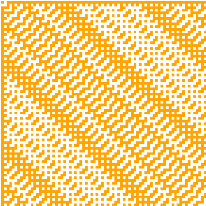
76 × 76 Hadamard Matrix
