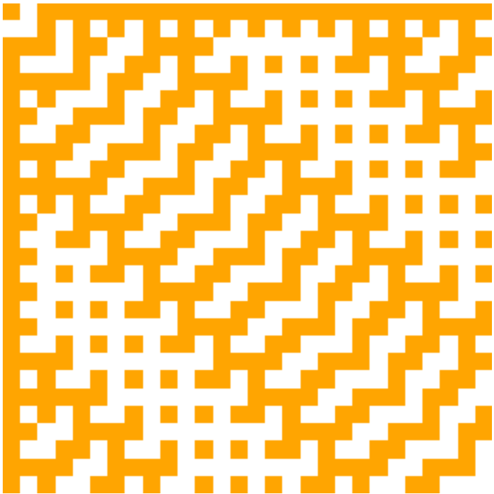
28 × 28 Hadamard Matrix
