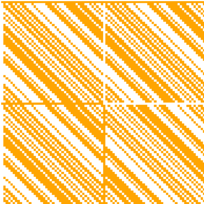
88 × 88 Hadamard Matrix
