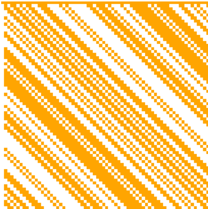
68 × 68 Hadamard Matrix
