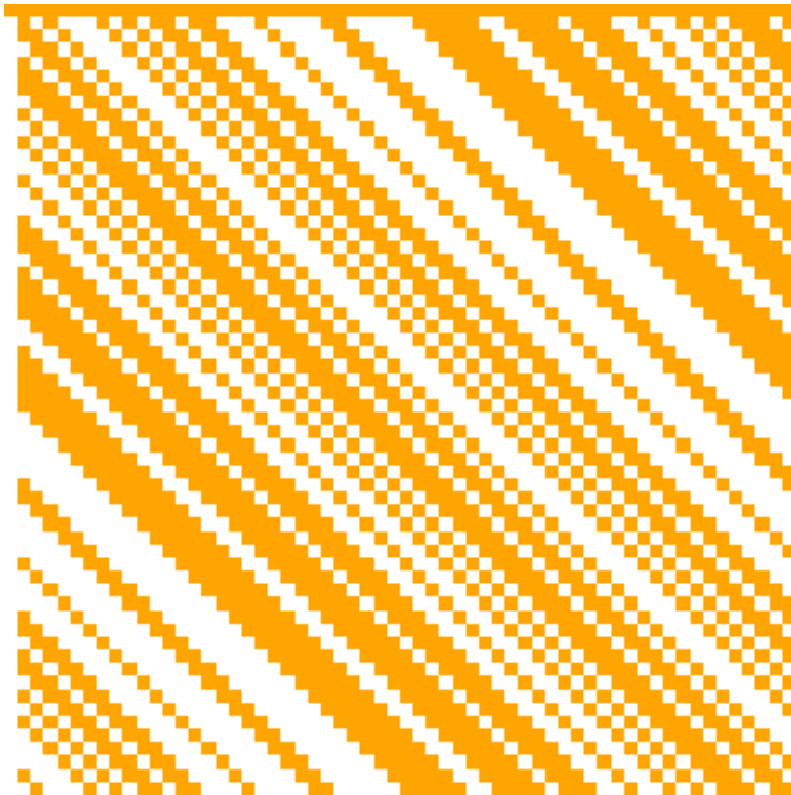
60 × 60 Hadamard Matrix
