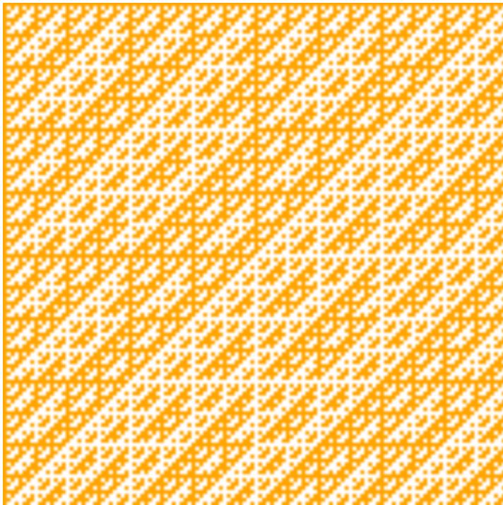
128 × 128 Hadamard Matrix
