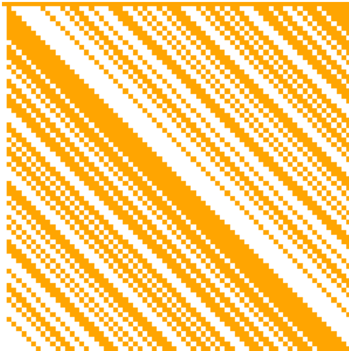
72 × 72 Hadamard Matrix
