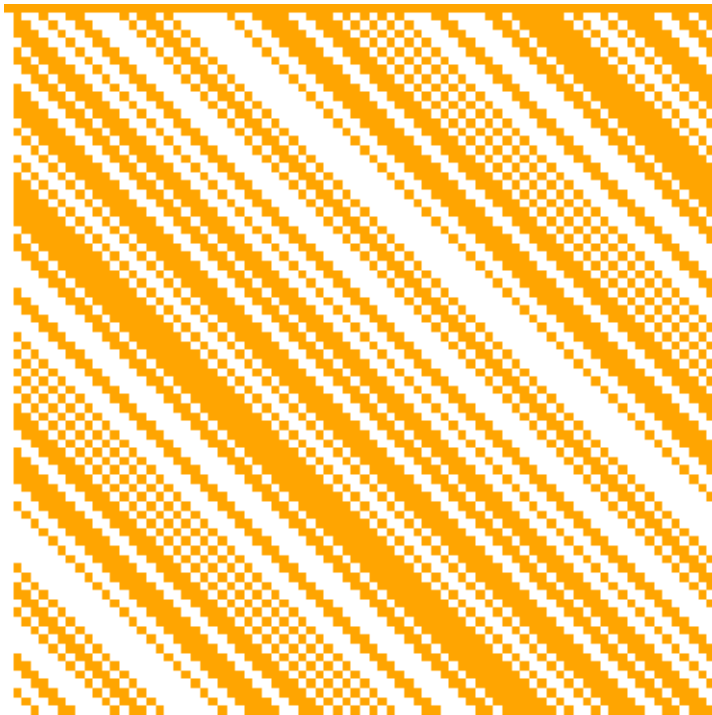
80 × 80 Hadamard Matrix
