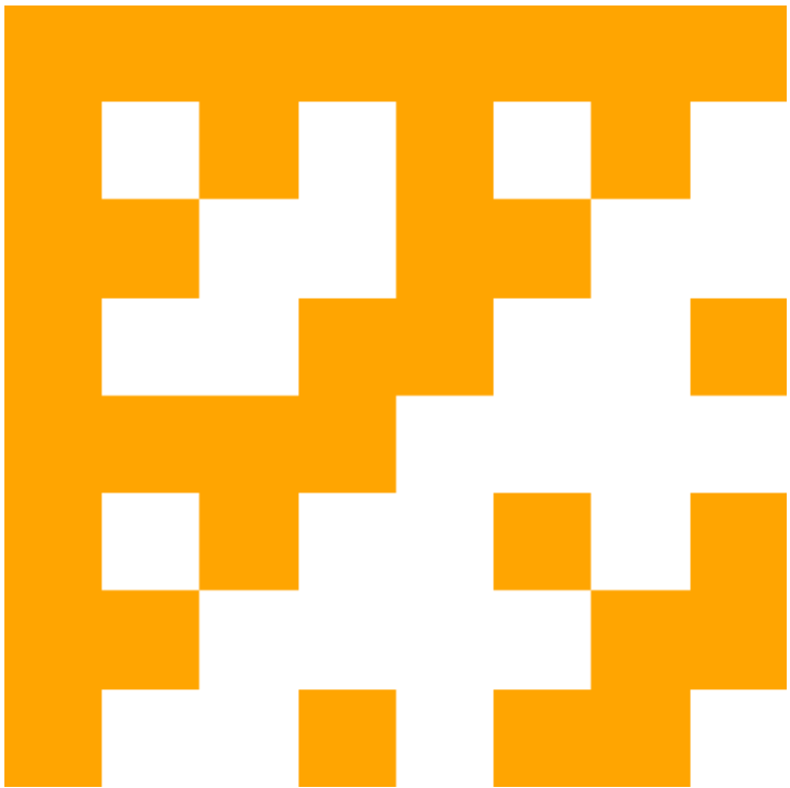
8 × 8 Hadamard Matrix
