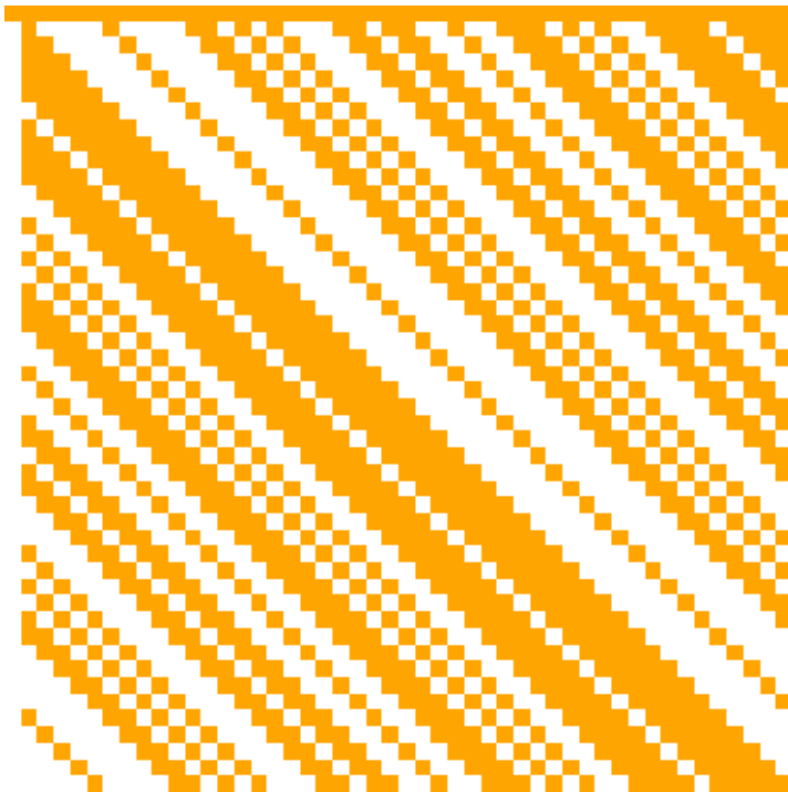
48 × 48 Hadamard Matrix
