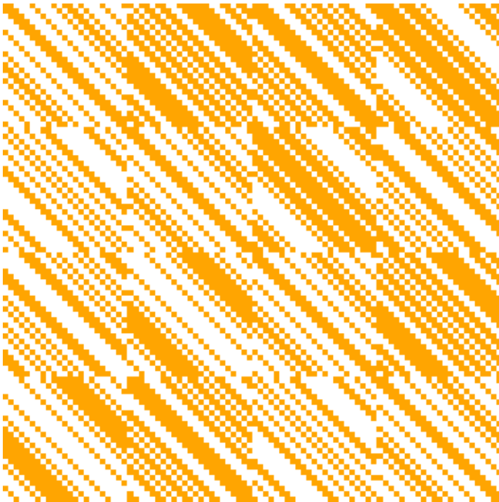
92 \times 92 Hadamard Matrix
