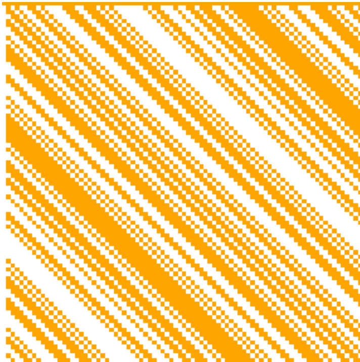
84 × 84 Hadamard Matrix
