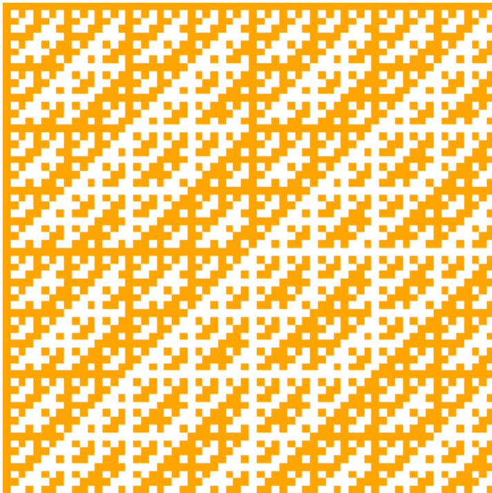
64 × 64 Hadamard Matrix
