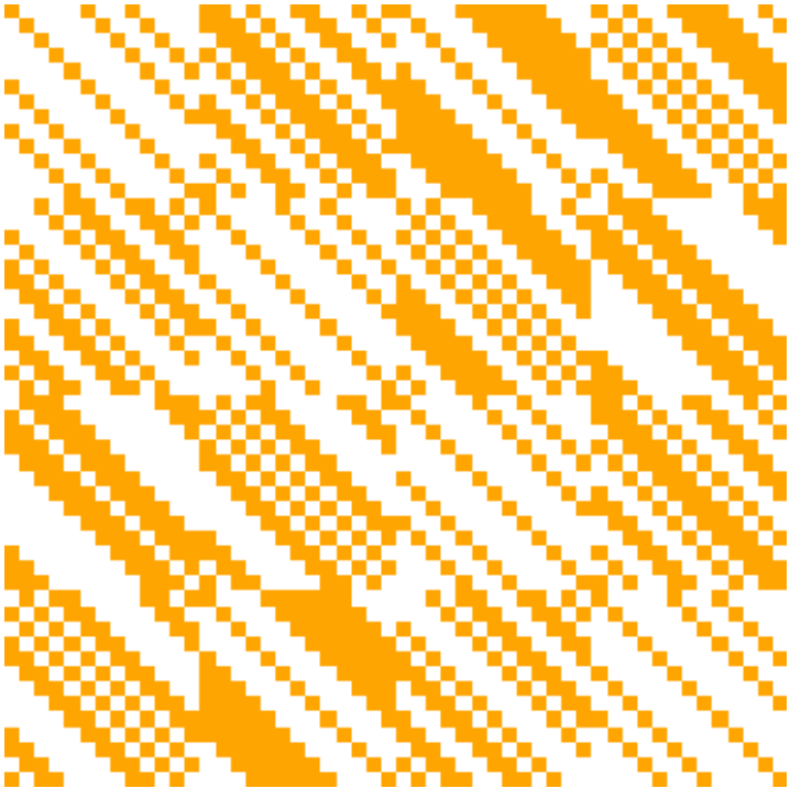
52 \times 52 Hadamard Matrix
