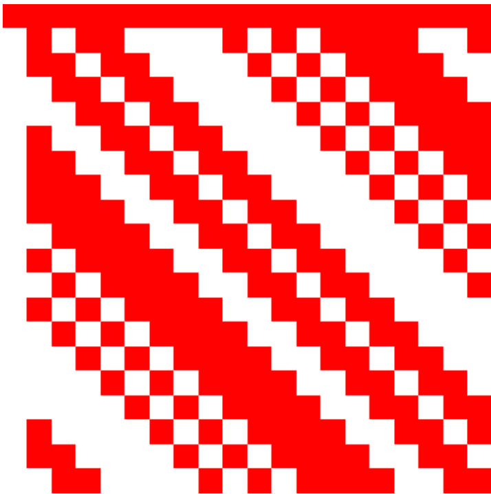
20 x 20 Paley construction (1)
