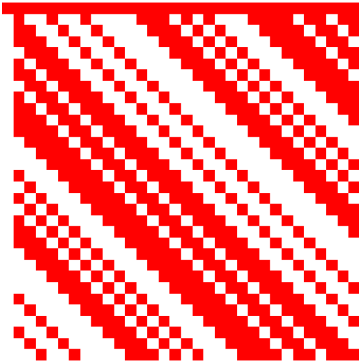
32 x 32 Paley construction (1)
