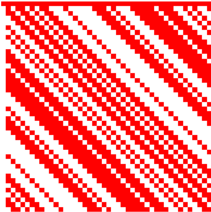
44 x 44 Paley construction (1)
