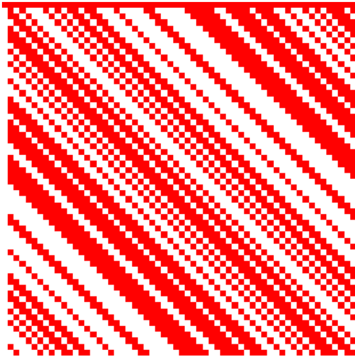
60 \times 60 Paley construction (1)
