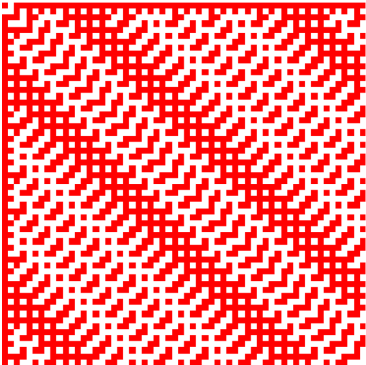
60 \times 60 Paley construction (2)
