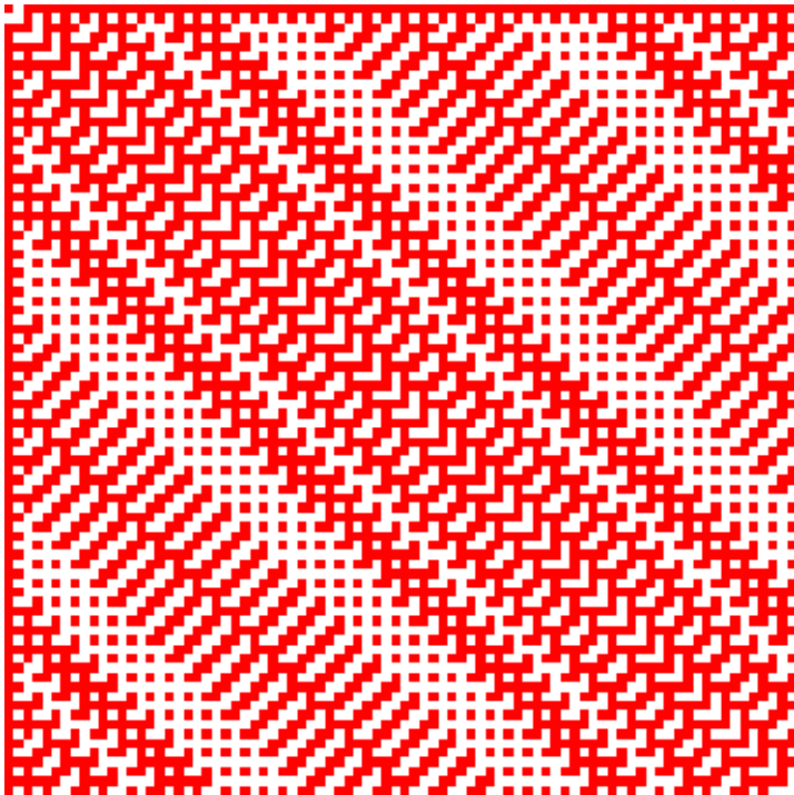
84 × 84 Paley construction (2)
