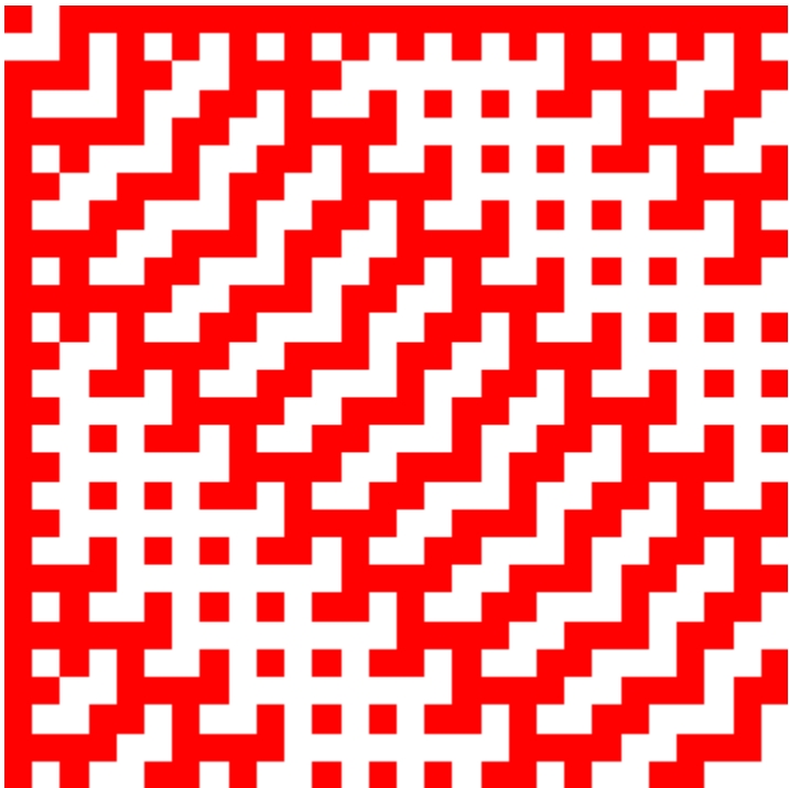
28 x 28 Paley construction (2)
