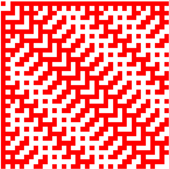
36 \times 36 Paley construction (2)
