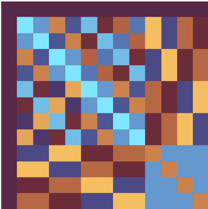
13 × 13 Petrescu Matrix
