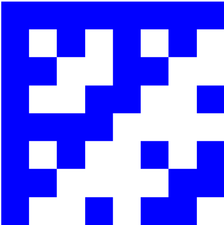
8 × 8 Sylvester construction
