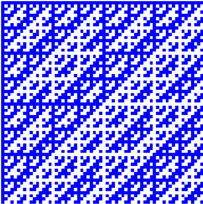
64 × 64 Sylvester construction
