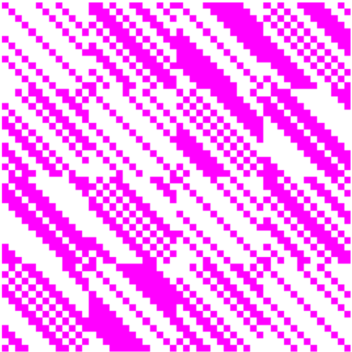
52 \times 52 Williamson construction
