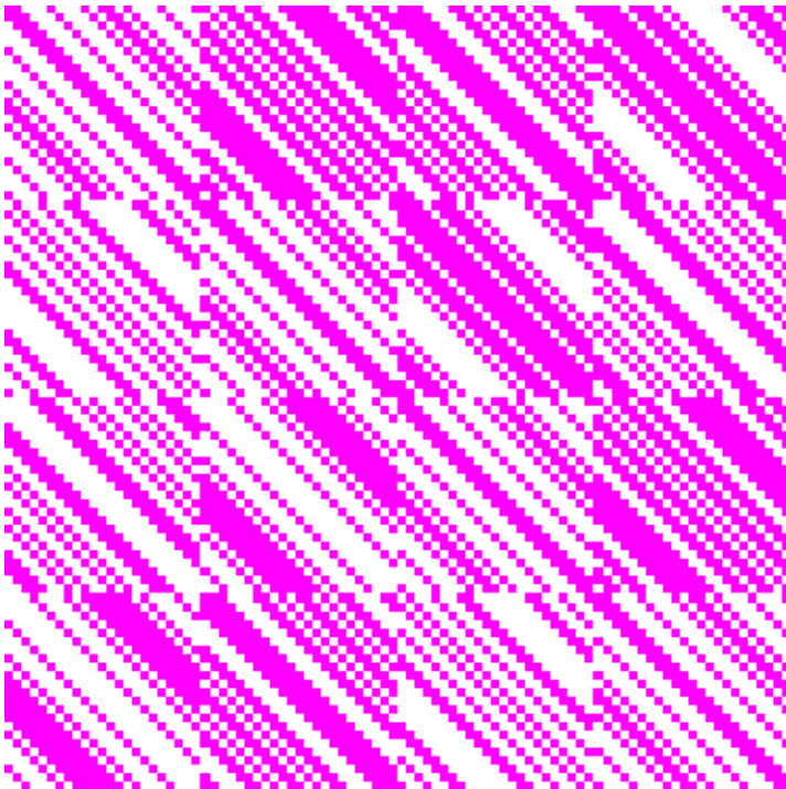
92 \times 92 Williamson construction
