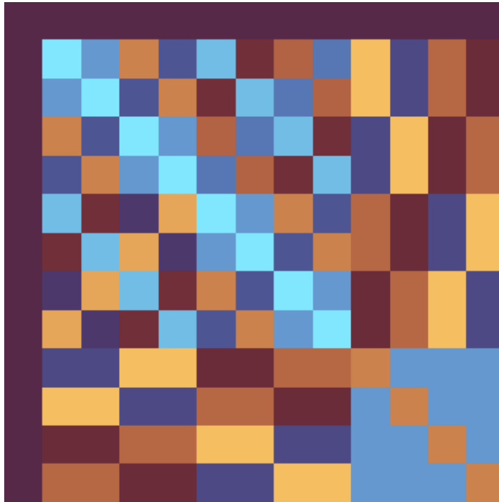
13 × 13 Petrescu Matrix
