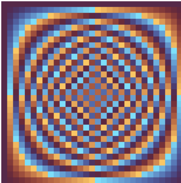
31 × 31 Fourier Matrix
