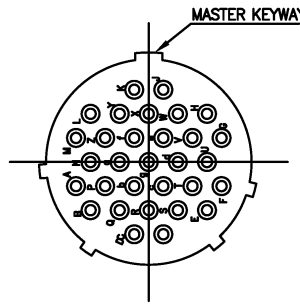
CN3 : 24-31SW (31 #16)
