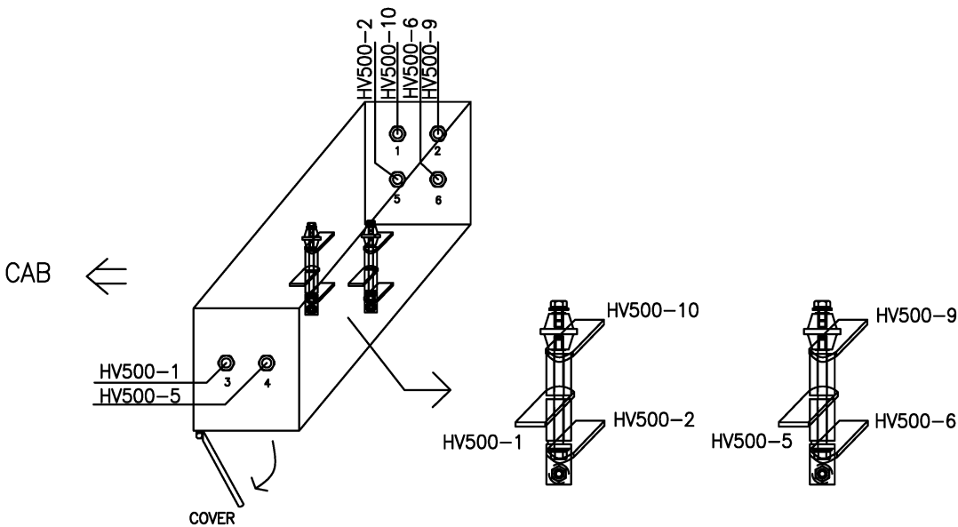
CSJB1 (FRONT)
