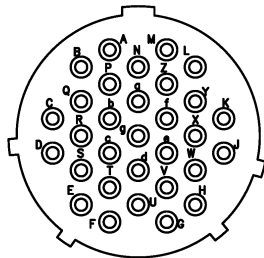
REAR VIEW OF PIN INSERT CONNECTOR : 31PIN
