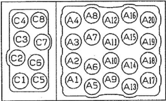
CONNECTOR PLUG : 9370100427
