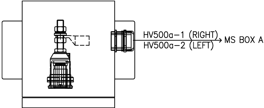
STINGER CONNECTOR WIRING
