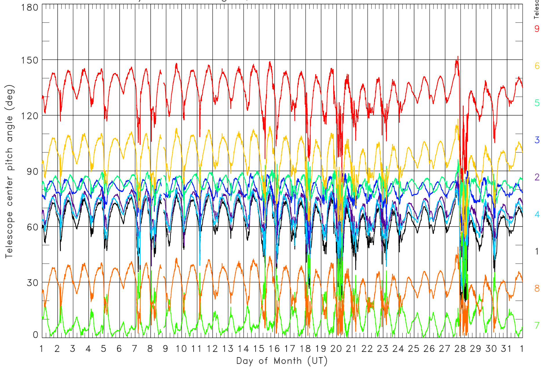
GOES-13 MAGED/PD Pitch Angles, 1m QC: 2017.05.01 00h – 2017.05.31 24h
