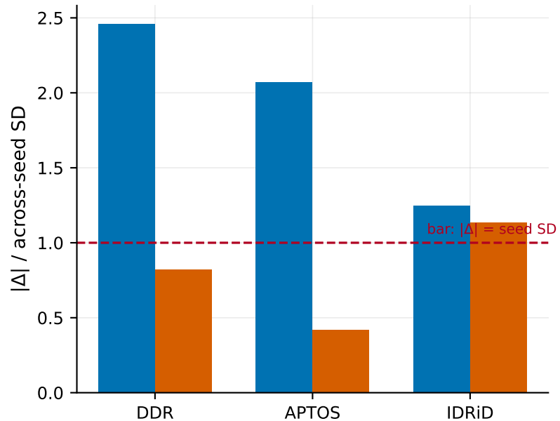
Effect against seed noise
