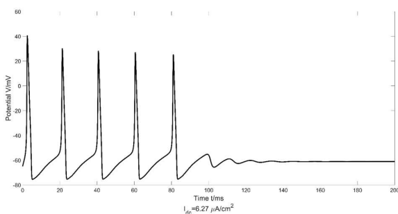
图5.7 直流刺激 6.27 \mu\text{A}/\text{cm}^2
