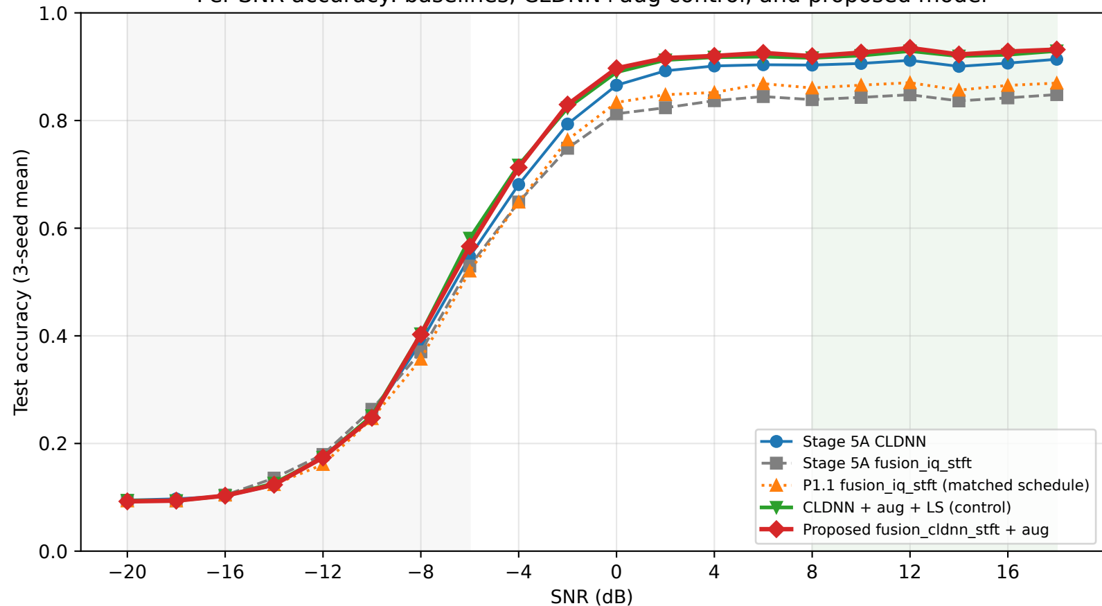
Per-SNR accuracy: baselines, CLDNN+aug control, and proposed model
