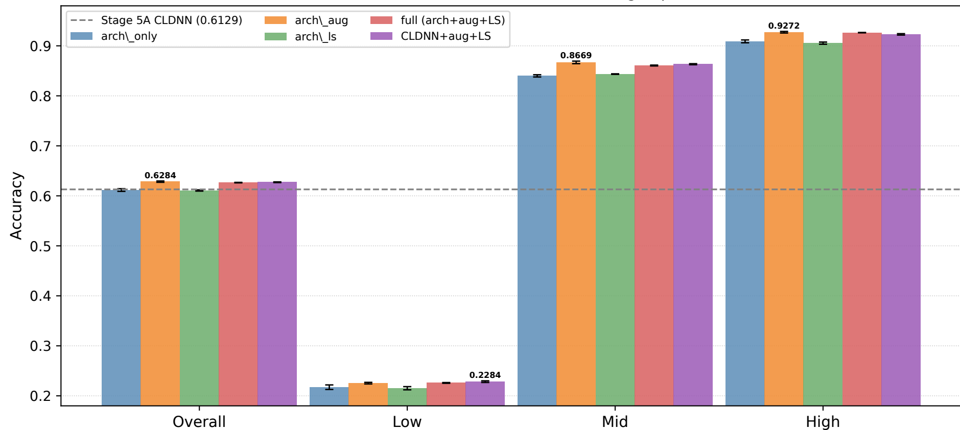
Ablation + CLDNN+aug Control: Accuracy by SNR Group (mean \pm std, 3 seeds; bold = best in group)
