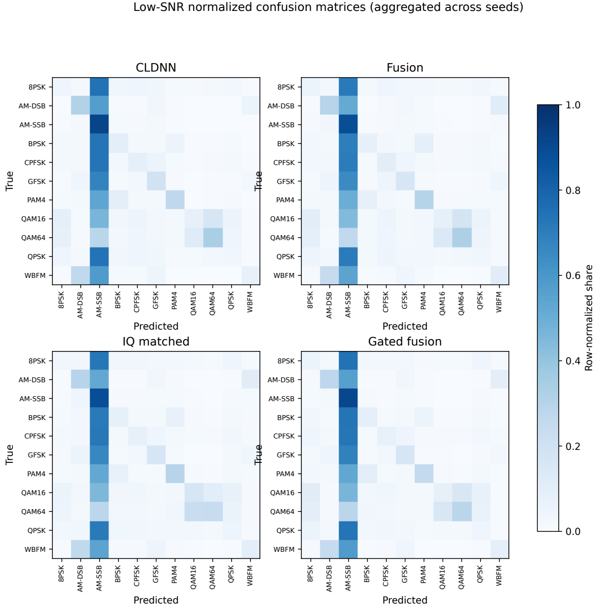
图 A.1 代表模型在 low-SNR scope 下的行归一化混淆矩阵，三训练种子聚合。Data source: confusion_low_snr.csv for seeds 42, 2025, and 3407.
