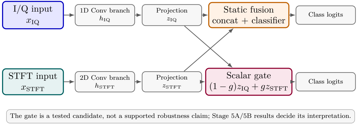
图 3.2 静态 I/Q-STFT 融合与标量门控融合的结构关系。Data source: src/radioml_amc/models/multiview.py and src/radioml_amc/models/gated_fusion.py .
