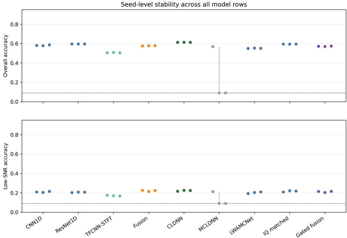
图 4.9 9 个模型行在三个训练种子上的 overall accuracy 与 low-SNR accuracy 稳定性。Data source: metrics_test.json for seeds 42, 2025, and 3407.
