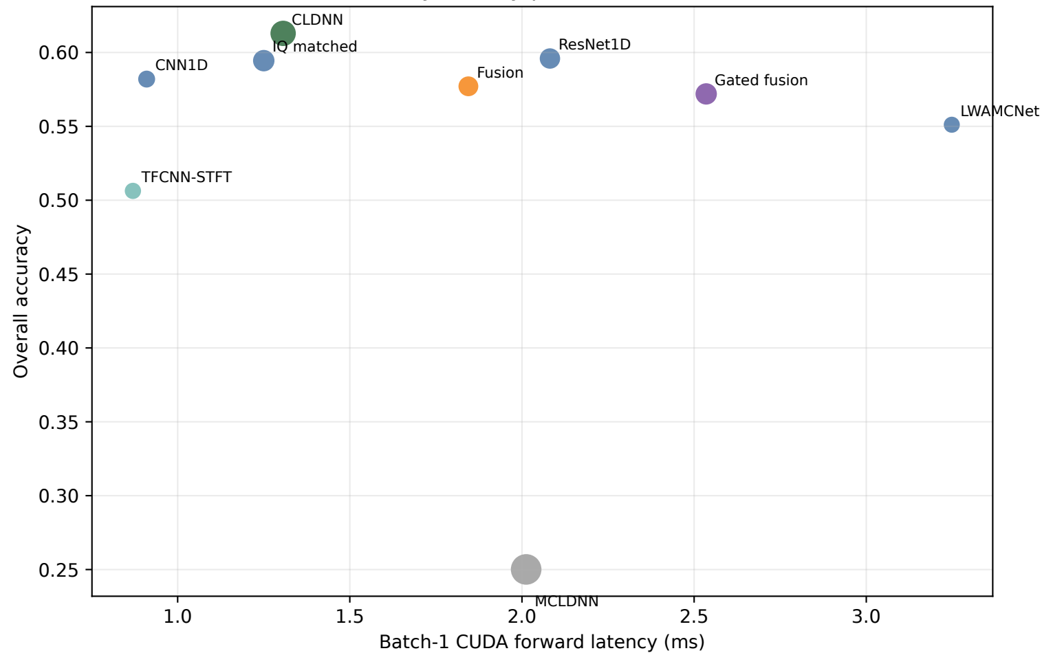
Accuracy-latency-parameter trade-off
