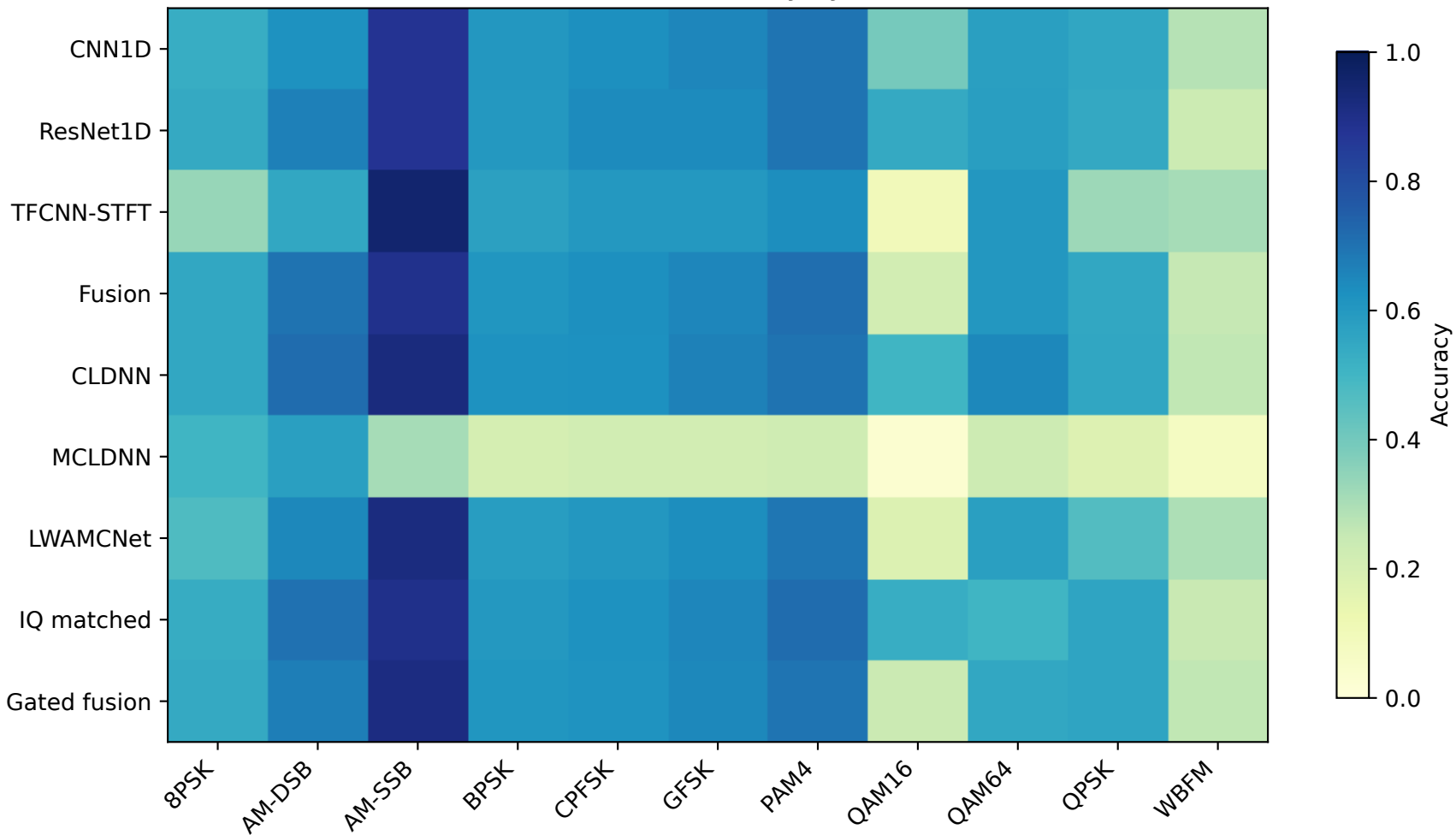
Overall class accuracy by model
