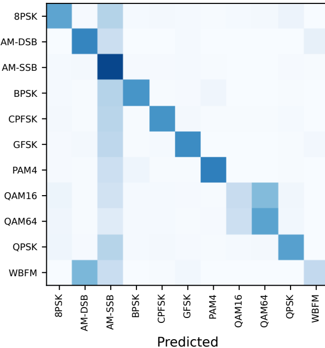
Gated fusion
