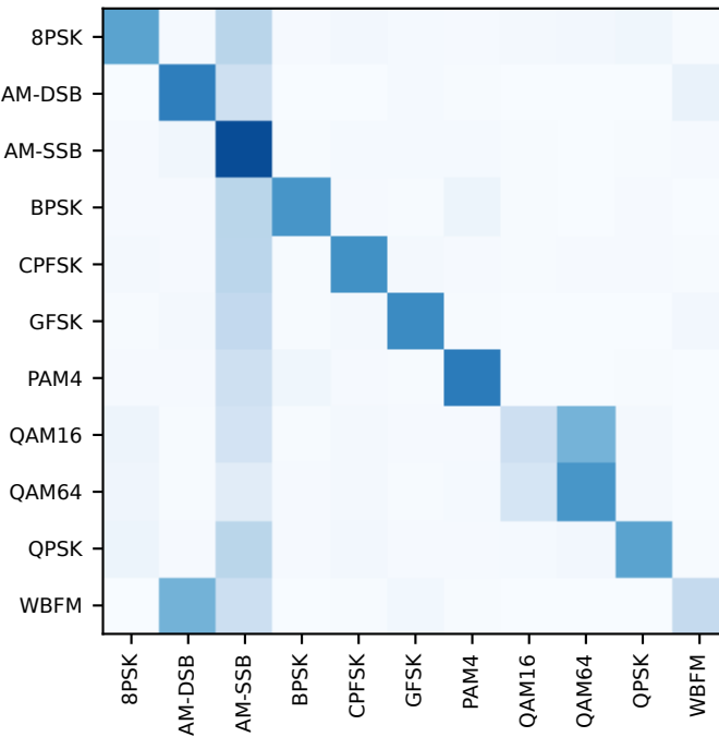
Gated fusion
