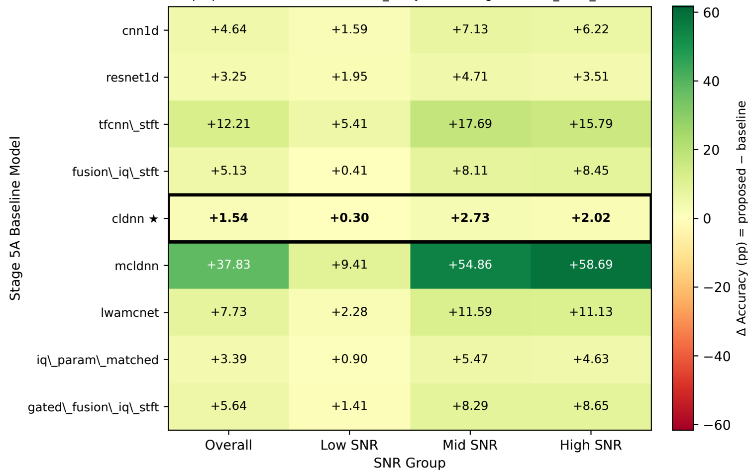
Proposed Model vs Stage 5A Baselines: \Delta Accuracy (percentage points) Data: proposed 3-seed mean (metrics_test.json) vs Stage 5A main_table_metrics.csv
