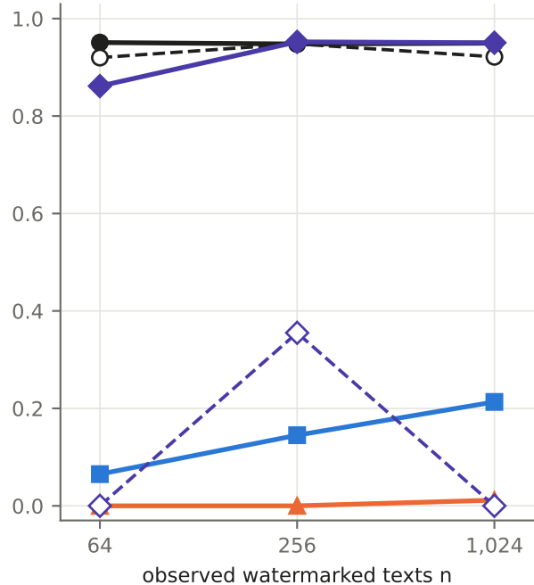
\rho = 0.50 : forgery acceptance (study keys)
