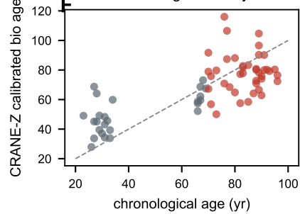
CRANE-Z bio age on array cohort
