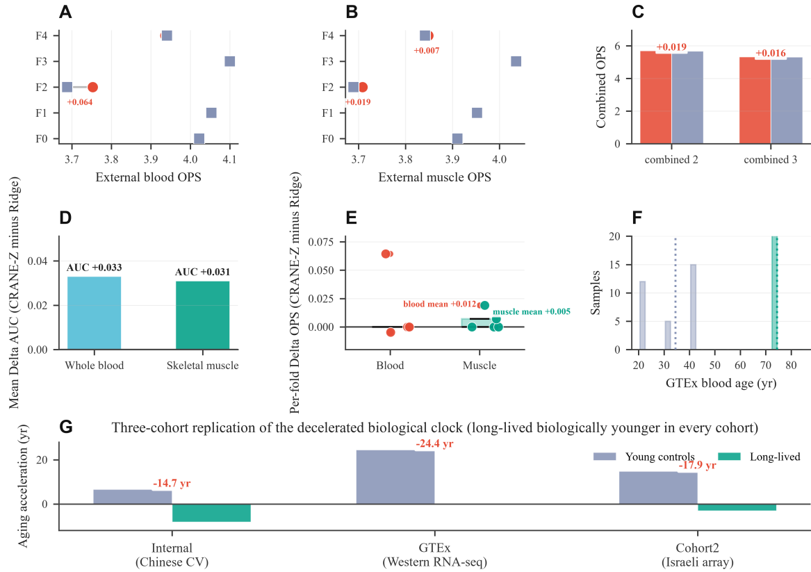
Figure 5: External validation confirming generalization across tissues and ethnicities. (A) Paired dot chart revealing the blood OPS gain on the strongest-fusion fold (filled circles: CRANE-Z, open squares: Ridge). (B) Paired dot chart displaying muscle OPS per fold (filled circles: CRANE-Z, open squares: Ridge). (C) Grouped bar chart demonstrating combined metrics above the Ridge reference (red bars: CRANE-Z, grey-blue bars: Ridge). (D) Bar chart quantifying the positive mean external AUC gain. (E) Box plot displaying the positive per-fold external OPS gain on average. (F) Histogram revealing the external age separation between the groups (blue bars: RYC, green bars: RLL).
