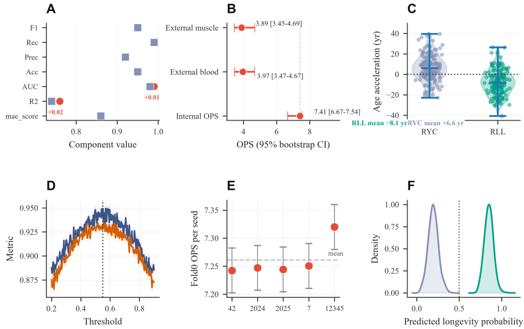
Figure 4: Component analysis showing stable and decomposable gains. (A) Dumbbell chart demonstrating CRANE-Z ahead on the age-regression components (red dots: CRANE-Z, grey-blue squares: Ridge). (B) Forest chart showing bootstrap intervals covering the internal mean. (C) Violin chart revealing aging acceleration negative in long-lived individuals. (D) Line chart illustrating threshold calibration peaking at the operating point. (E) Scatter chart displaying consistent seed stability. (F) Density chart demonstrating clean separation of the two phenotypes.
