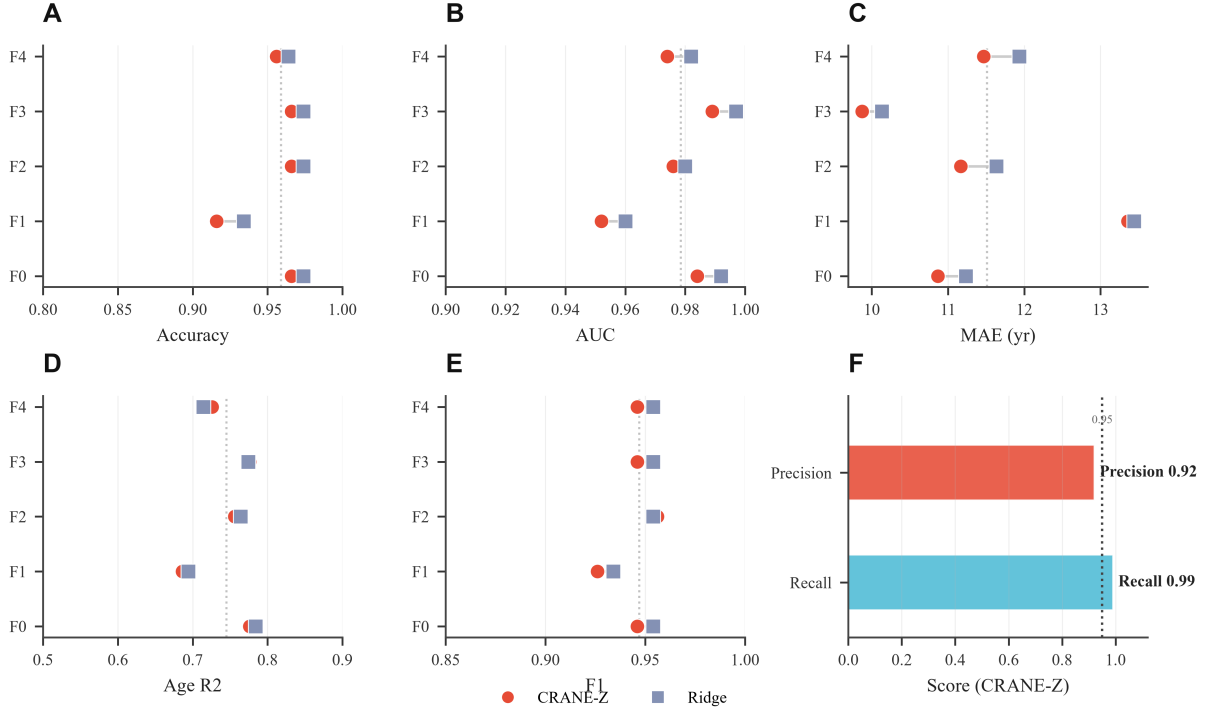
Figure 6: Per-fold detail showing component-level consistency. (A) Paired dot chart demonstrating internal accuracy per fold. (B) Paired dot chart comparing internal AUC per fold. (C) Paired dot chart revealing age MAE lower for CRANE-Z on four of five folds. (D) Paired dot chart displaying age regression R2 higher for CRANE-Z. (E) Paired dot chart illustrating F1 per fold. (F) Bar chart demonstrating precision and recall above 0.9.
