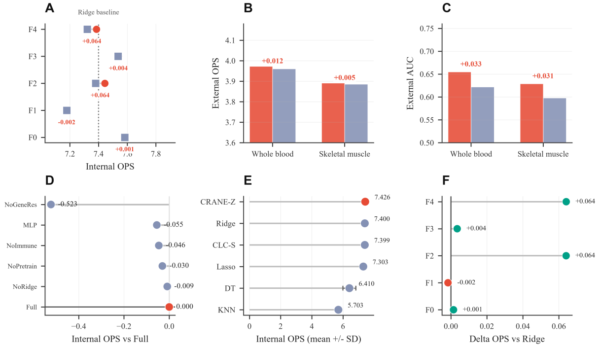
Figure 3: Main results demonstrating the age-regression advantage and the decelerated biological clock in long-lived individuals. (A) Paired dot chart demonstrating internal OPS per fold, CRANE-Z leading on four of five folds (filled circles: CRANE-Z, open squares: Ridge). (B) Grouped bar chart revealing external OPS above Ridge on both tissues (red bars: CRANE-Z, grey-blue bars: Ridge). (C) Grouped bar chart comparing external AUC, favorable to CRANE-Z on both tissues (red bars: CRANE-Z, grey-blue bars: Ridge). (D) Lollipop chart quantifying the gene-residual stream as the largest ablation cost. (E) Lollipop chart ranking CRANE-Z first among all baselines. (F) Bar chart displaying a positive per-fold OPS gain over Ridge.
