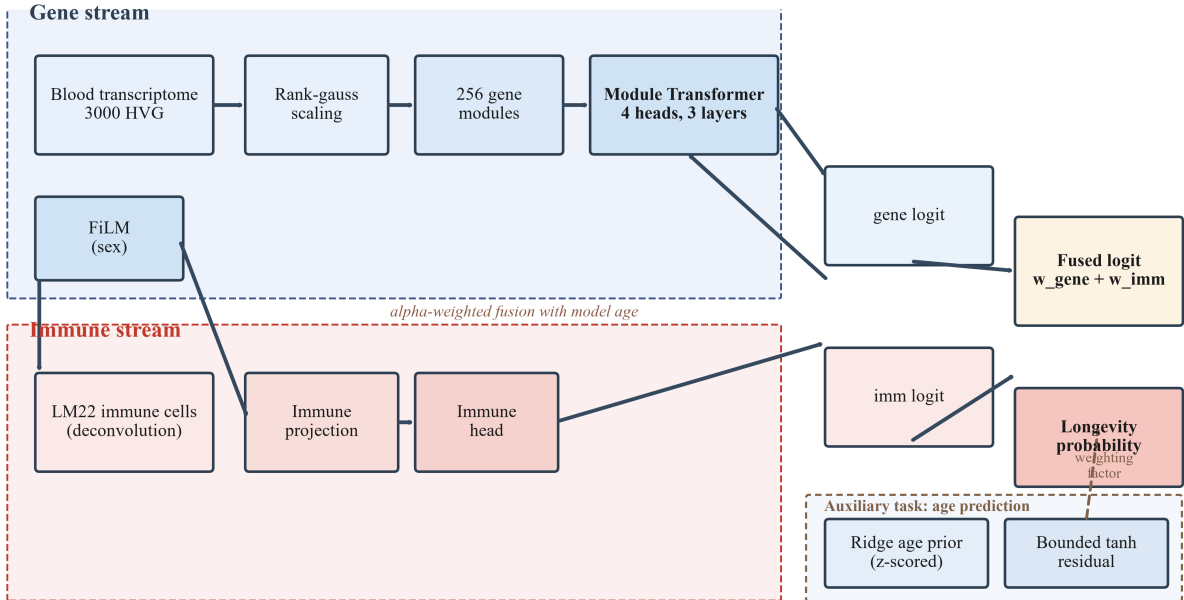
Figure 2: Model architecture of the dual-modality classifier with independent gene and immune streams. Architecture diagram demonstrating how the two modalities fuse into the longevity probability.
