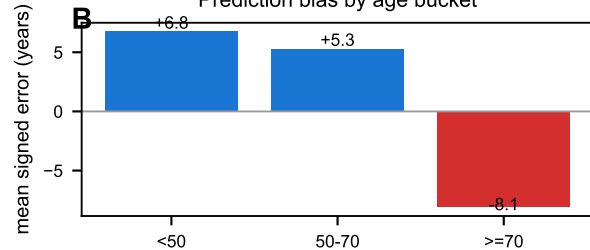
Prediction bias by age bucket
