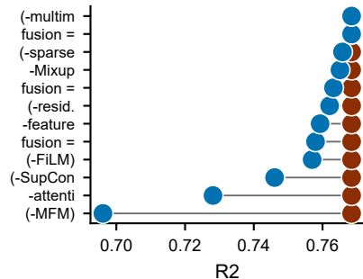
Per-variant effect (top 12)
