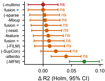
Statistical contribution (top 12)
