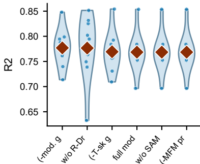
Variant performance (top 6)
