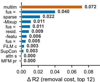
Statistical contribution (top 12)
