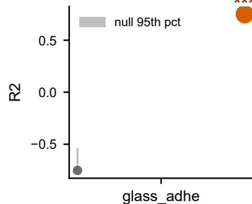
Permutation test (observed vs null 95th pct)
