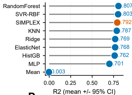
Improvement &amp; significance (forest plot)
