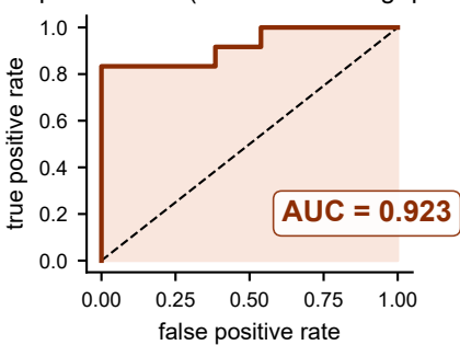
I Top-50% ROC (AUC \approx screening quality)
