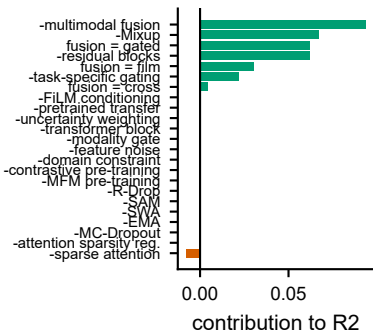
A Component contribution
