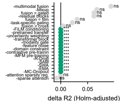
D Statistical contribution
