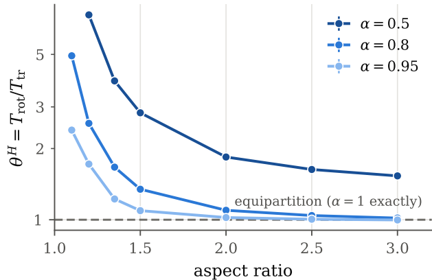
a Equipartition breaking
