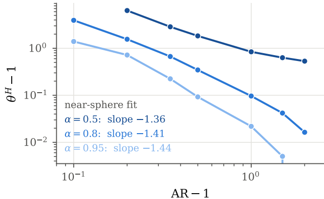
b Divergence into the smooth-sphere limit
