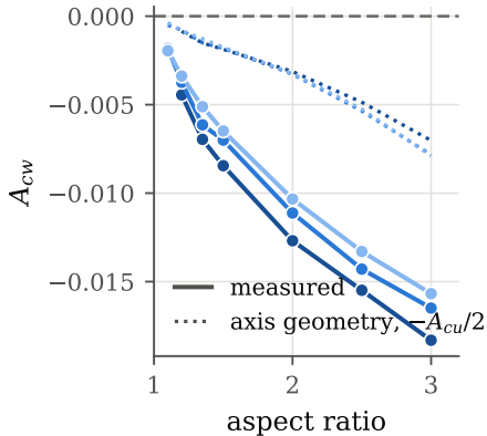
b Velocity-spin alignment
