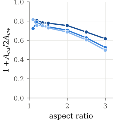
c Dynamical share of A_{cw}
