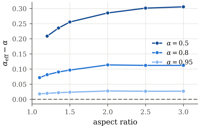
b Shielding saturates near AR \approx 2
