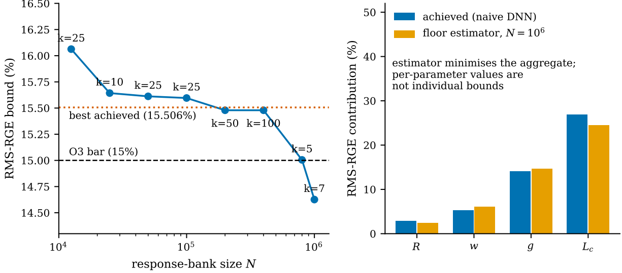
Figure 5: Left: the information bound against response-bank size, with the best neighbourhood size k annotated. The estimate is an upper bound on the true bound, and falls as the bank grows. At N = 10^6 it lies below the 15% objective threshold. Right: per-parameter error of the best model against the bound estimator’s per-parameter error; these are not individual bounds, since the estimator minimises the aggregate.
