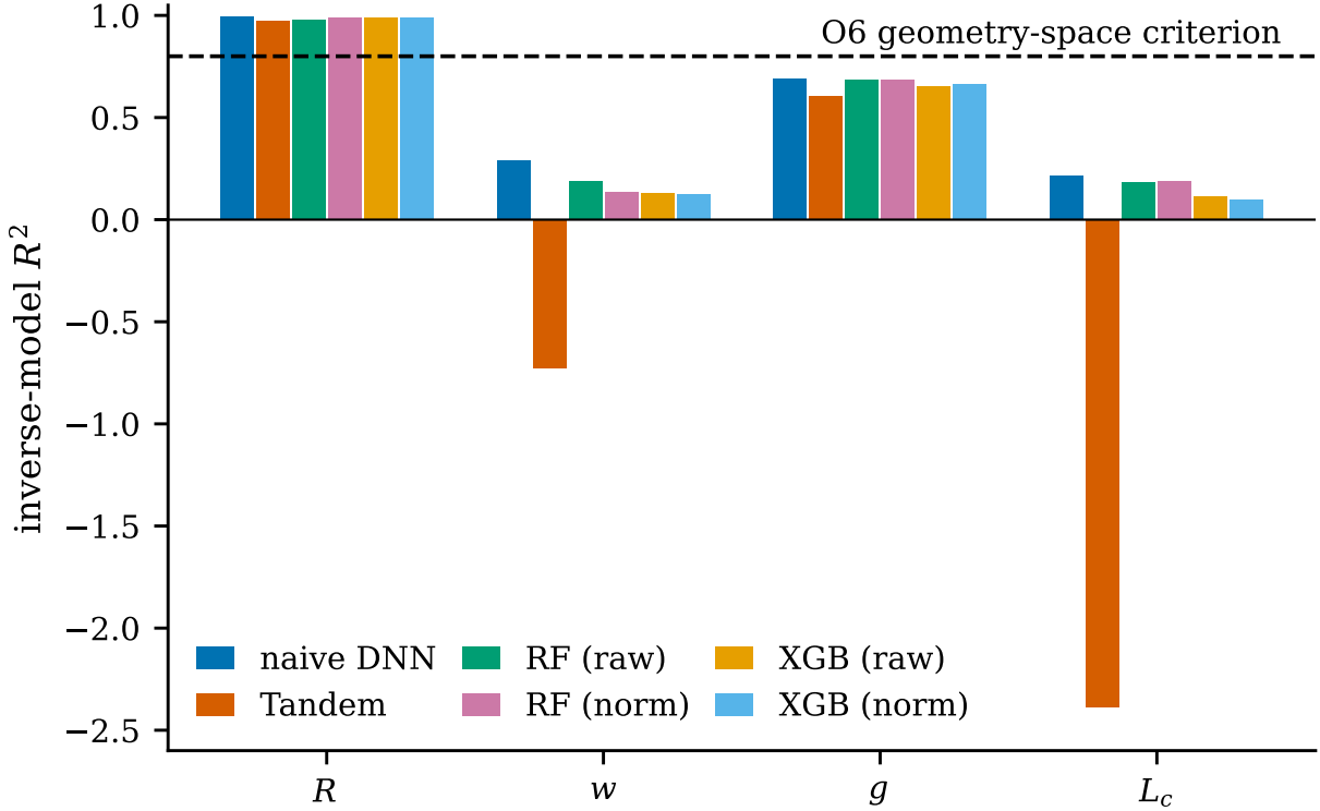
Figure 1: The geometry-space half of the one-to-many test. Only the ring radius is recovered; width, gap and coupling length are not, for every method. The dashed line is the R^2 \geq 0.80 criterion. The tandem network’s negative values for w and L_c indicate predictions worse than the test-set mean.
