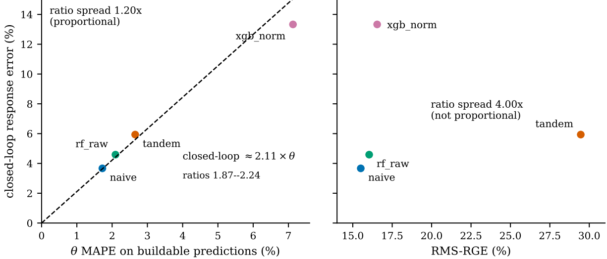
Figure 2: Closed-loop response error against two candidate metrics, for the four models whose predictions were re-simulated. Left: error in the coupling phase \theta , evaluated on buildable predictions so that the two axes cover the same designs. Right: RMS-RGE. The ratio of closed-loop error to \theta error is constant to within a factor 1.20; formed with RMS-RGE it varies by a factor 4.00.
