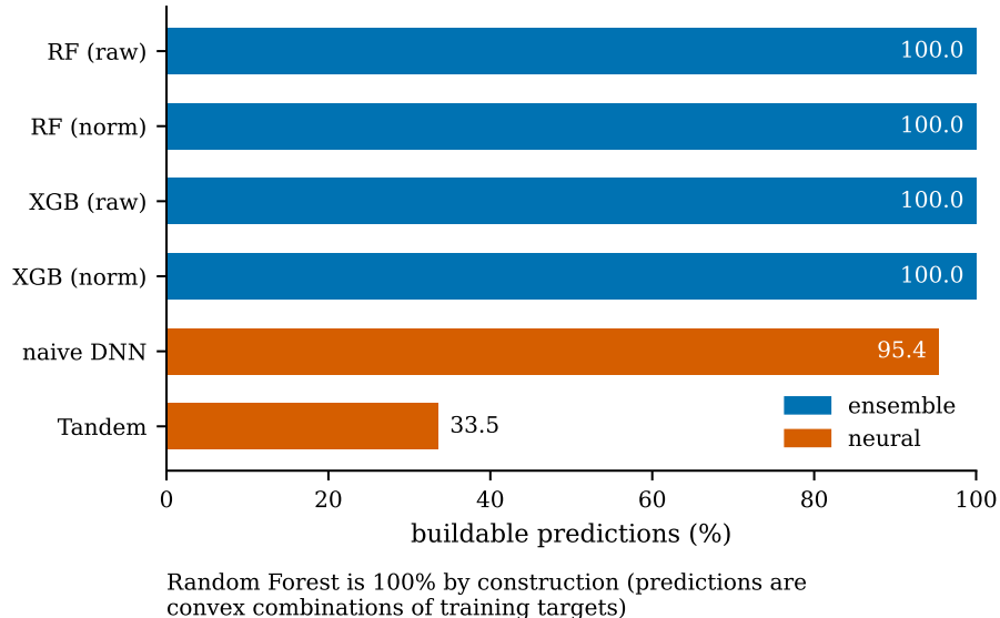
Figure 3: Fraction of test-set predictions lying inside the design box. The distinction is architectural, and invisible to both metrics of Section 3.3.
