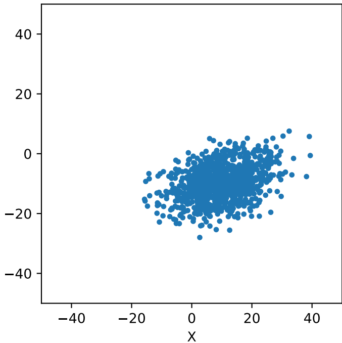
2D Gaussian distribution
