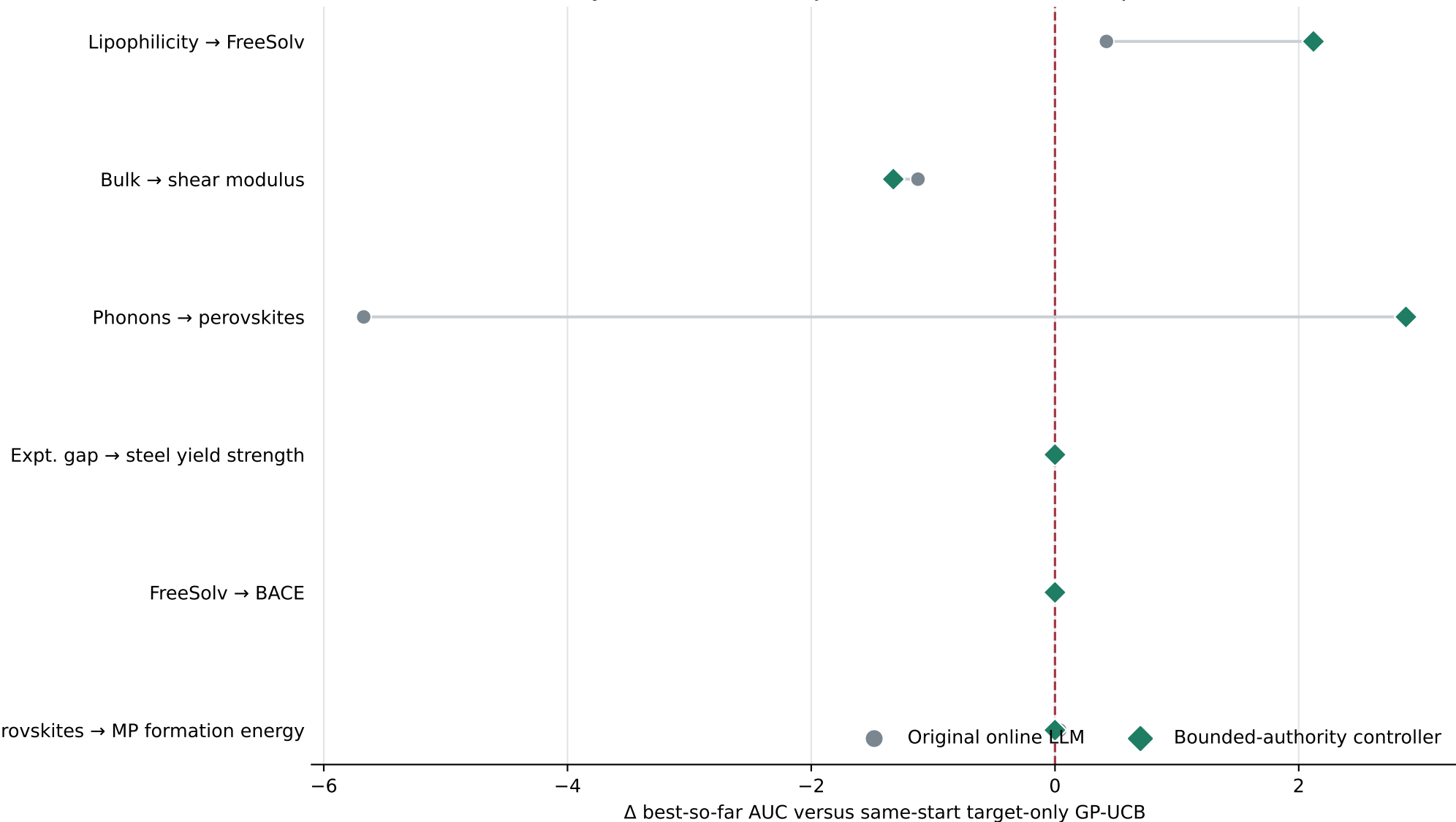
Bounded LLM authority on the route-disjoint 6-route stress-test panel
