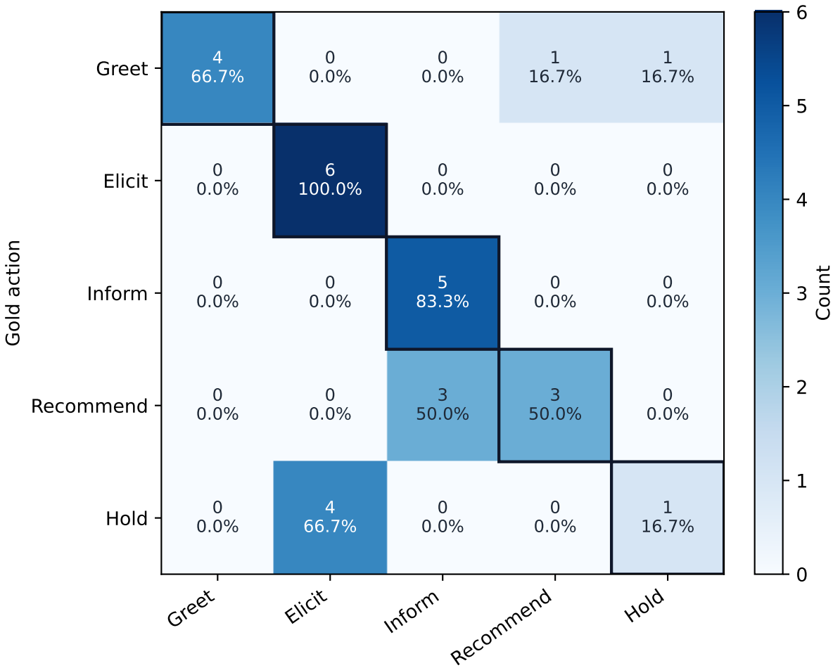
PIWM Confusion Matrix on Target-Test (n=30)
