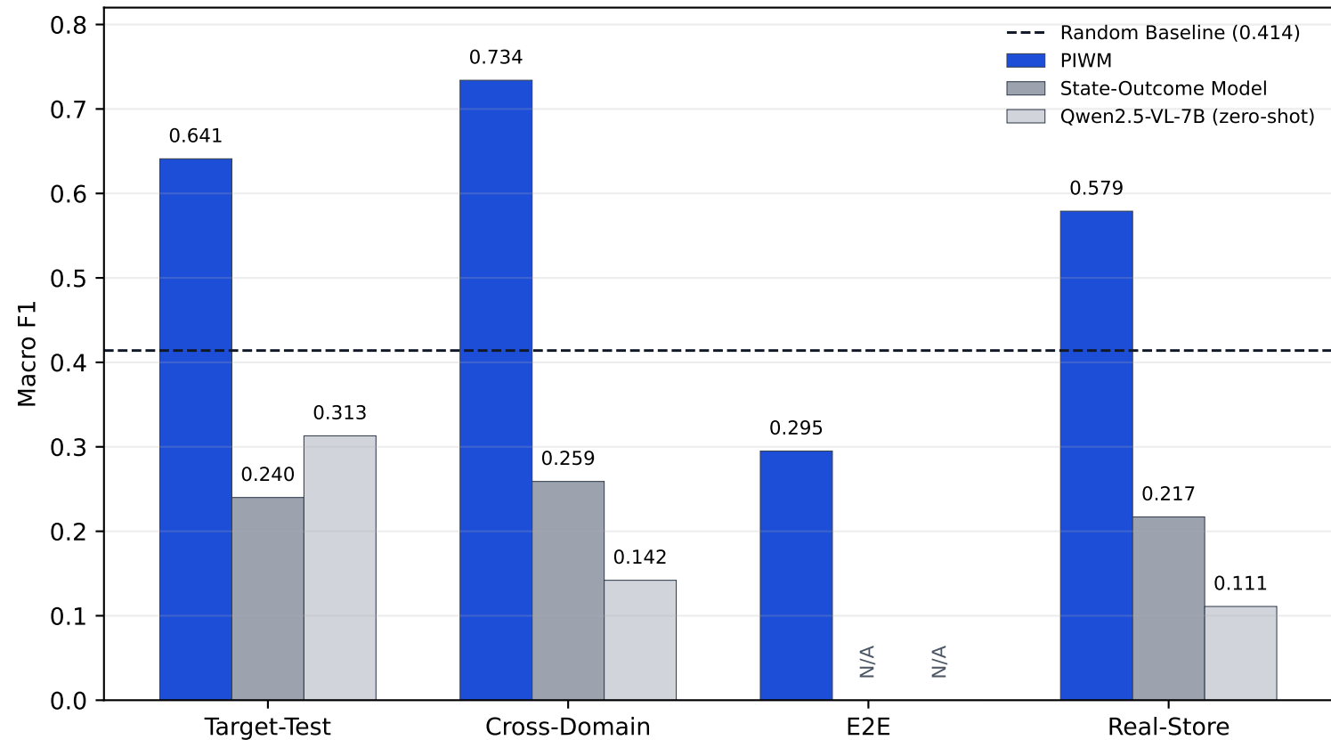
Best-Action Selection Across Evaluation Scenarios
