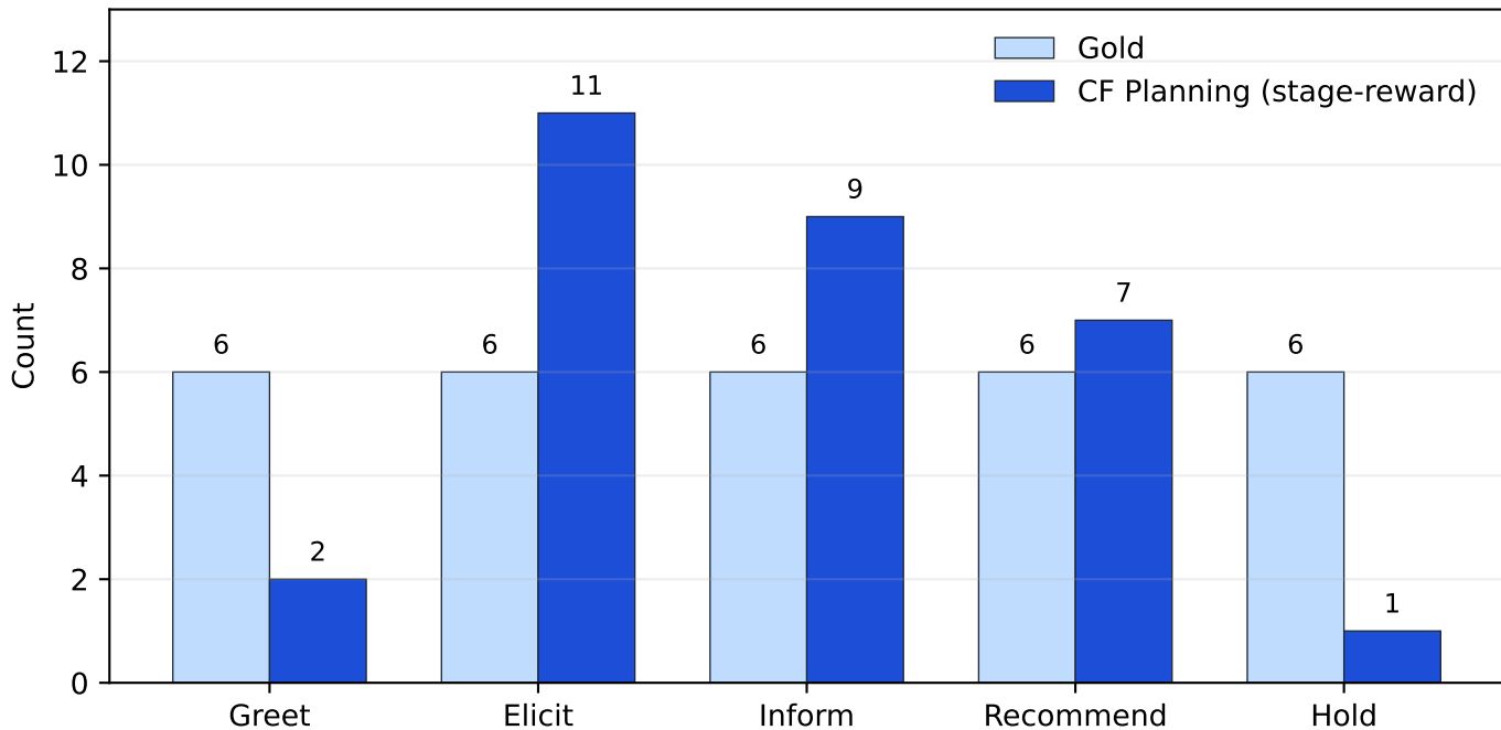
Counterfactual Planning Distribution: Predicted vs Gold
