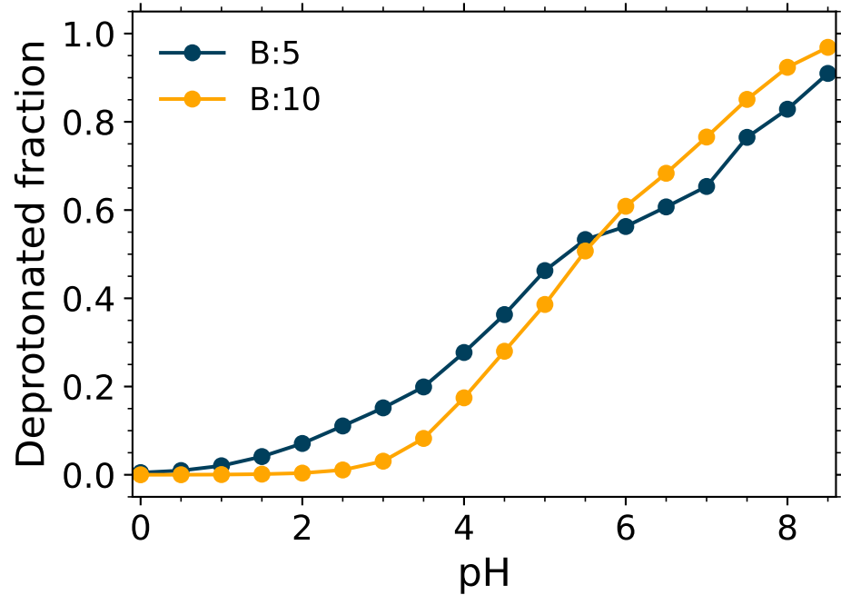
(B) Histidine
