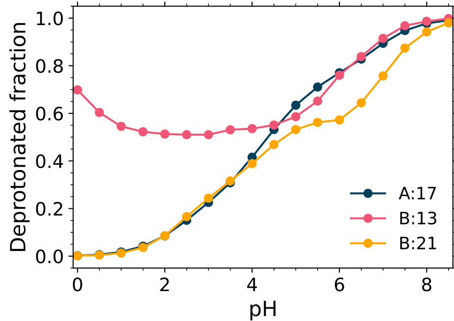
(A) Glutamate
