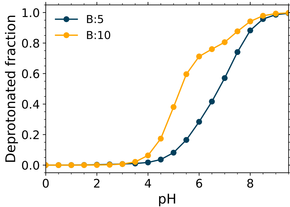
(B) Histidine
