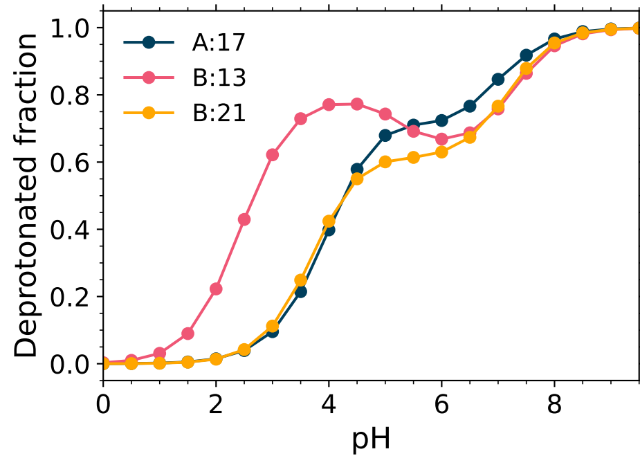
(A) Glutamate
